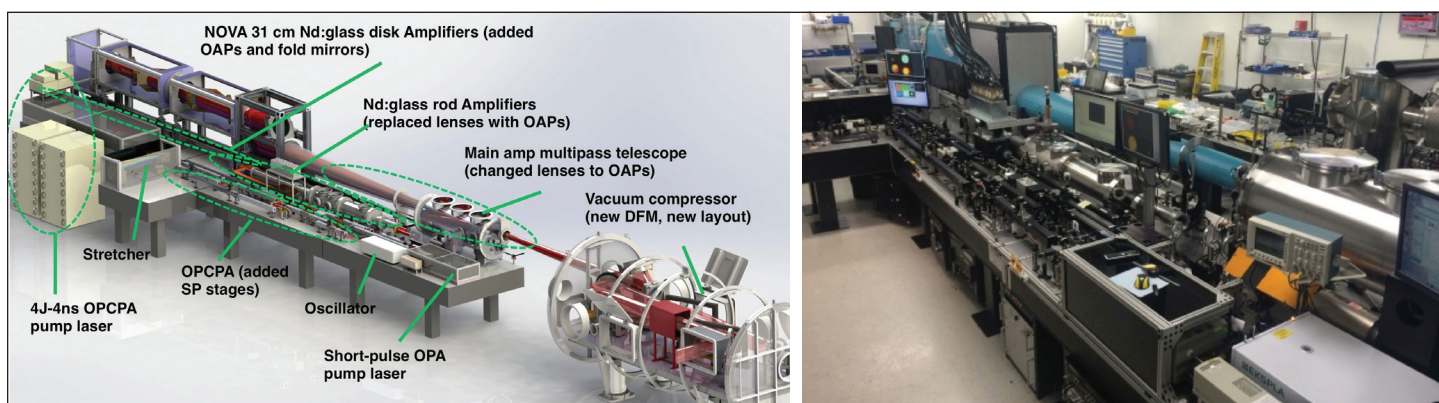
Figure 2. A graphical summary of the improvements made to the TPW laser (left) and a photo of the upgraded laser chain (right).
