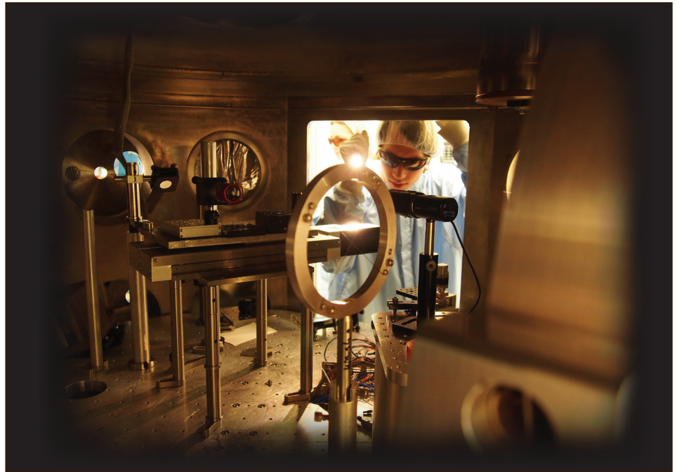
The Texas Petawatt Laser high intensity target chamber from behind the final mirror.
