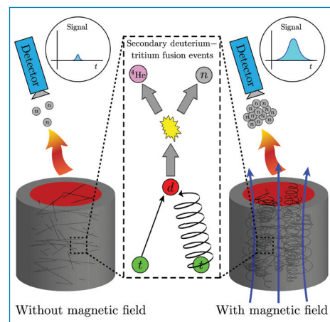
Figure 1. Graphic depicting the impact of extreme magnetic fields on secondary fusion reactions in MagLIF. Center: Illustration of “secondary” fusion events in pure deuterium fuel, where fast tritium nuclei produced by fusing deuterium react with additional deuterium nuclei, producing a high-energy neutron. Bottom left: schematic of a burning cylinder of fusion fuel without a magnetic field, with the black tracks indicating fast tritium trajectories. Tritium escapes along straight lines, producing few secondary neutrons. Bottom right: schematic of tritium trajectories in the presence of strong magnetic fields inferred on the first MagLIF experiments. Effective tritium confinement manifests in neutron detectors (top right and left) as a 100-fold stronger secondary signal than what would have been anticipated in the absence of the extreme magnetic fields.
