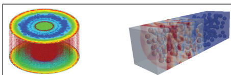
Figure 1. (Left) Multiphase three-dimensional simulations of cylindrical blast wave. (Right) Mesoscale simulations of shock propagating through a random pack of particles.
