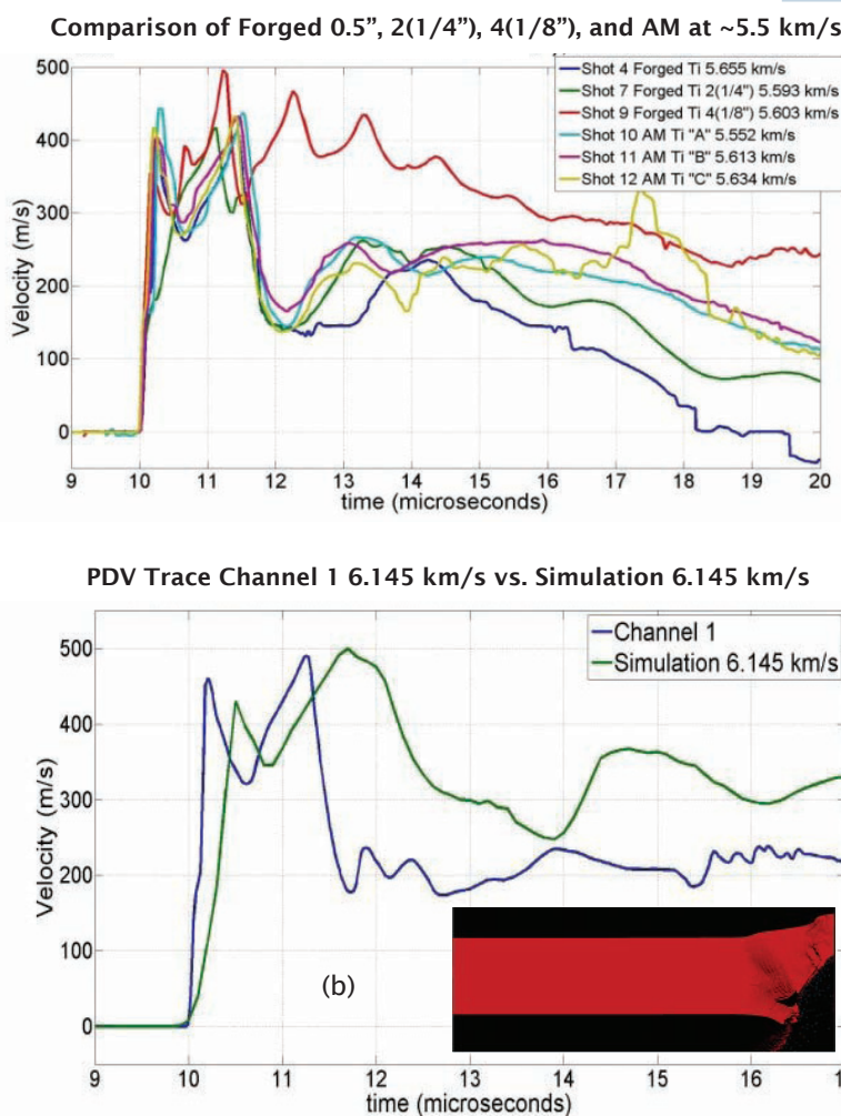
Figure 2. Velocity traces of (a) Experimental forged, layered, and AM Titanium and (b) AM titanium experimental and computer code (LS-DYNA) simulation. In (a), 2(1/4) indicates two stacked 1/4"-thick plates. 4(1/8) indicates four stacked 1/8"-thick plates. In (b), the picture shows the symmetric cross section of an impacted plate.
