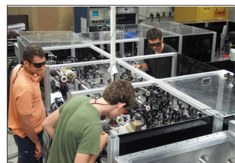
Figure 3. CHEDS students working on the GHOST 20 TW table top laser in preparation for solid target experiments.
