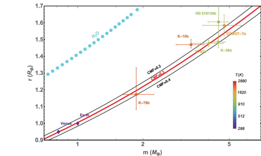
Figure 1. Radius versus mass plot for Venus, Earth and exoplanets with up to five Earth masses, given in units of Earth radii and Earth masses ( \oplus = Earth). The color of the symbols for each planet indicates their surface temperatures (see scale in kelvins). The blue dotted curve is for planets made of pure H 2 O. The solid red curve is for planets with the same bulk chemical composition as the Earth (including the CMF as the Earth of 0.3). For comparison curves for CMF values of 0.2 and 0.4 are also shown. Previous work suggested a core mass fraction of about 0.17 for the exoplanets, and their bulk chemistry would then be different from the Earth. Our new equation of state estimate for real Earth chemistry shows, however, that the exoplanets are consistent (within error) of an Earth-like chemical composition.
