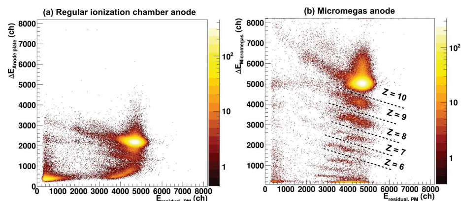
Figure 1. A comparison of measured particle energy loss ( \Delta E ) in an ionization chamber versus the measured residual energy ( E ) in plastic scintillator in cases where the ionization chamber was (a) regular ionization chamber anode plate, and (b) the newly developed Micromegas anode plate. The measured energies are given in digitized values (ch) and the color scale shows the intensity of the particles. Both data were collected by bombarding a ^{13}\text{C} foil with a 12-MeV/nucleon ^{22}\text{Ne} beam at the same scattering angle. The enhanced isotopic resolution of the new detector is evident as the different elements (labeled with their proton number, Z ) are clearly separated from the main beam (Neon, Z = 10 ). This allows for a much enhanced particle identification, which produces improved energy resolution and a reduction of background.
