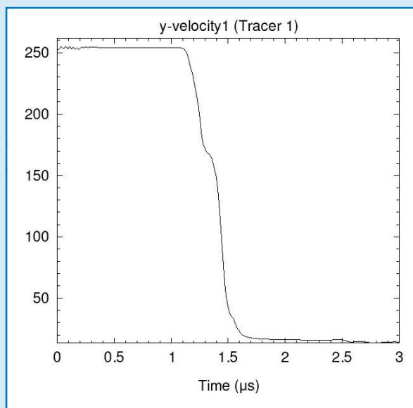
Figure 1. Hydrocode simulation of the shock velocity in the aluminum target due to a symmetric impact of 0.5 km/s.
