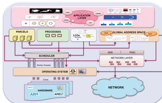
Figure 2: HPX runtime system (version 1.3.0), which reifies the ParallelX execution model.
