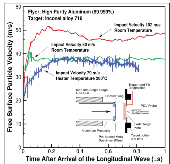
Figure 2. Free-surface particle velocity vs time profiles obtained from normal shock-compression plate impact experiments on high purity polycrystalline aluminum.
