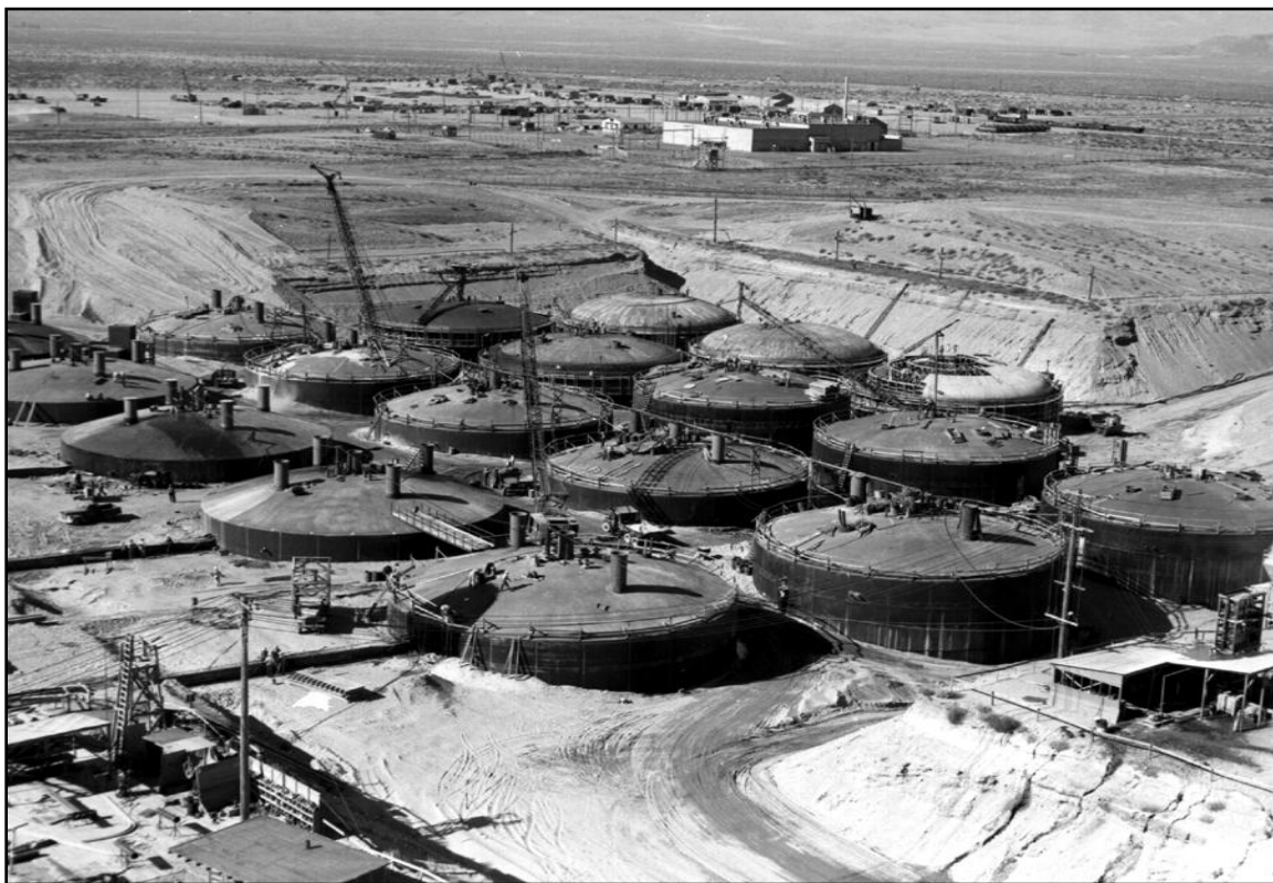
Figure S-2. Single-Shell Tanks Under Construction at the Hanford Site, 1947 to 1948
