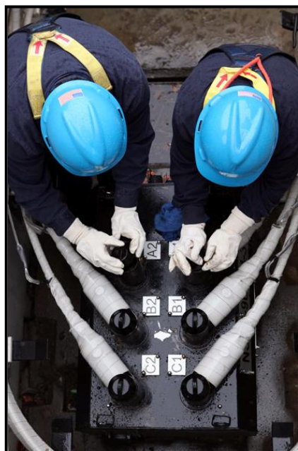
The smart switch is a main component of Con Edison’s intelligent underground system.
