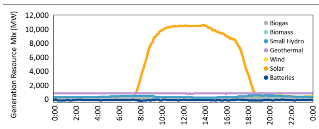
Figure 2-30. The generation mix (MW) on March 18, 2019 in CAISO. (Data source: CAISO)
