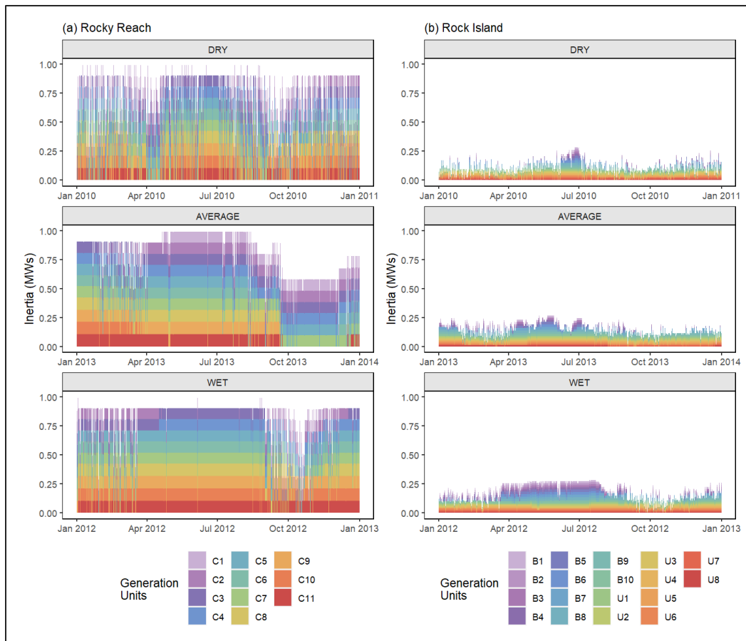
Figure 2-16. Hourly average inertia (MWs) contributed by all generating units for (a) Rocky Reach and (b) Rock Island run-of-river projects across dry, average, and wet years. Inertia response capabilities depend on water availability throughout the year, and the most generation during summer of wet years.
