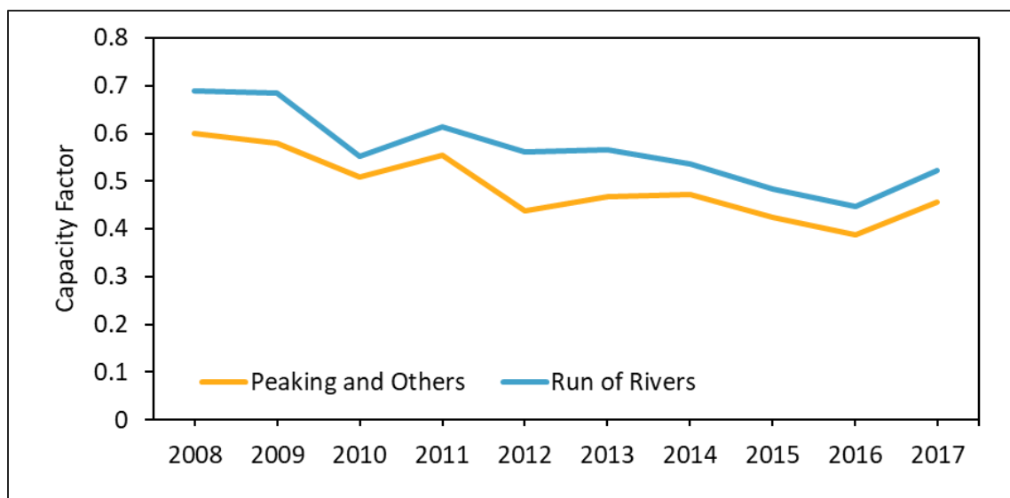
Figure 2-11. Capacity factors of conventional hydro resources in ISO-NE. (Data source: FERC Electric Quarterly Report [EQR])
