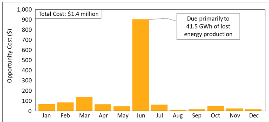
Figure 2-28. Opportunity costs associated with carrying operating and contingency reserves at LAP hydropower resources in the Western Area Power Administration, Colorado-Missouri Region balancing authority area of the Rocky Mountain Transmission Group joint-tariff market, for simulation year 2024.
