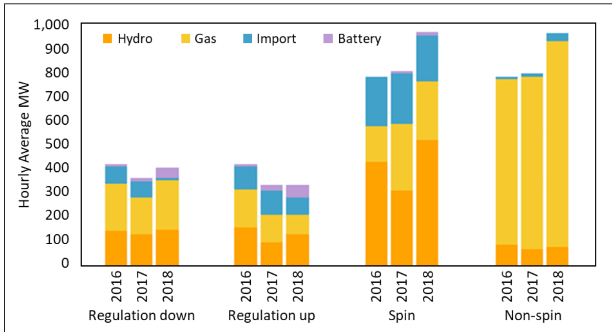
Figure 2-15. Contribution of hydropower resources for essential reliability services in CAISO. 20 Hydropower’s total capacity ranges from 10–15% of total capacity in CAISO. (Data source: CAISO)
