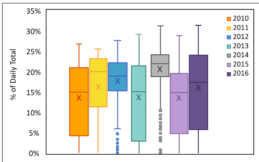
Figure 2-14. Percentage of spinning reserve provided by conventional hydropower resources in MISO. Hydropower’s total capacity ranges from 3–5% of total the installed generation capacity. (Data source: MISO)
