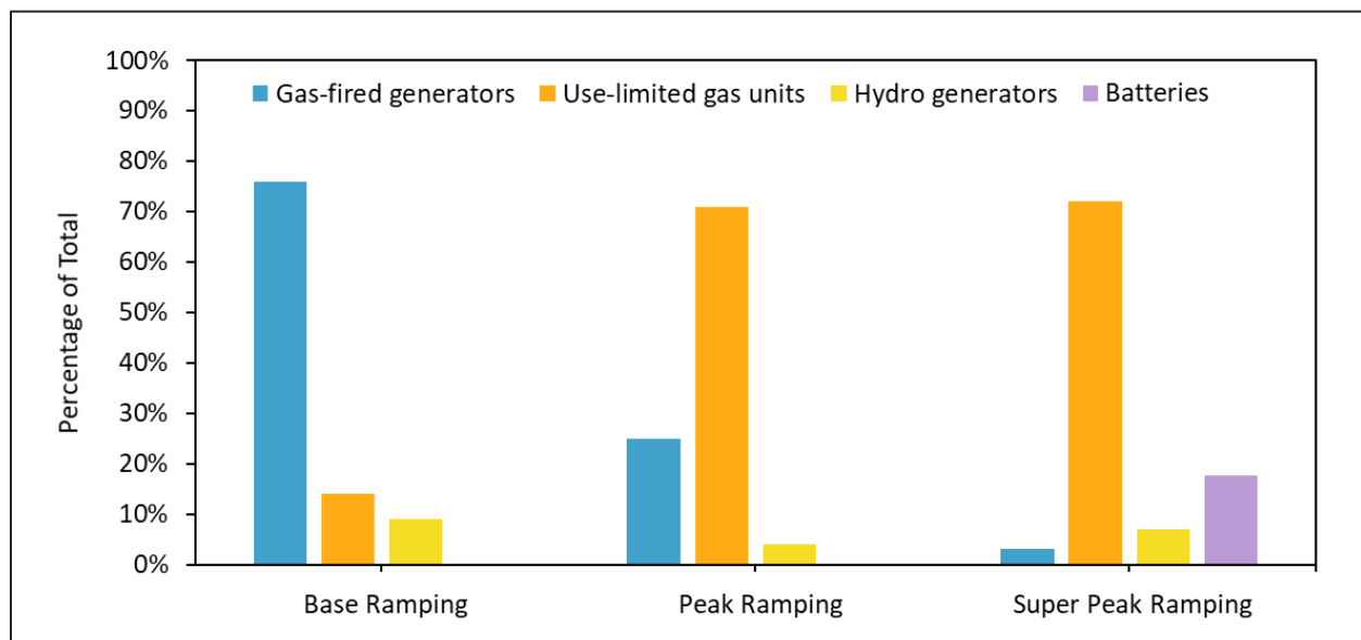
Figure 2-31. FRA capacity provided by different resources in CAISO. (Data source: CAISO)
