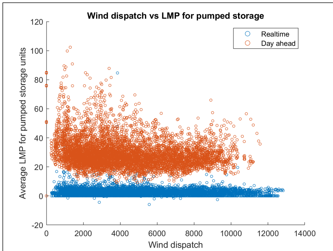
Figure 2-6. Wind generation does not affect LMPs at the PSH locations in MISO. (Data source: MISO)
