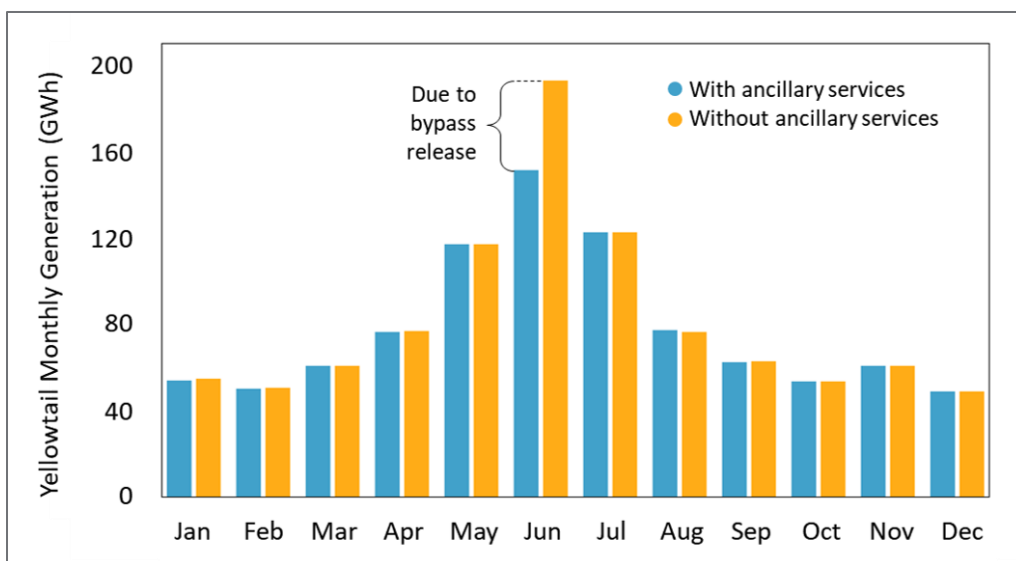
Figure 2-29. Monthly projected generation for Yellowtail hydropower facility during a sample year.
