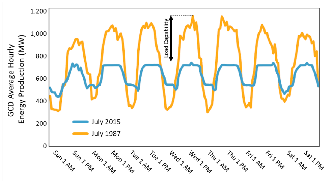
Figure 2-17. Hourly energy production at the GCD powerplant during a July week in 1987 and 2015. Flexibility was restrained with the implementation of new environmental restrictions.
