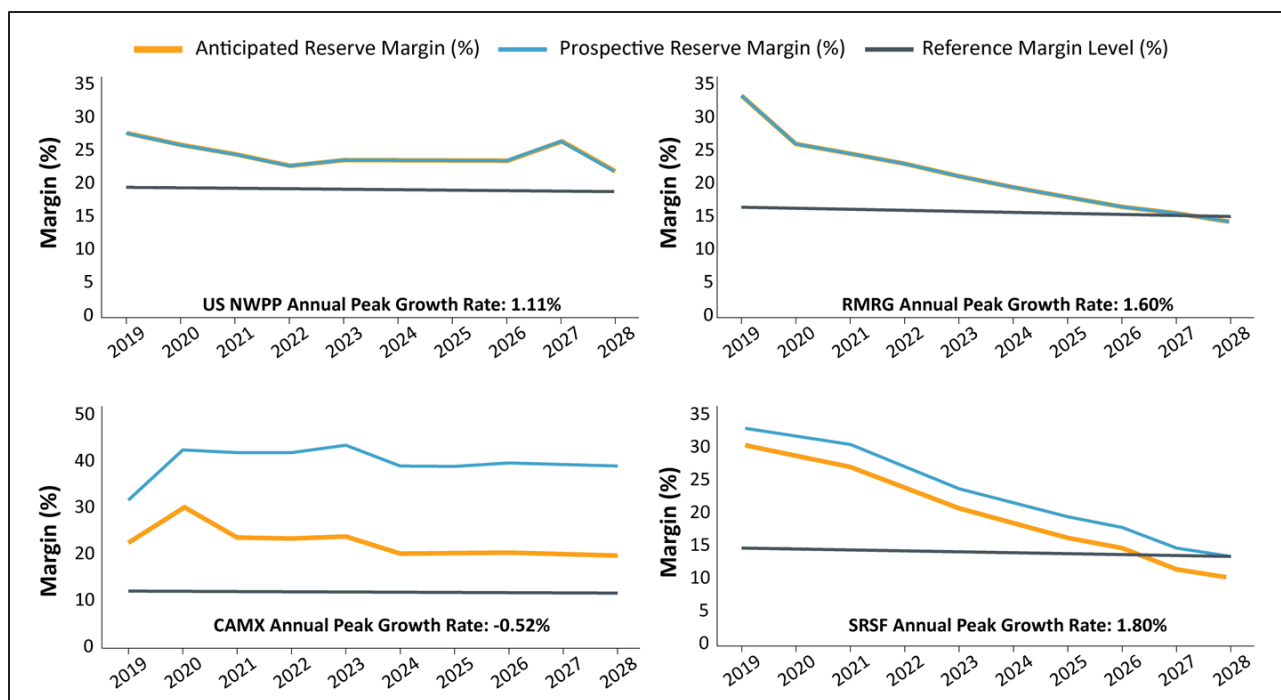
Figure 2-13. Capacity RMs between 2019 and 2028 in the four NERC subregions.
