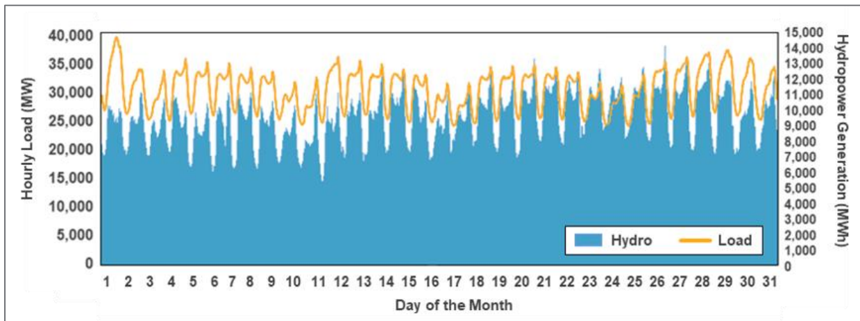
Figure 2-9. Typical pattern of hydropower operations in the Pacific Northwest compared to gross load in March 2016. Hydropower is continuing to operate in gross load-following patterns as designed. (Data source: EIA)
