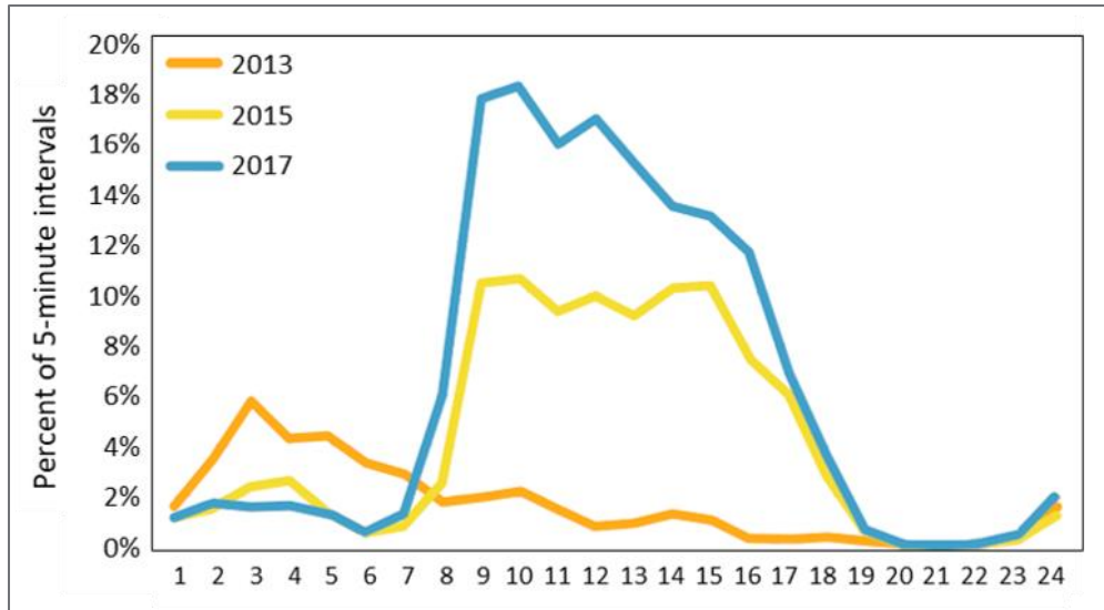
Figure 2-2. Percentage of negative price 5-minute intervals in 2013, 2015, and 2017 in the CAISO during the hours of a day. (Data source: CAISO)
