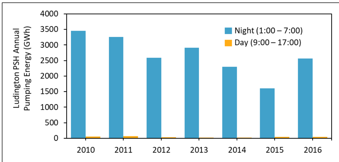
Figure 2-3. Pumping operations of PSH plants in MISO over the years. (Data source: MISO)
