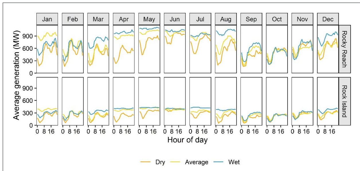
Figure 2-18. Comparison of average hourly generation during dry, average, and wet years at Rocky Reach and Rock Island Dams. During spring and early summer months of wet years at both Rocky Reach and Rock Island, the flexibility of operations is restricted due to high flow conditions. (Data source: Chelan PUD)
