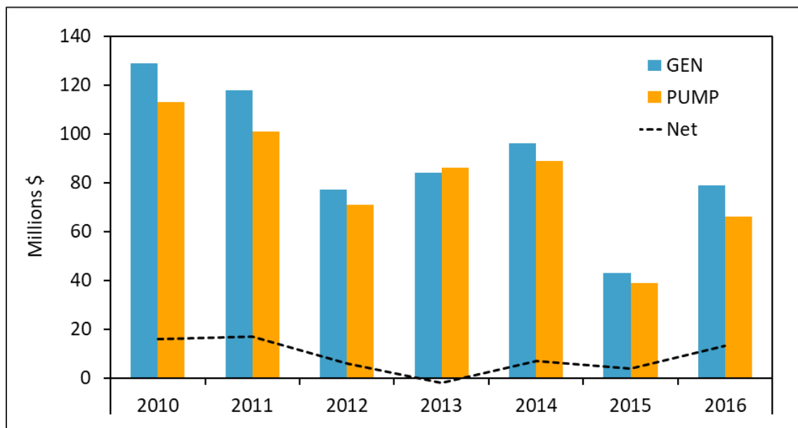
Figure 2-25. Comparison of annual revenue and pumping costs for PSH units in MISO. Net revenue has decreased since 2010 but increased slightly in 2016. (Data source: MISO)
