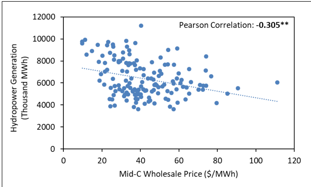
Figure 2-21. Hydropower generation is negatively correlated with Mid-C wholesale price. (Data source: EIA)
