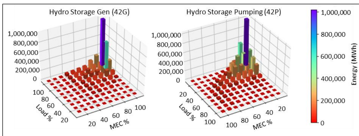
Figure 2-8. Comparison of PSH operations in pumping vs. generation modes in MISO (2015–2017). Marginal Energy Charge (MEC) is the energy component of the LMP. (Data source: MISO)
