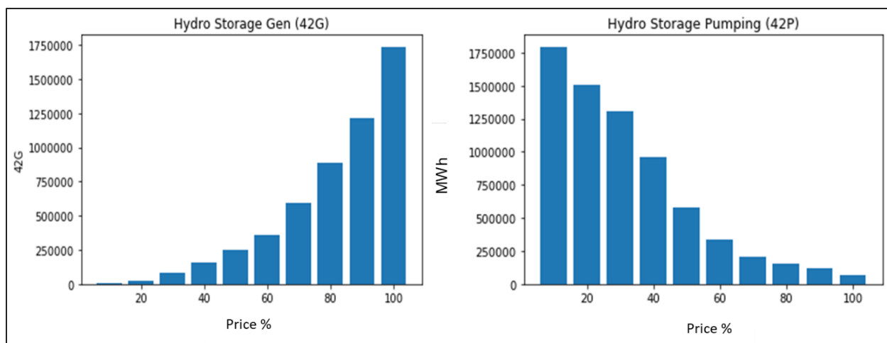
Figure 2-7. PSH generation and pumping relative to system prices (LMPs). (Data source: MISO)
