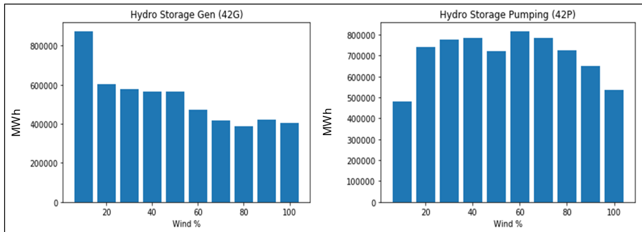
Figure 2-5. PSH generation and pumping relative to wind generation. (Data source: MISO)
