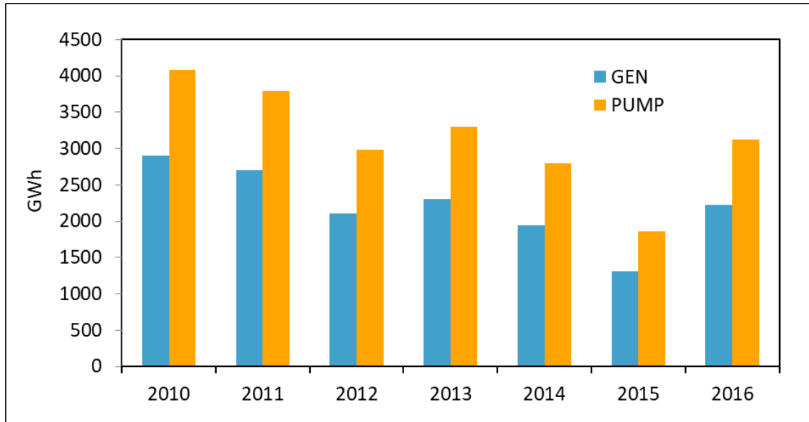
Figure 2-23. Annual generation vs. pumping load for PSH resources in MISO. Total generation and pumping have decreased since 2010. (Data source: MISO)
