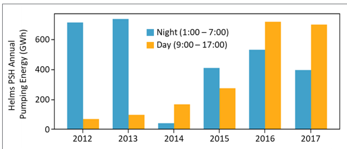
Figure 2-4. The changes in annual pumping schedules of the Helms PSH plant in CAISO. (Data source: PG&E)
