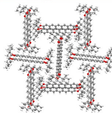
Photograph and crystal structure of candidate molecular system for entangled qubit generation through light absorption and singlet fission.
