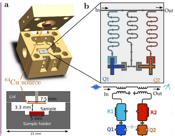
Illustration of the sample holder and the ^{64}\text{Cu} radiation source. The copper radiation source is mounted 3.3 mm above the silicon chip containing the superconducting aluminum transmon qubits. b) False-color micrograph and circuit schematic of the qubit sample.
