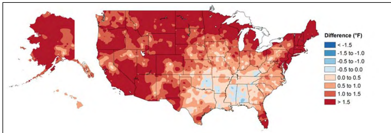
Figure 3.10-9. Observed U.S. Temperature Change, 1986 to 2015, Relative to 1901 to 1960
