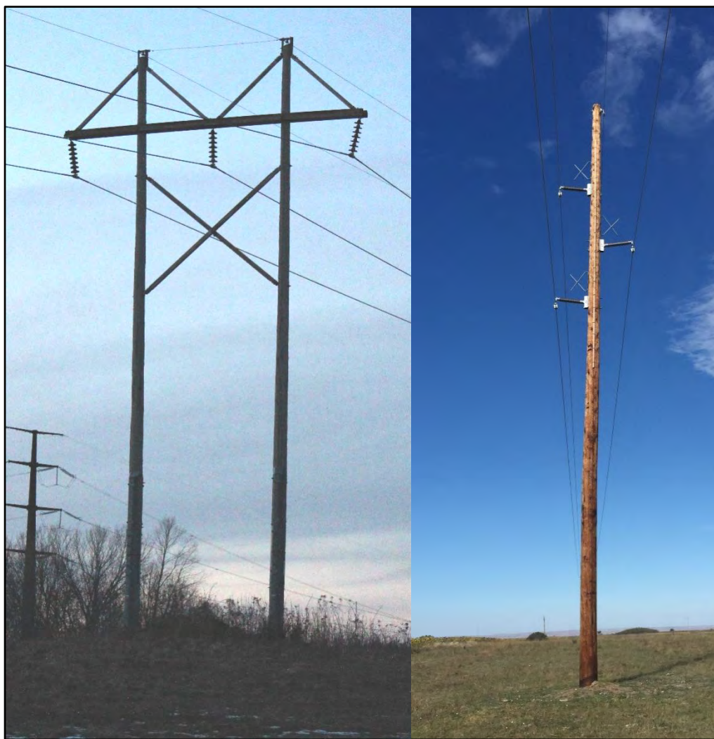
Figure 6-4. Examples of 115-kV H-frame Transmission Structures (left) and Monopoles (right)
