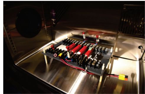
The Impedance Measurement Box can effectively look at a single battery cell or battery strings commonly used in many consumer applications.
