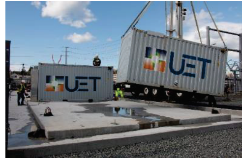
Snohomish PUD's flow battery system housed in shipping containers. Batteries manufactured by UniEnergy Technologies.
