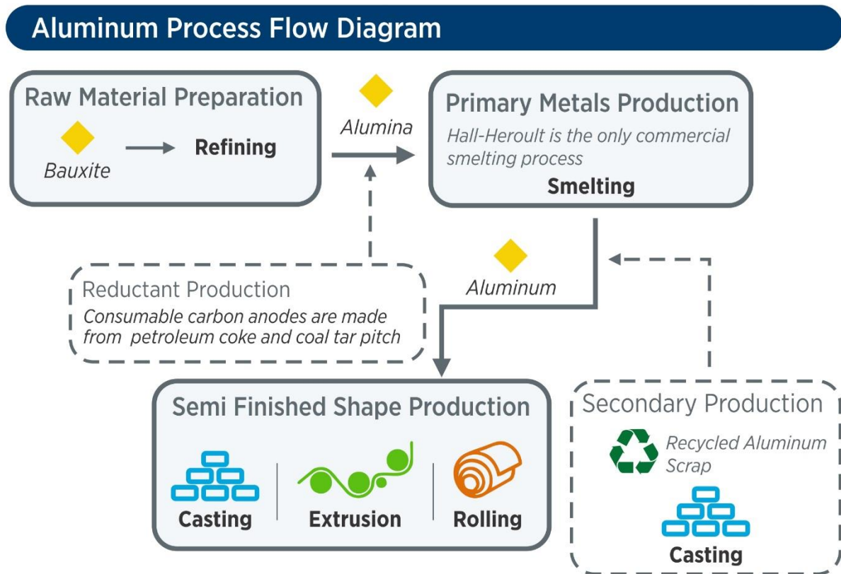
Figure 2-1. Aluminum manufacturing process flow diagram Source: EERE
