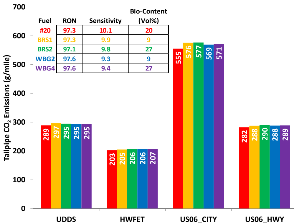
Figure 4-7. Modeled tailpipe CO 2 emissions for the mid-size sedan using the FWG matrix fuels and CR11.4 pistons.
