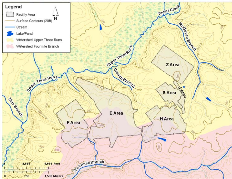
Figure 2.1-9: GSA Topography
