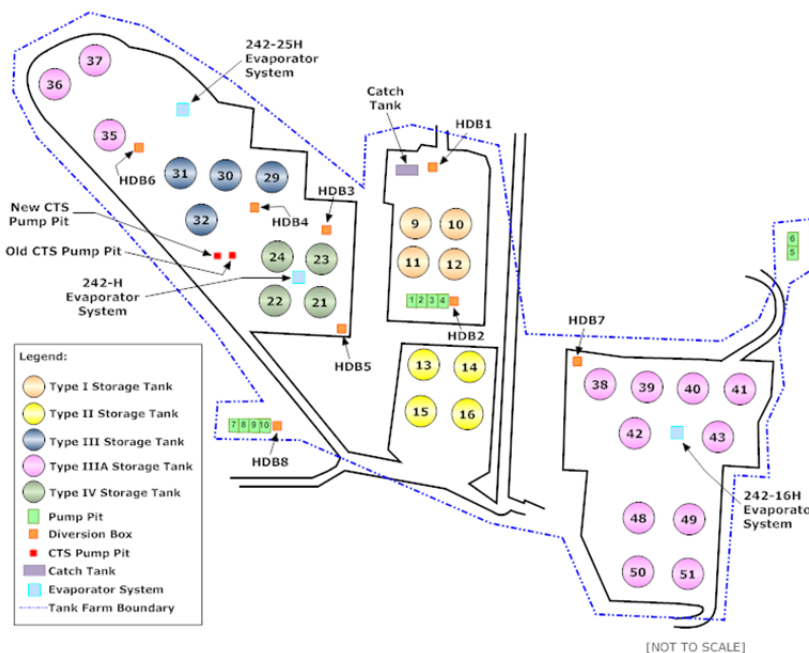
Figure 2.1-56: General Layout of HTF
