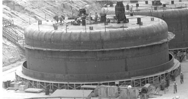
Figure 2.1-31: Type I Tank Primary and Secondary Liner Construction
