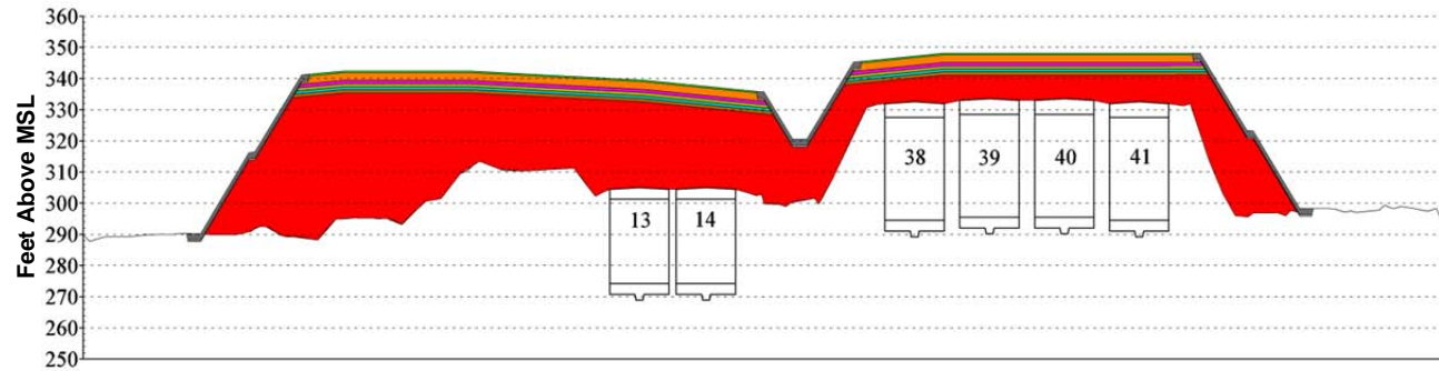
Section B-B
