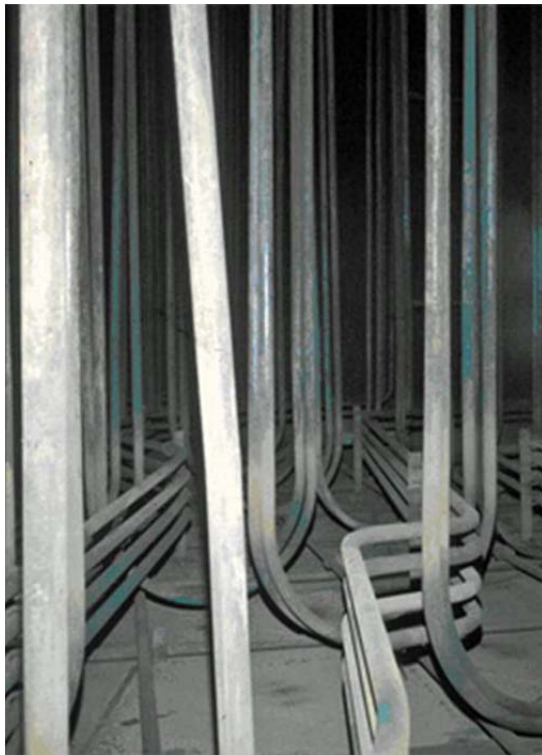
Figure 2.1-40: Typical Type II Tank Cooling Coil Obstacles
