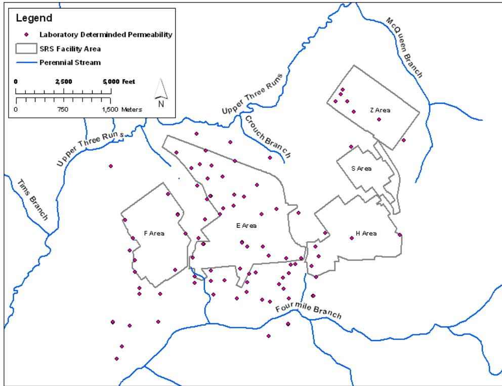
Figure 2.1-19: Laboratory Determined Permeability Data in GSAD
