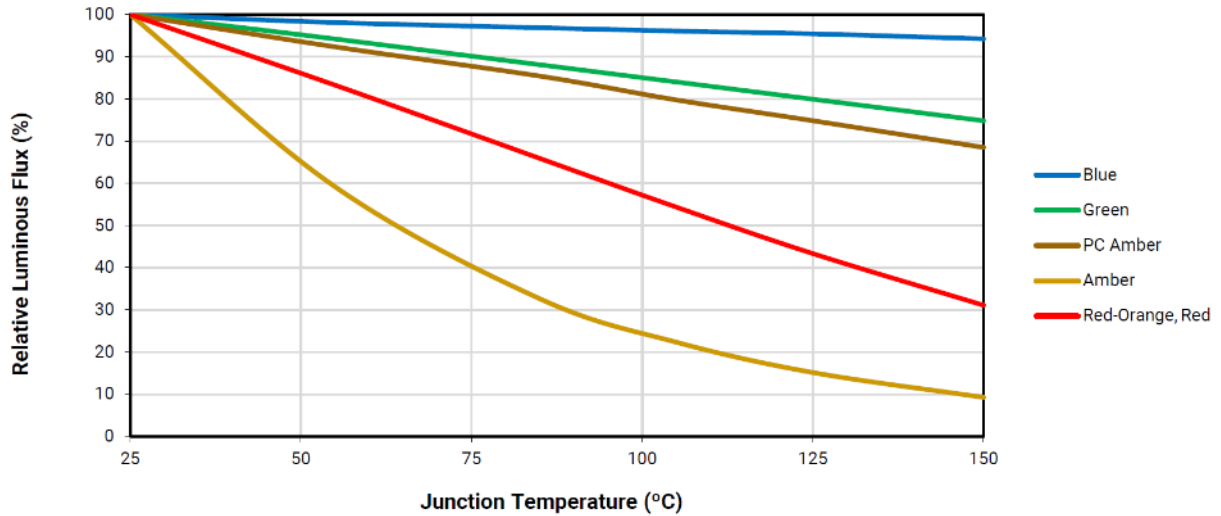
Figure 5-7. LED Efficiency as Function of Junction Temperature [16]
