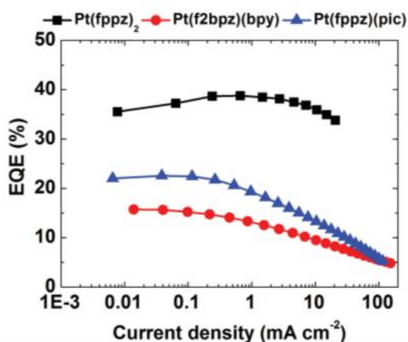
Figure 6-5. External Quantum Efficiency of Phosphorescent OLEDs with Pt-Based Emitters [51]
