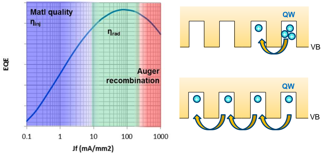
Figure 5-4. Blue LED EQE vs. Current Density and Schematic of LED Quantum Well Valence Band [14]
