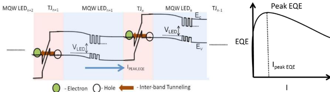
Figure 5-9. Schematic Band Diagram of a Stacked Active Region LED with Tunnel Junctions (left); the External Quantum Efficiency at the Peak LED Operating Current (right) [19]
