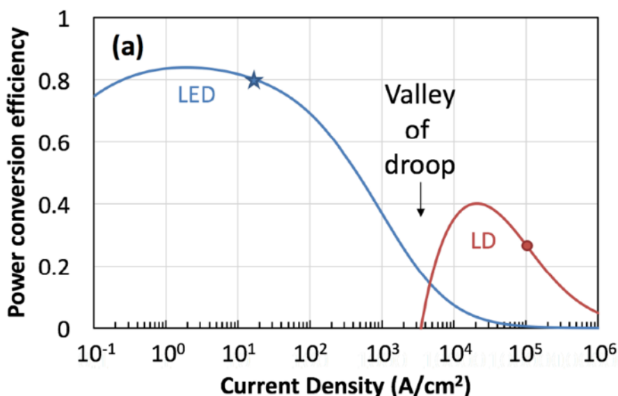
Figure 5-8. PCE Vs. Current Density for a State-of-The-Art LED and LD Emitting at Violet Wavelengths [18]
