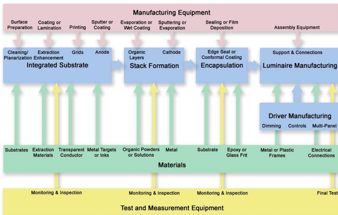
Figure 7-4. OLED-Based SSL Manufacturing Supply Chain
