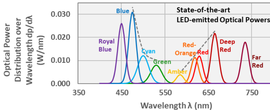
Figure 5-5. Spectral Power Densities of State-of-the-Art Commercial LEDs vs. Wavelength
