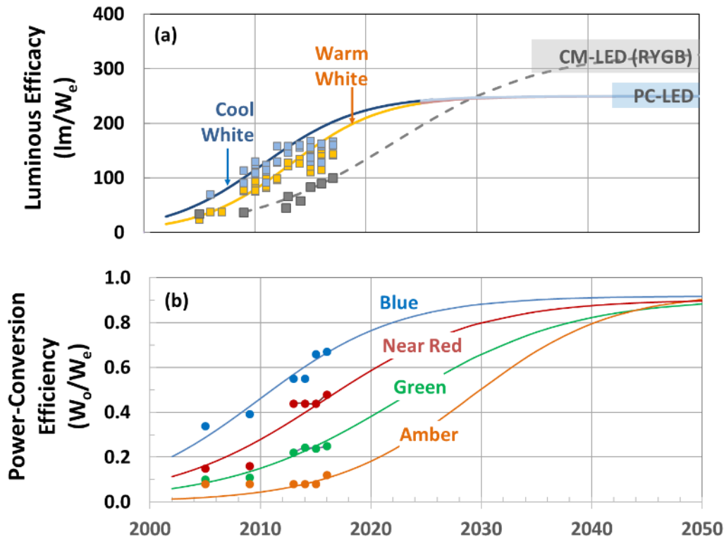
Figure 3-1. Efficiencies and Efficiencies Over Time of White and Colored LED Packages
