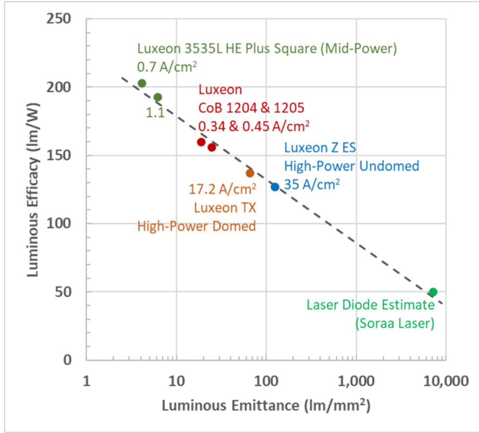
Figure 5-10. Luminous Efficacy vs. Luminous Emittances for State-of-the-Art Commercial White LEDs
