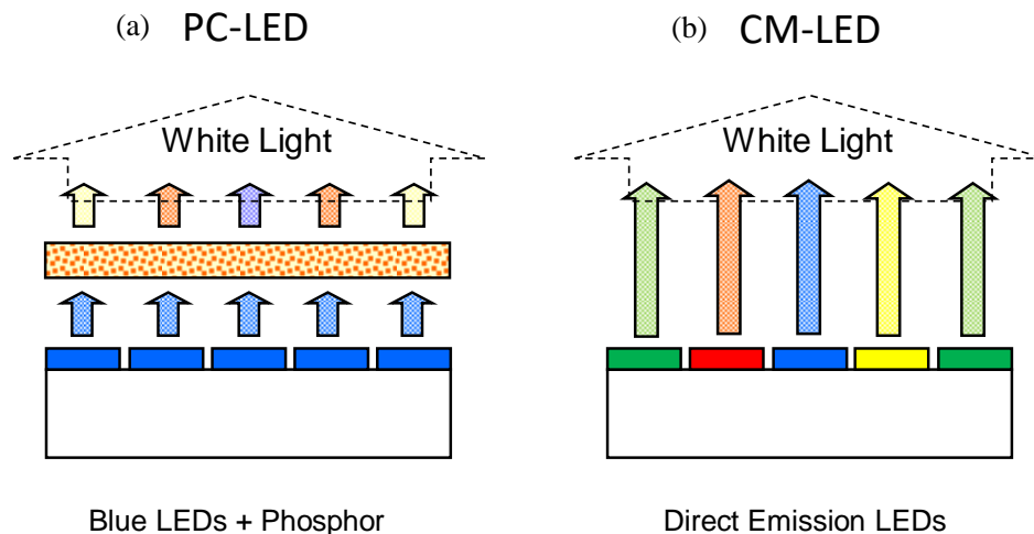
Figure 5-1. Schematic of Two Main White LED Architectures
