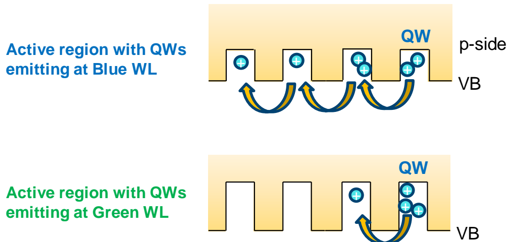
Figure 5-6. Schematic of the LED Quantum Well Valence Band [14]
