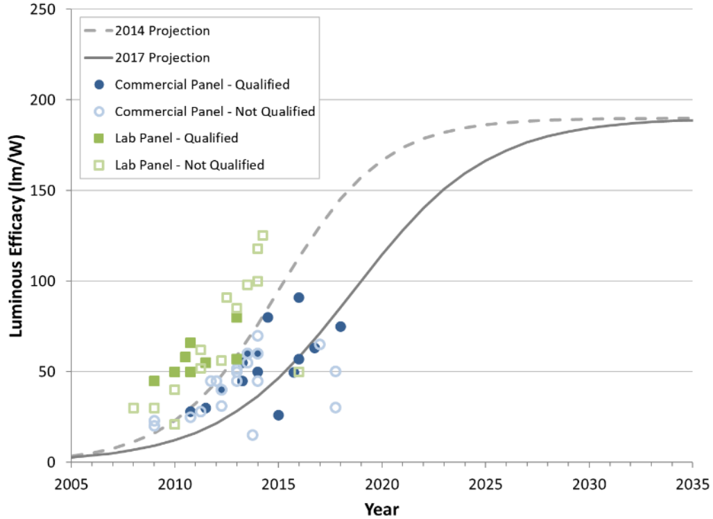
Figure 3-2. White-Light OLED Panel Efficacy Projections
