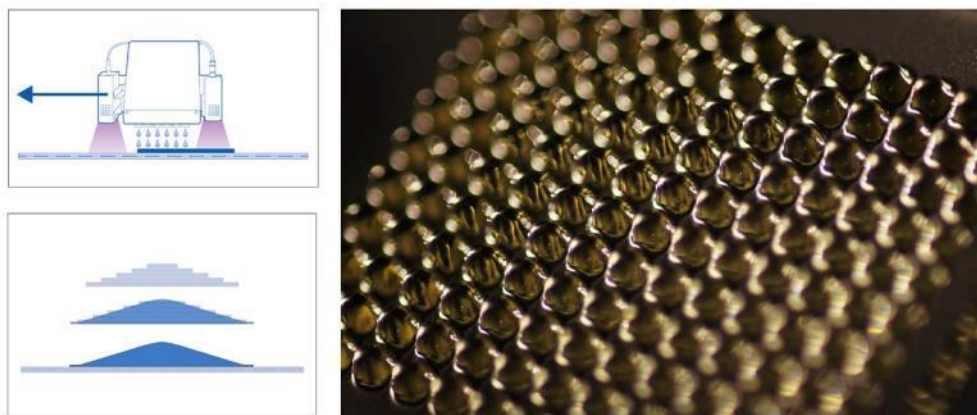
Figure 5-15. Deposition of Droplets by UV Print Head onto Substrate Material (left-top). Droplets of Polymer Are Allowed to “Flow” under Surface Tension before Curing with UV Light, giving Smooth Surfaces Needed for Optics (left-bottom). Array of Micro-Optic Lenses (right). [28]
