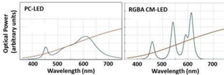
Figure 5-2. Typical Simulated Spectral Power Density for White-Light LED Package Architectures
