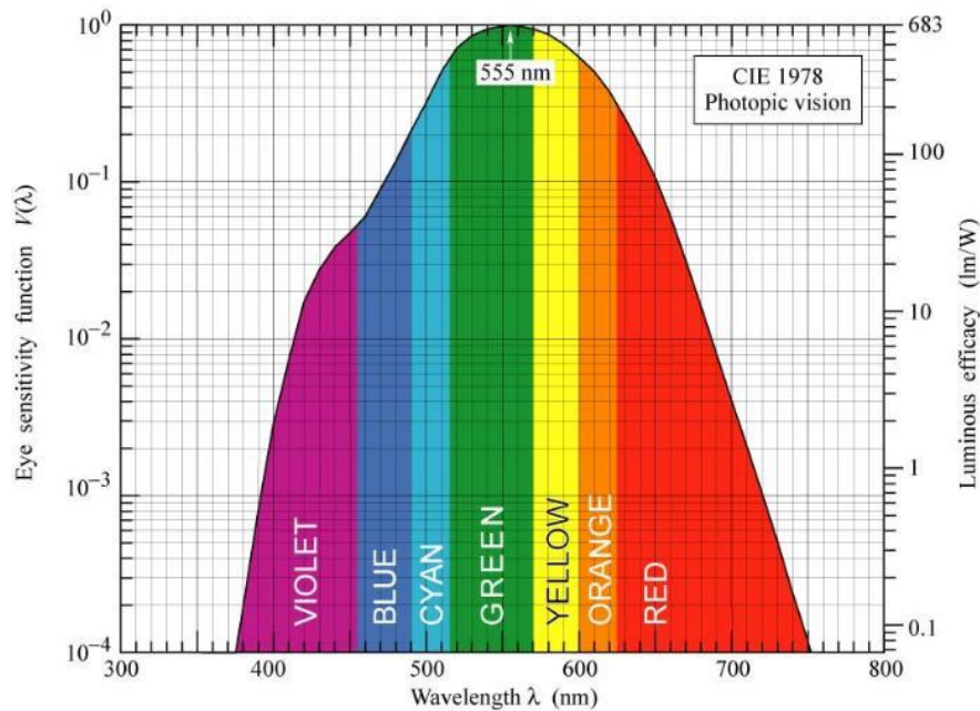
Figure 4-1. Human Eye Sensitivity Function CIE 1978 Photopic Vision
