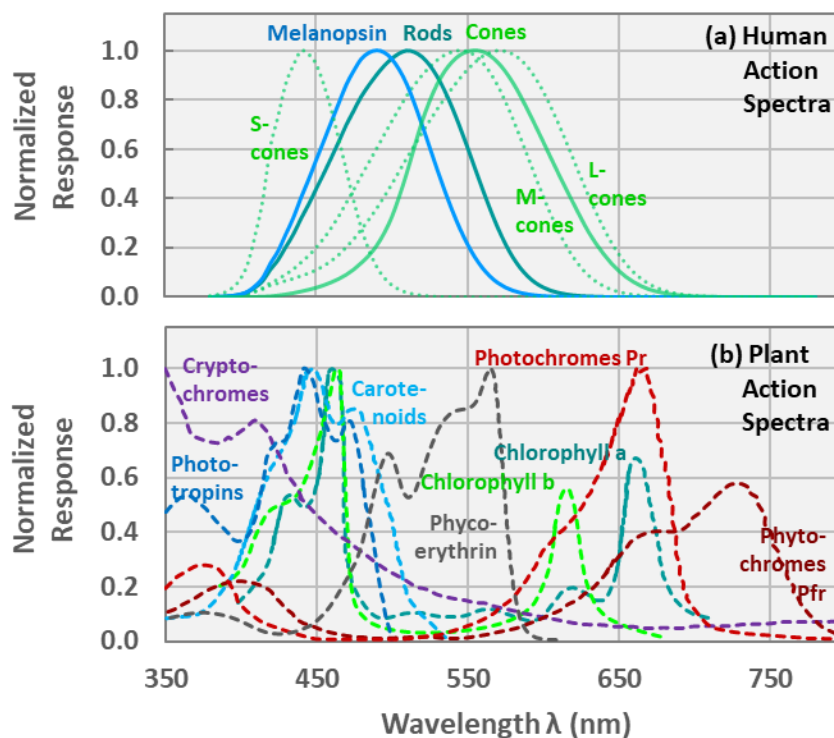
Figure 4-3. Action Spectra for Humans and Plants: (a) Human Action Spectra [4] (b) Plant Action Spectra [5]
