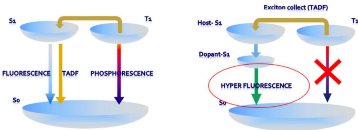
Figure 6-3. Comparison of the Mechanisms of TADF and Hyperfluorescence [41]
