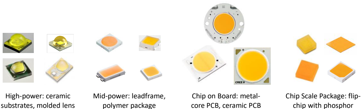
Figure 7-3. Examples of High-Power, Mid-Power, Chip-on-Board, and Chip Scale LED Packages
