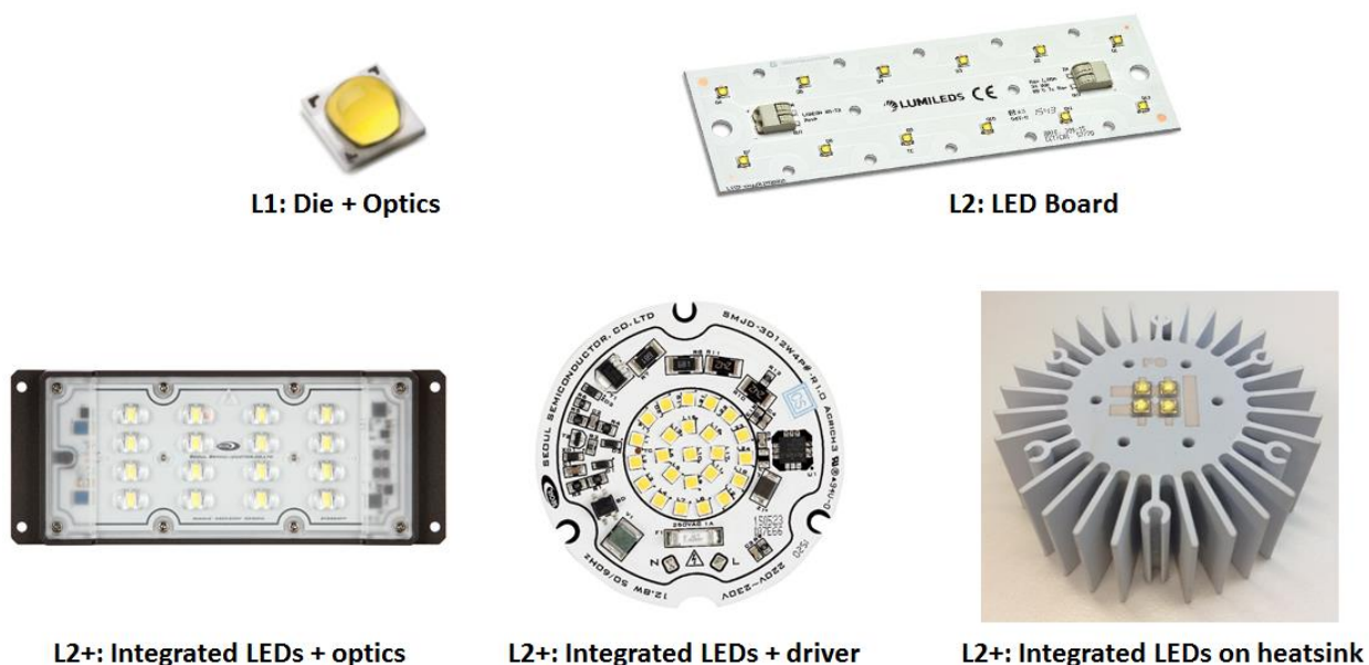
Figure 7-2. Integration Path for LED Components [61] [62] [63] [64] [65]
