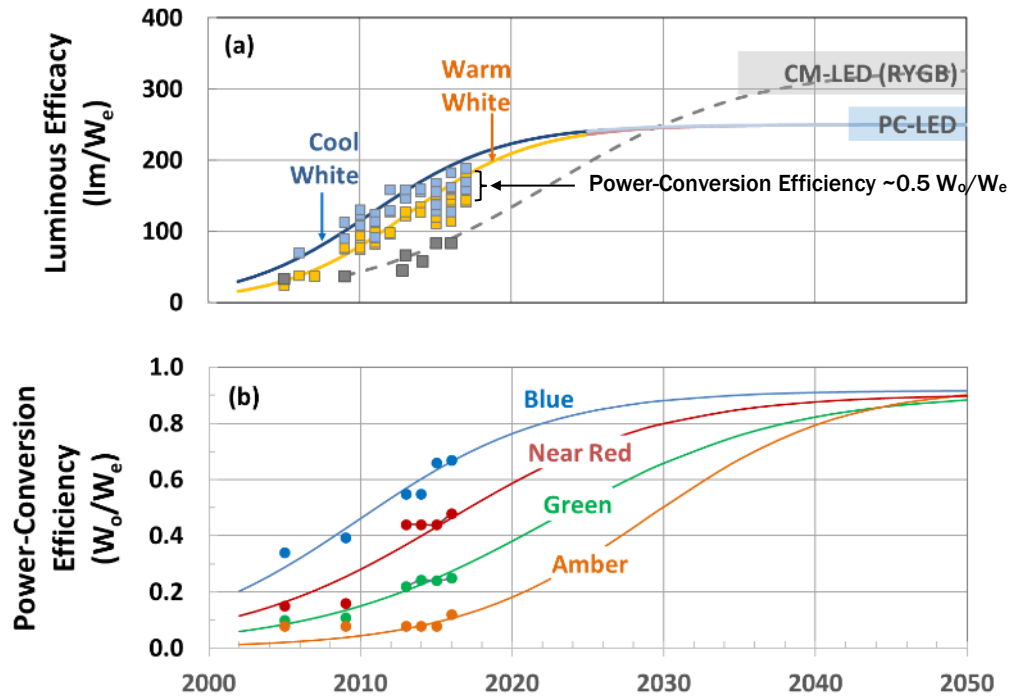
Figure 5-3. Efficacies and Efficiencies Over Time of White and Colored LED Packages
