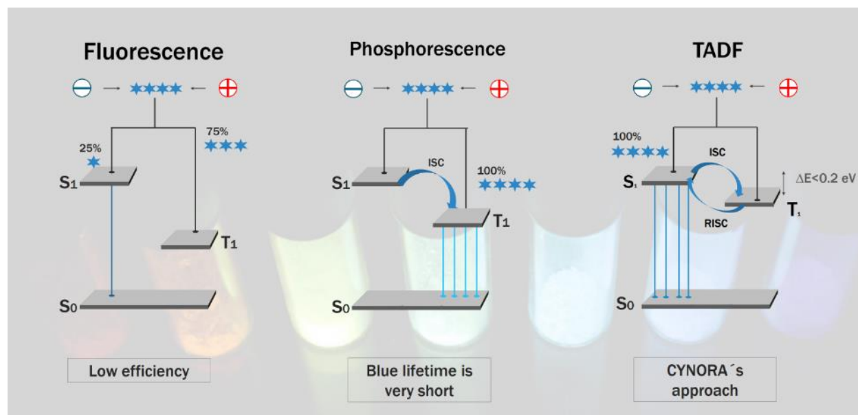
Figure 6-2. Cynora's Illustration of TADF as Compared with Fluorescent and Phosphorescent Approaches [36]
