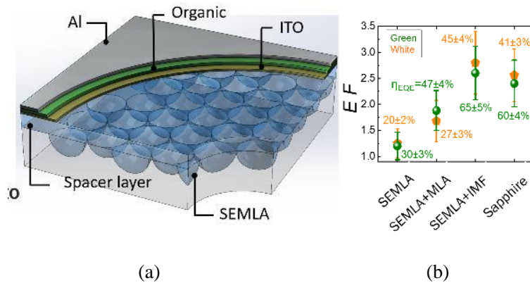
Figure 6-4. University of Michigan Sub-electrode Microlens Array Approach: (a) Device Architecture; (b) Light Extraction Enhancement Factor [46]
