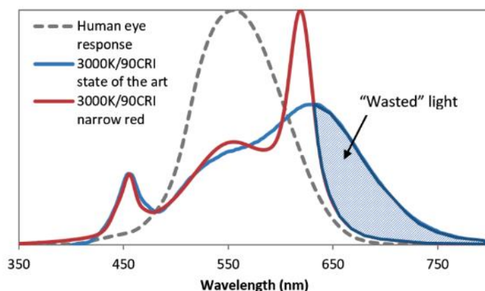
Figure 5-11. Spectrum Comparison of 90 CRI PC-LED, 90 CRI Conventional Red Phosphor LED, and Human Eye Response [20]
