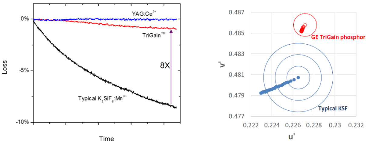
Figure 5-12. Light Loss of Phosphors in LED Packages under High Blue Flux Densities (left) and Color Shift under Stressed Operating Conditions (right) [21]
