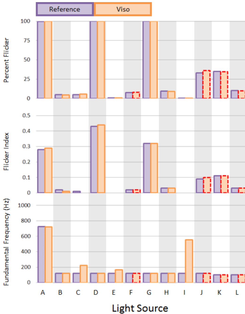
Figure 14. Viso and reference meter flicker metrics for the various light sources tested.
