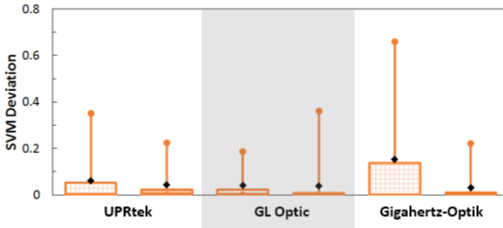
Figure 24. Comparison of handheld meter SVM calculated from waveform measurements using MATLAB and measurements from the reference meter SVM derived from the reference meter waveform using MATLAB.
