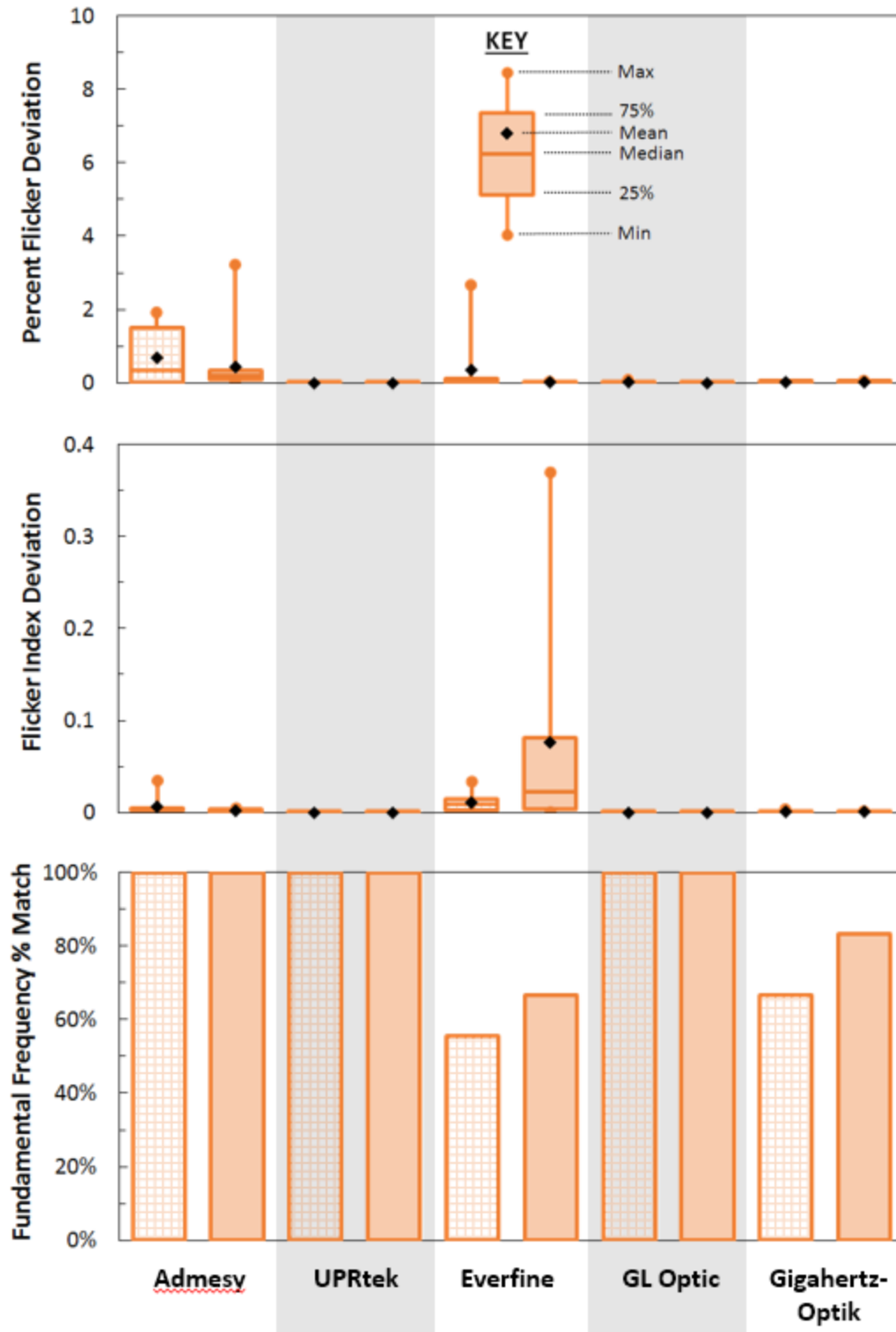
Figure 21. Comparison of the metrics reported by the meter and metrics derived from MATLAB calculations from the same meter's waveform.
