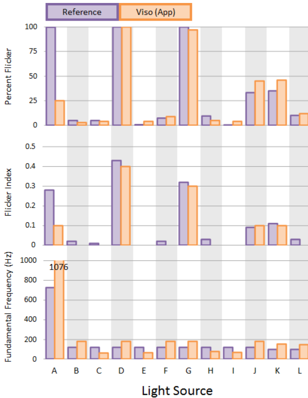
Figure 13. Viso (App) and reference meter flicker metrics for the various light sources tested.
