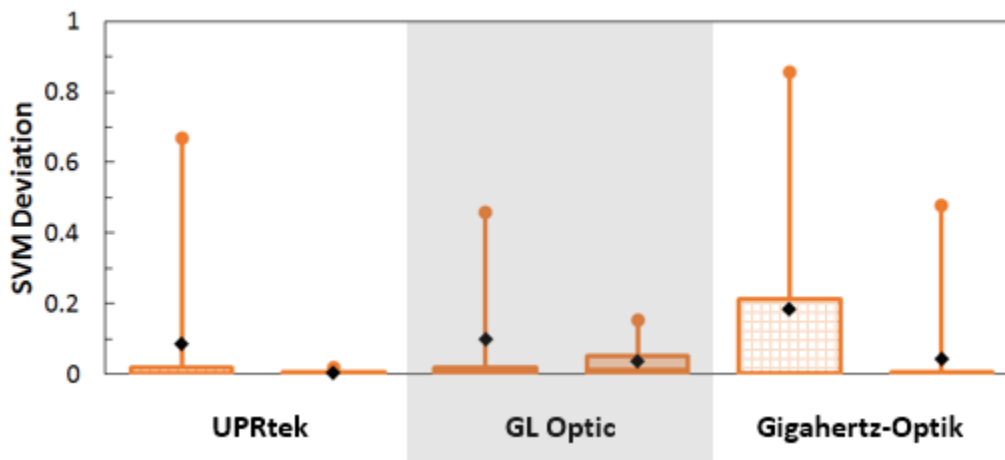
Figure 22. Comparison of SVM as reported by the meter and SVM as derived from MATLAB calculations from the same meter's waveform.
