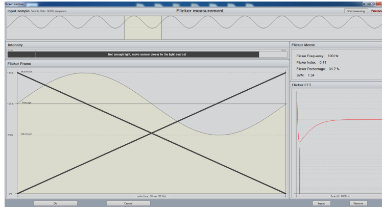
Figure 6. Viso Systems LabFlicker invalid reading.
