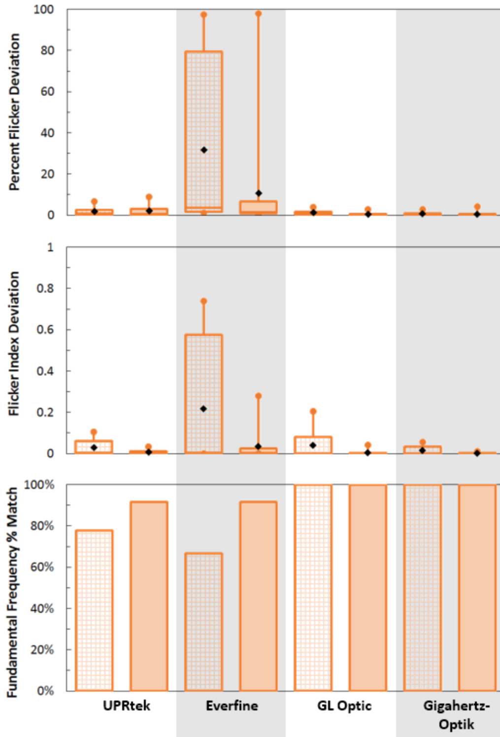
Figure 23. Comparison of handheld meter metrics calculated from waveform measurements using MATLAB and measurements from the reference meter metrics derived from the reference meter waveform using MATLAB.
