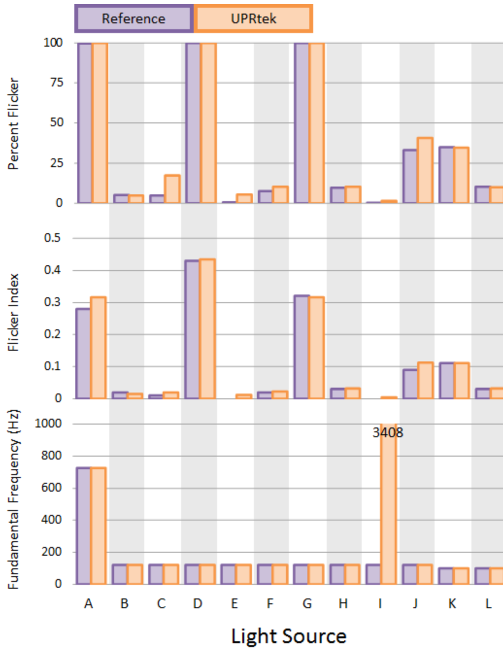
Figure 17. UPRtek and reference meter flicker metrics for the various light sources tested.
