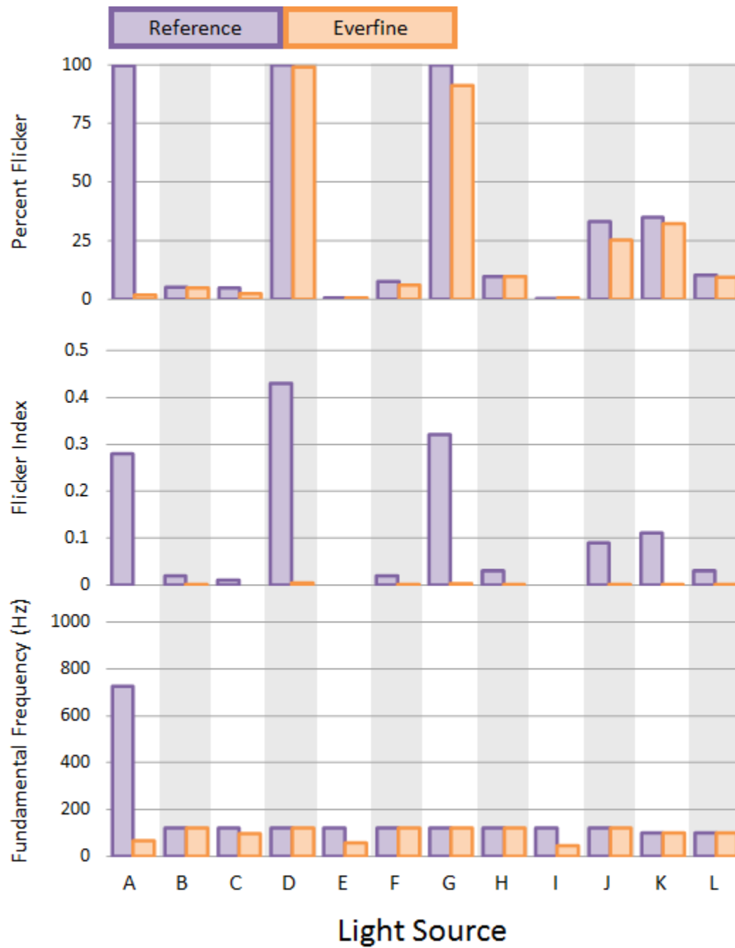
Figure 18. Everfine and reference meter flicker metrics for the various light sources tested.
