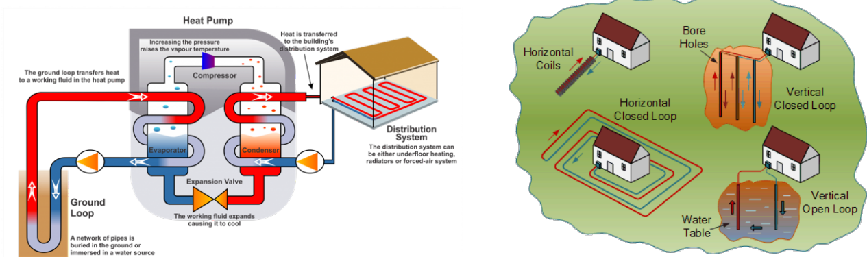
Figure 2. Ground Source Heat Pump Diagram (Left) and Ground-Loop Configuration for GSHPs (Right). On the left is a diagram of a GSHP showing the ground loop, heat pump, and distribution system. On the right, is a figure showing the different available forms of ground-loops for GSHPs.
