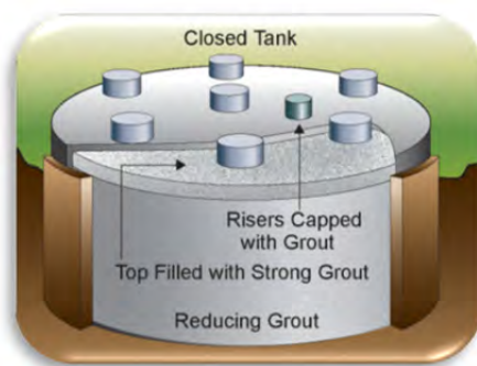
Figure 4-7 — Grouted Tank
