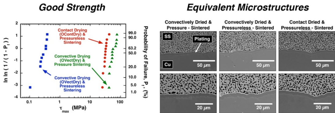
Figure I.8.2 - Convective-drying (left and middle) is different than contact-drying (right).
