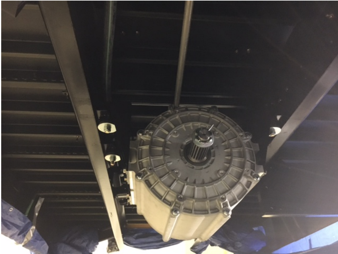
Figure II.5.1 - 3000NM Electric Motor Installed in Bus P1
