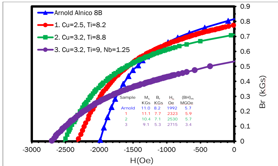
Figure I.13.1 - Demagnetization curves with peak value of H_{cj} is obtained when the volume fraction of L2_1 phase approaches to \sim 50\% . A recorded H_{cj} of 2715 Oe is achieved. On the other hand, M_s and B_r decreases due to the reduction of FeCo phase.
