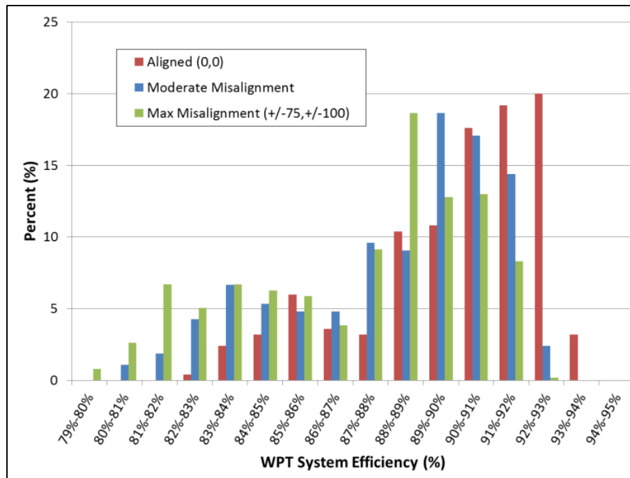
Figure V.2.2 - Efficiency Results from Interoperable Bench Testing of Wireless Charging Systems (Source: INL)
