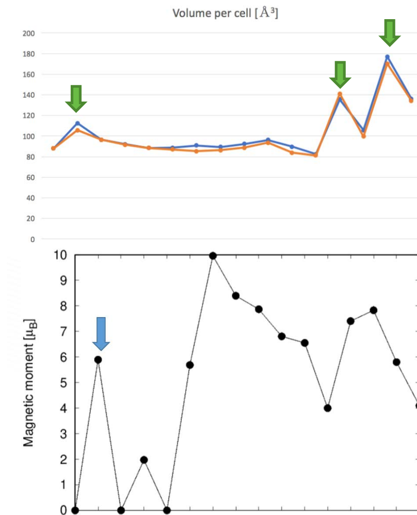
Figure I.10.3 - Change in the unit cell volume of B2 structure (Fe-Si) with ternary alloying addition. Two additional elements (#13 and #15, indicated by arrows) were identified that had higher volume change compared with previously identified element #2.
