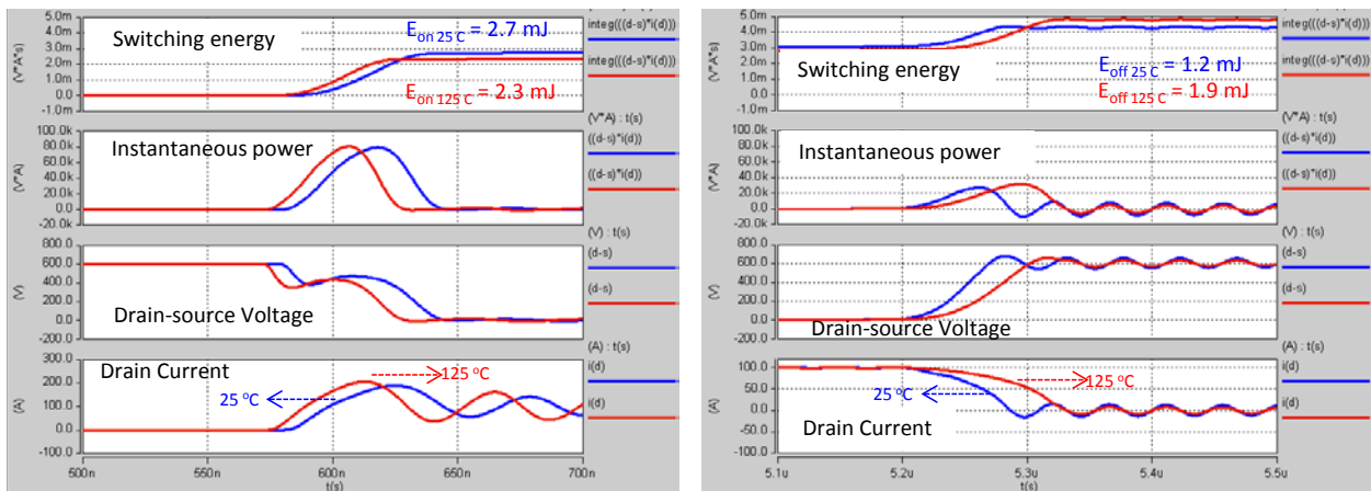
Figure I.6.3 - Simulated switching transient of SiC MOSFET: turn-on transient (left) and turn-off transient (right).
