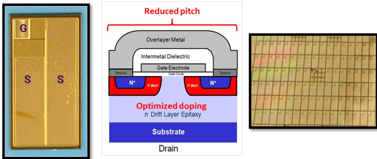
Figure II.6.1 - 650V, 7m \Omega , 37mm ^2 SiC MOSFET die shown singular (left image), cross-section (center image), and on-wafer (right image)
