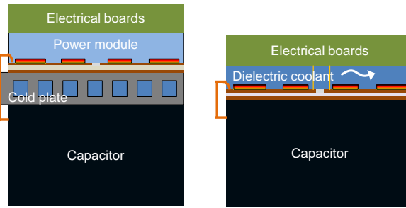
Figure I.16.5 - Schematics of two compact-packaging inverter concepts. The concept on the left uses a thin cold plate between the modules and capacitors. The concept on the right directly cools the devices and electrical interconnections using a dielectric fluid.
