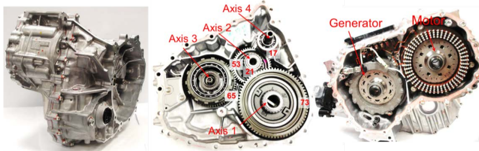
Figure I.7.6 - 2017 Prius transmission/transaxle.
