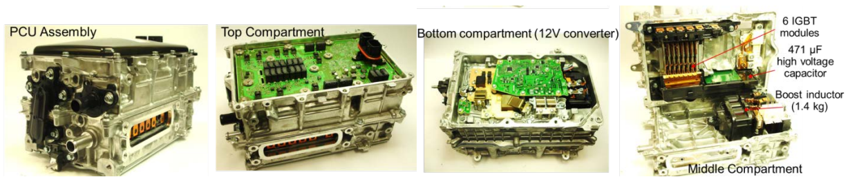
Figure I.7.1 - 2017 Prius PCU assembly and compartments.
