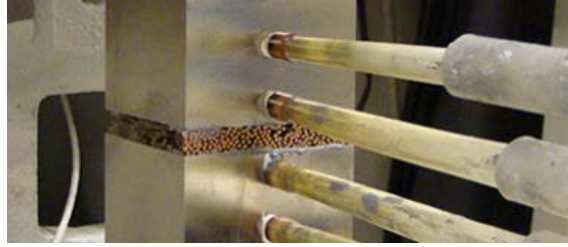
Figure I.15.2 - Sample winding thermal transmission testing Photo Credit: Emily Cousineau, NREL
