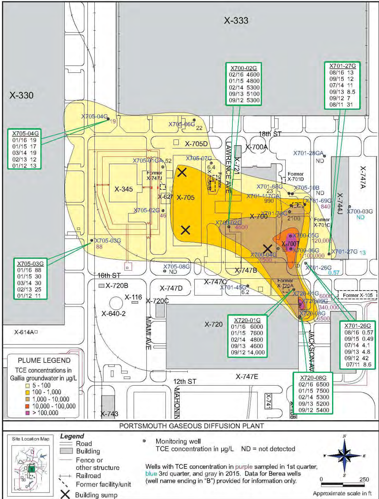
Figure 6.4. TCE-contaminated Gallia groundwater plume at the Quadrant II Groundwater Investigative (7-Unit) Area – 2016.
