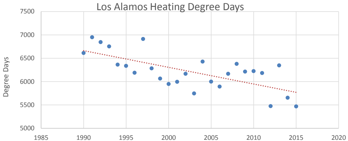
Figure 2-8 Los Alamos heating degree days
