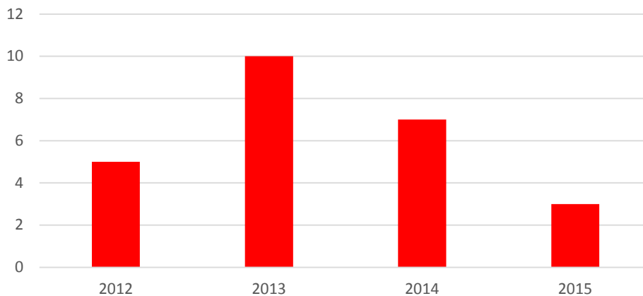
Figure 2-10 Number of National Weather Service red flag warning days for zone 102 (Los Alamos)
