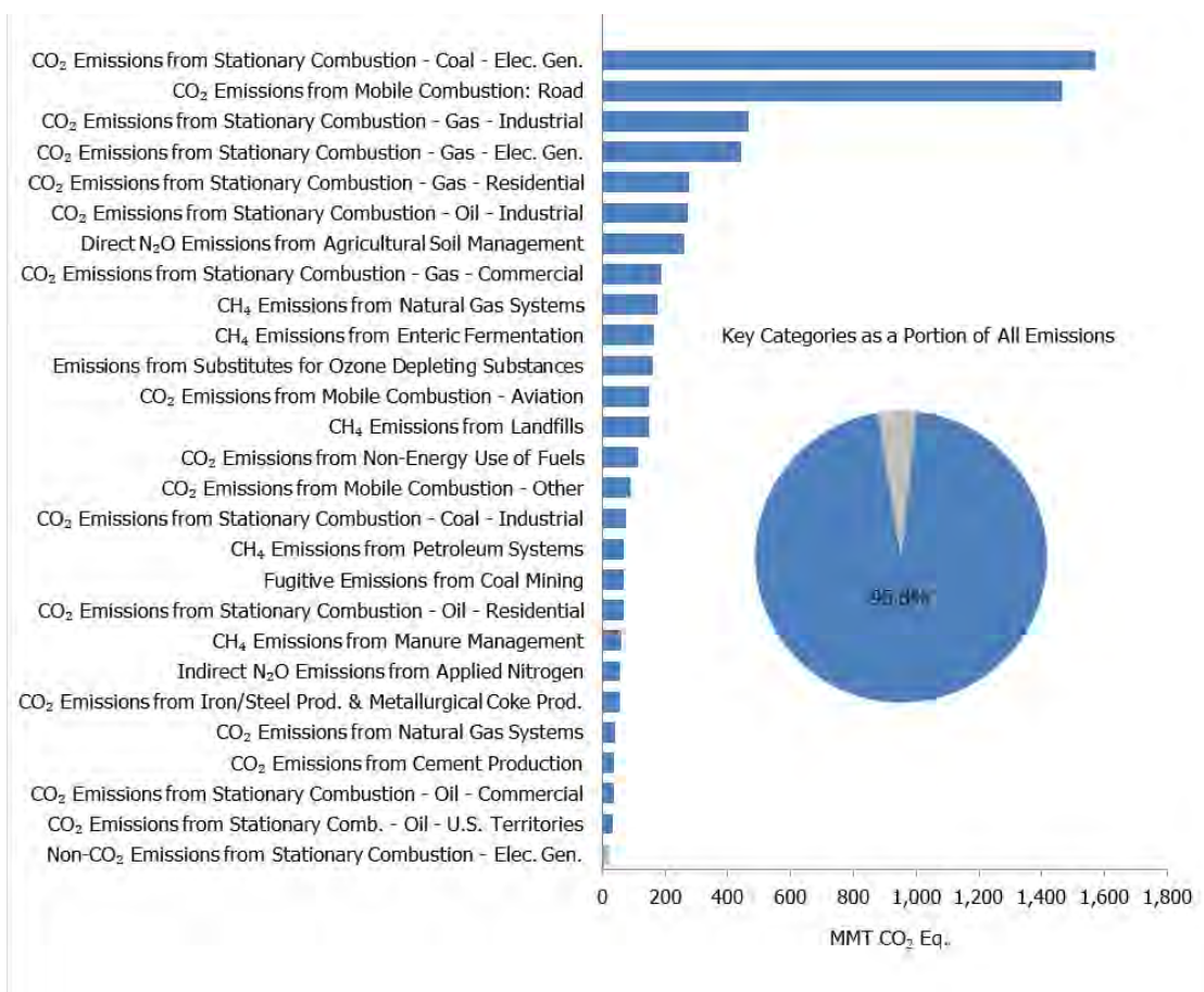
Figure ES-16: 2014 Key Categories (MMT CO 2 Eq.)
