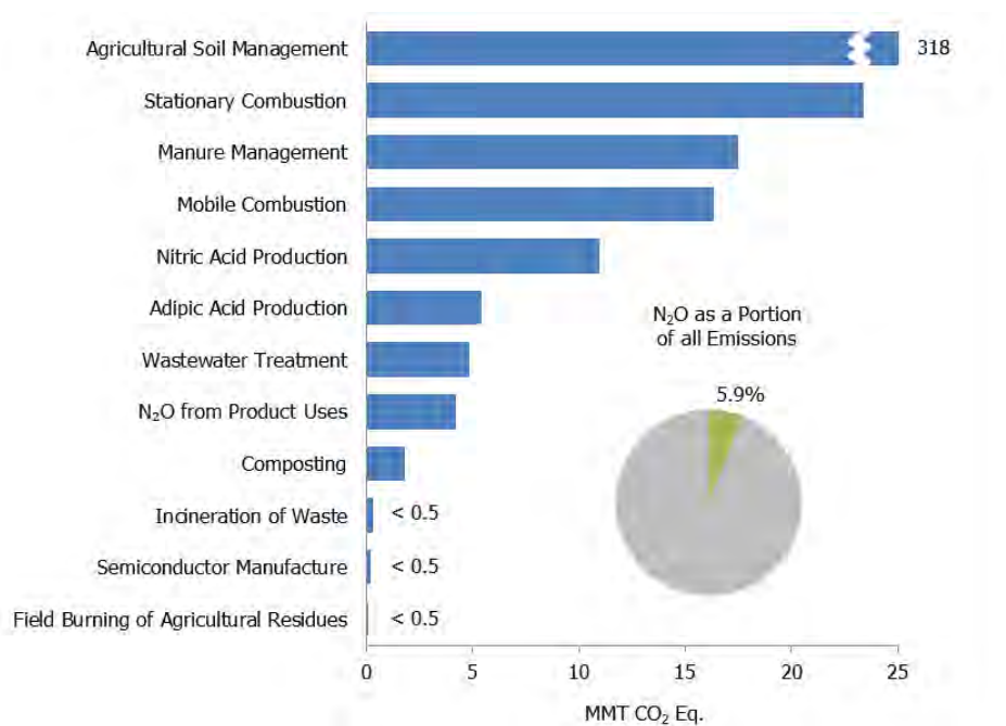
Figure ES-9: 2014 Sources of N 2 O Emissions (MMT CO 2 Eq.)
