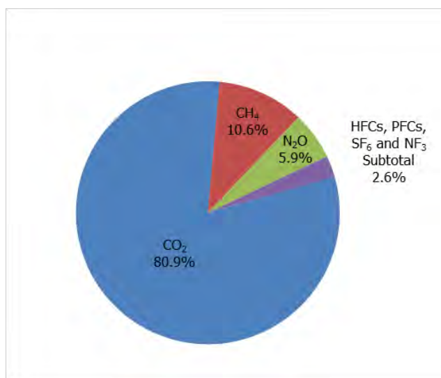
Figure ES-4: 2014 U.S. Greenhouse Gas Emissions by Gas (Percentages based on MMT CO 2 Eq.)
