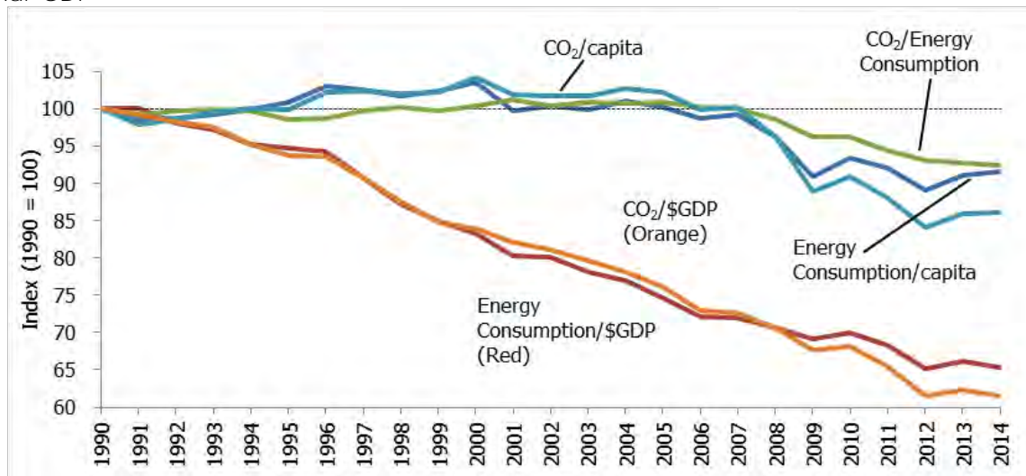
Figure 3-14: U.S. Energy Consumption and Energy-Related CO 2 Emissions Per Capita and Per Dollar GDP
