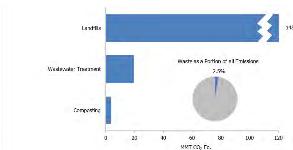
Figure 7-1: 2014 Waste Chapter Greenhouse Gas Sources (MMT CO 2 Eq.)
