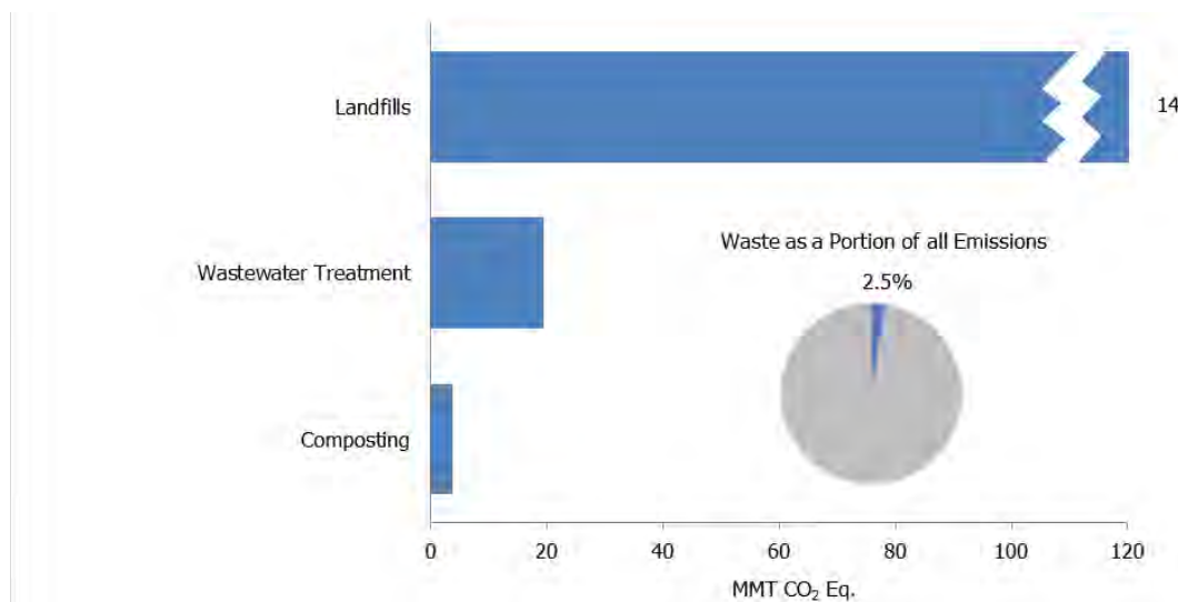
Figure 2-11: 2014 Waste Chapter Greenhouse Gas Sources (MMT CO 2 Eq.)
