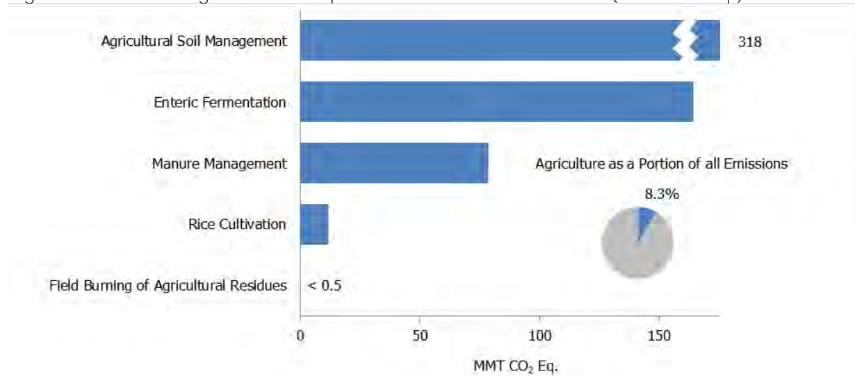
Figure 2-10: 2014 Agriculture Chapter Greenhouse Gas Sources (MMT CO 2 Eq.)
