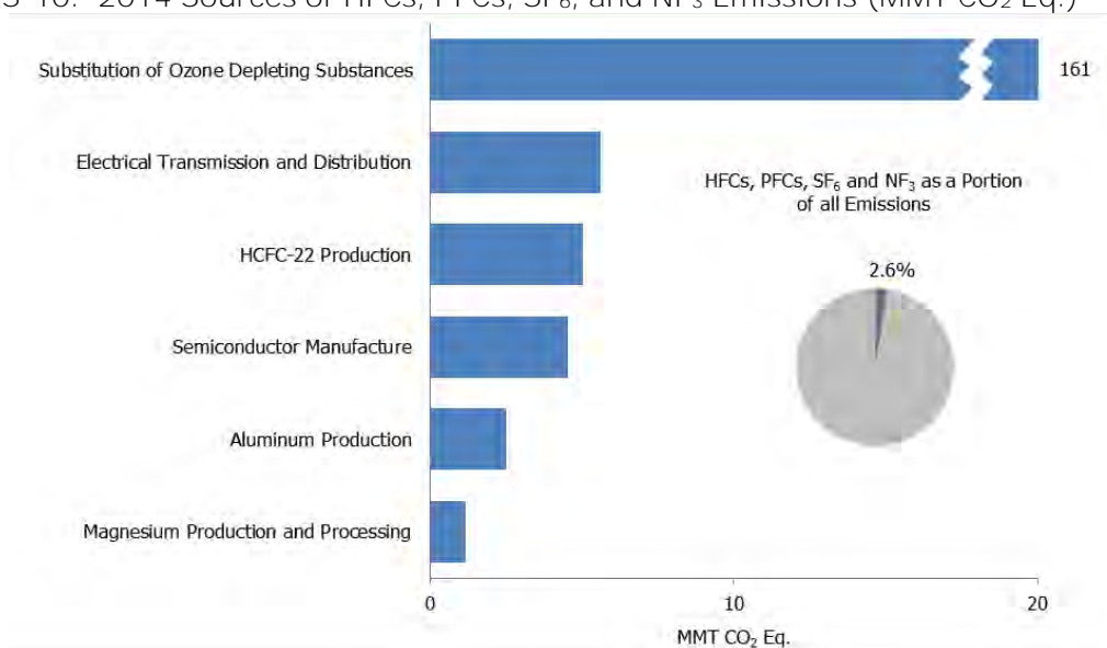
Figure ES-10: 2014 Sources of HFCs, PFCs, SF 6 , and NF 3 Emissions (MMT CO 2 Eq.)
