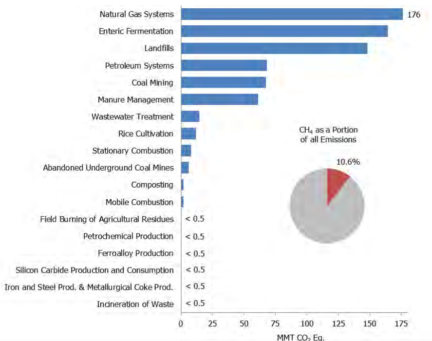
Figure ES-8: 2014 Sources of CH 4 Emissions (MMT CO 2 Eq.)
