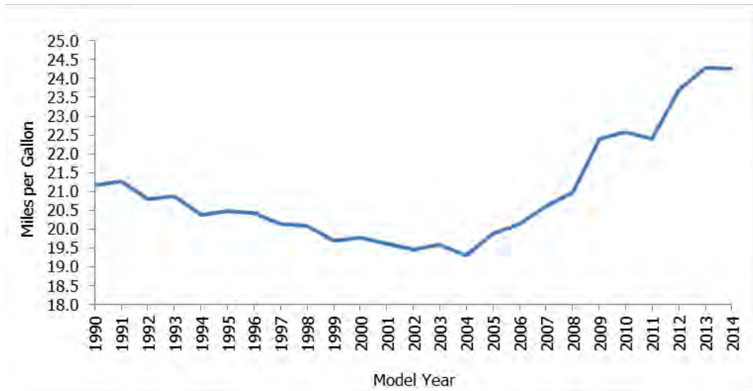
Figure 3-11: Sales-Weighted Fuel Economy of New Passenger Cars and Light-Duty Trucks, 1990–2014 (miles/gallon)
