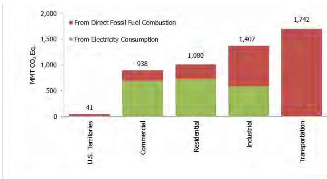
Figure 2-8: 2014 End-Use Sector Emissions of CO 2 from Fossil Fuel Combustion (MMT CO 2 Eq.)
