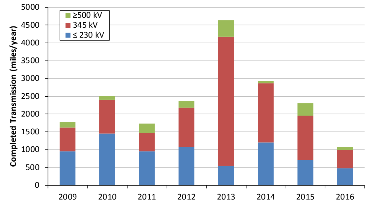
Figure 54. Miles of transmission projects completed, by year and voltage
