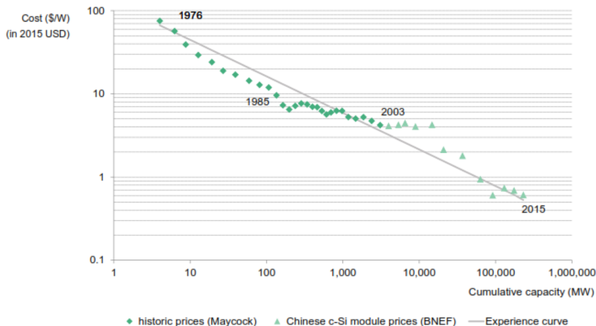
Figure 17: Experience Curve for PV Modules 78
