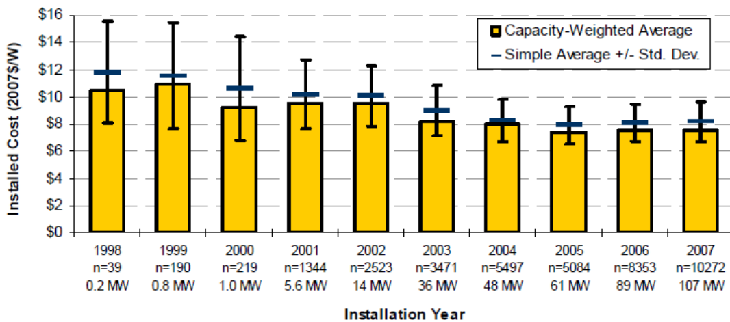
Figure 8: Installed Cost Trends for Photovoltaic Systems in the U.S., 1998-2007 41
