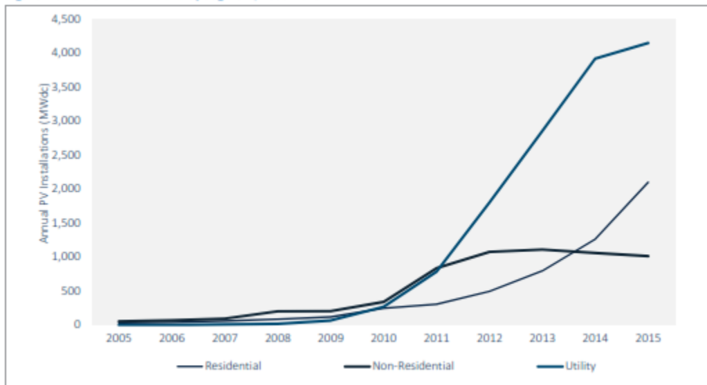
Figure 19: Annual PV Installations by Segment, 2005-2015 81
