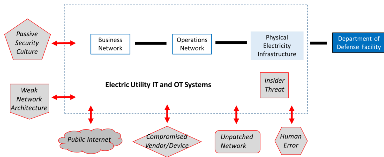
Figure 1-5. Example Cyberattack Vectors for an Electric Utility 121
