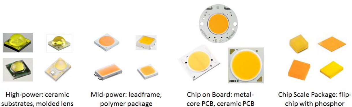
Figure 5.11 Examples of High-Power, Mid-Power, Chip-on-Board and Chip Scale LED Packages
