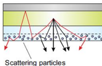
Figure 6.4 Internal Extraction Schematic
