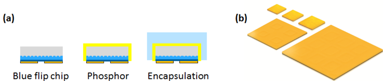
Figure 5.12 (a) CSP Manufacturing Approach and (b) Recent Example of the Scalability of Commercial CSPs.
