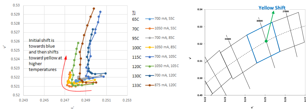
Figure 5.23 The Color Shift of a Representative High Power Package Indicating a Steady Yellow Shift
