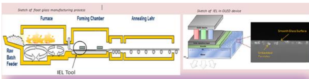
Figure 6.26 IEL Layer Applied in a Float Glass Manufacturing Process
