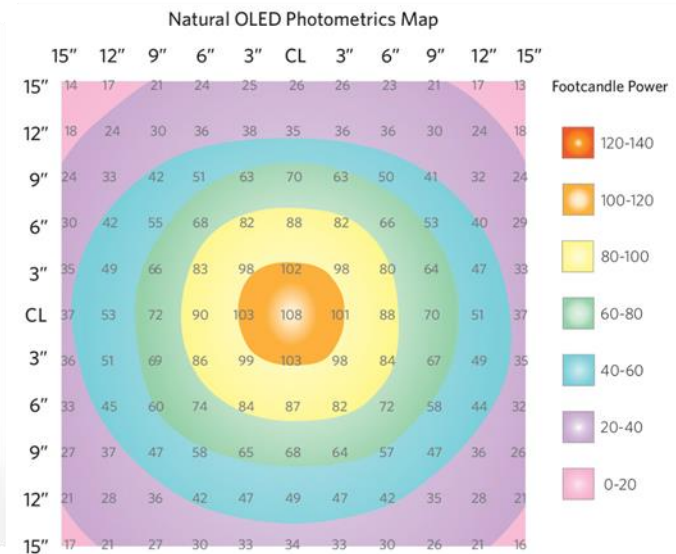
Figure 2.3 Distribution Comparison of Workrite Ergonomics' (a) Astra 2.0 Single Arm (LED) Desk Light and (b) Natural OLED Desk Light
