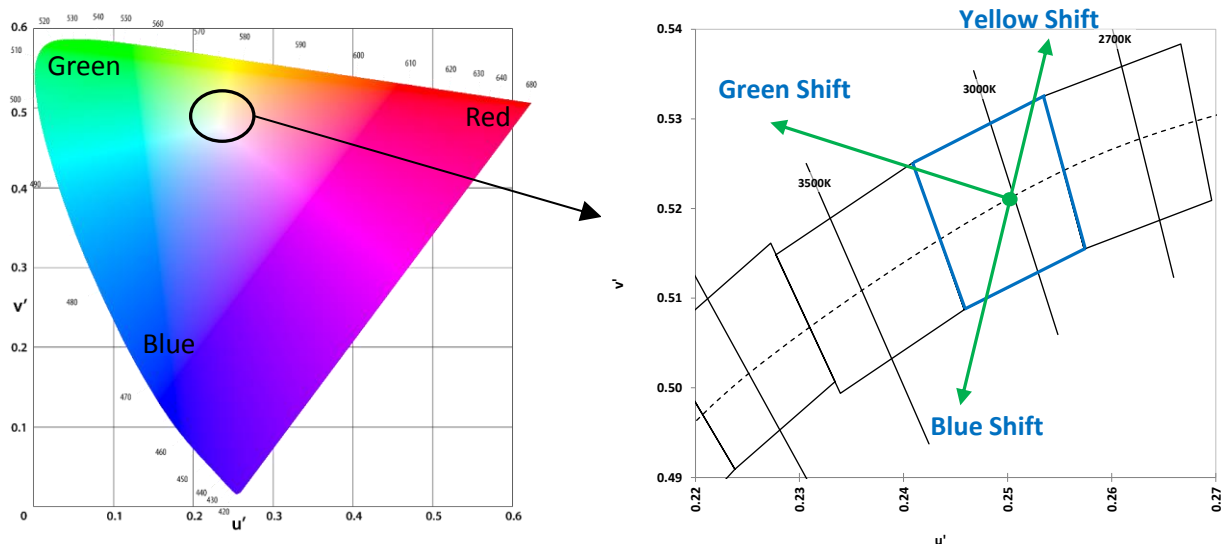
Figure 5.22 1976 CIE Chromaticity Diagram Illustration the Common Directions of Color Shift in LED Packages
