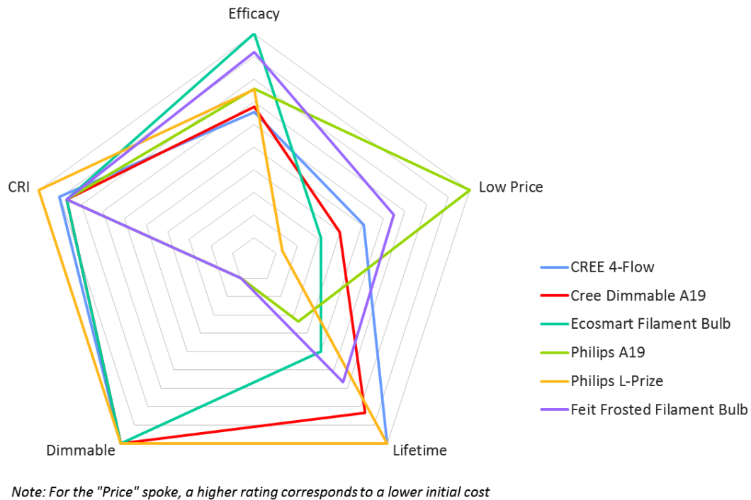
Figure 5.16 Comparison of Quality Tradeoffs for Various A-Type LED Lamps
