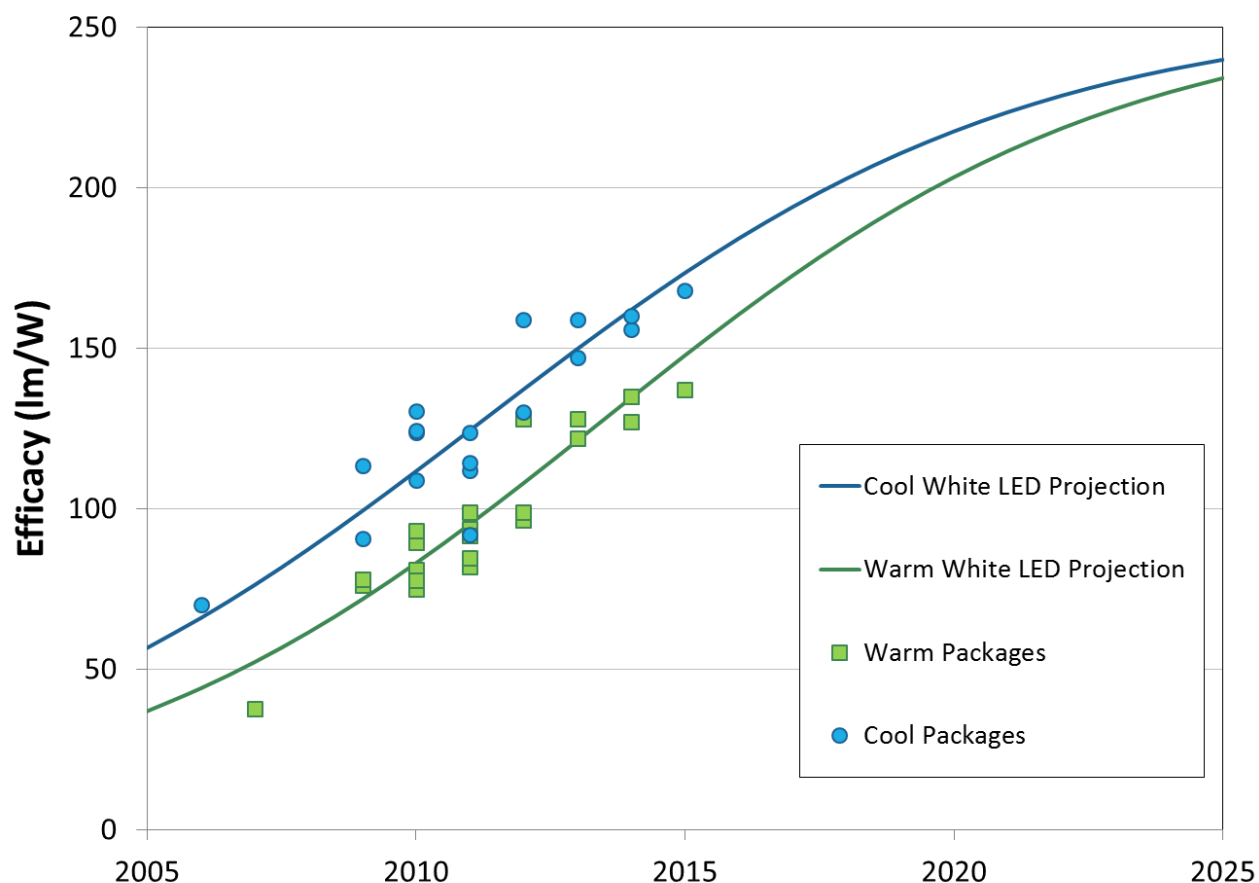
Figure 7.2 LED Package Efficacy Projections for Commercial Products
