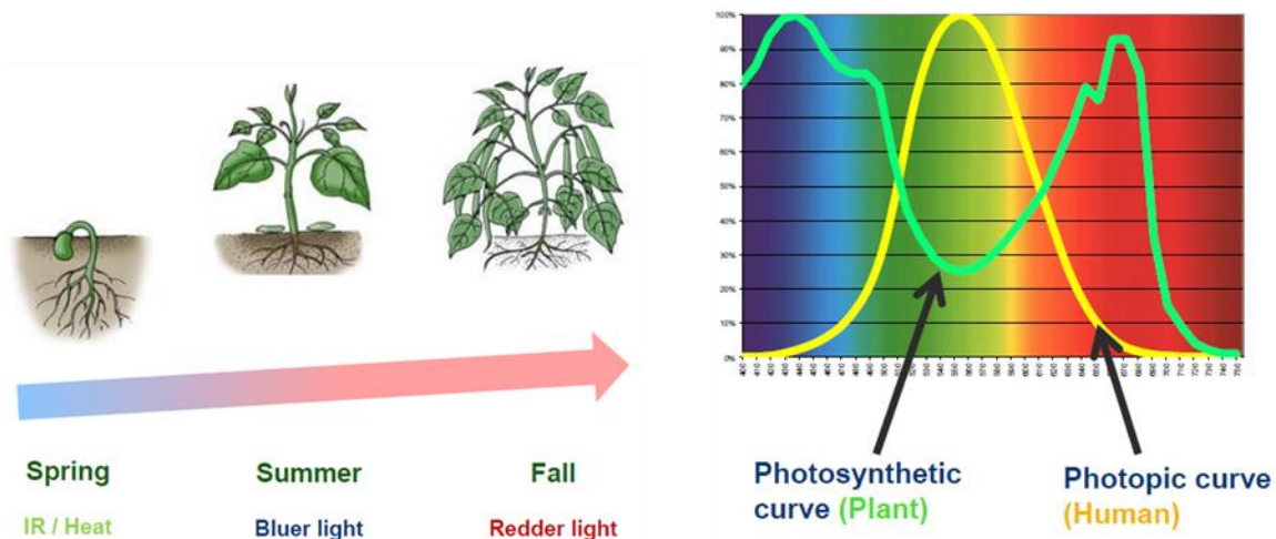
Figure 2.10 Effect of Light on Plant Growth
