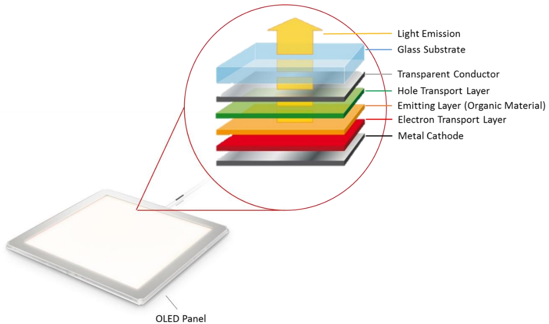
Figure 8.2 Components of an OLED Panel
