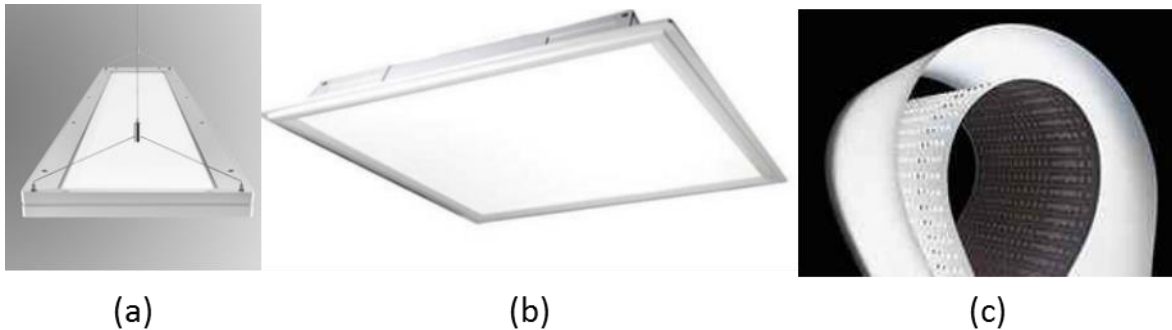
Figure 6.20 (a) GE Edge-Lit Panel (b) Maxlite Direct-Lit Luminaire (c) Cooledge Flexible Direct-Lit Technology
