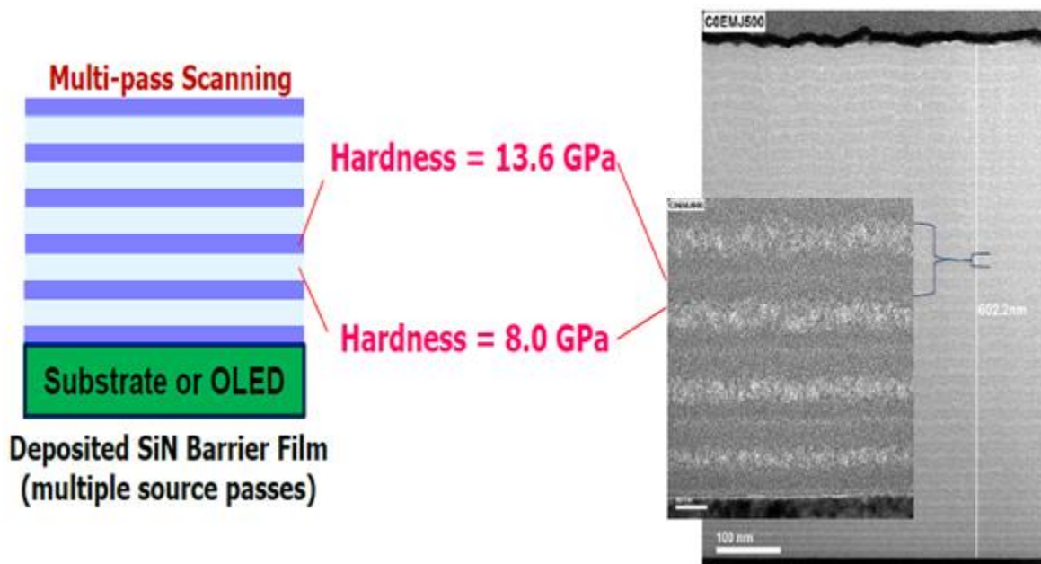
Figure 6.24 Multi-Stack Barriers with Alternating Inorganic Layers of Varying Hardness (Aixtron) Source: Juergen Kreis, Aixtron, "Cost Efficient OLED Manufacturing," Smithers Apex OLED World Summit, October 2015 [172]
