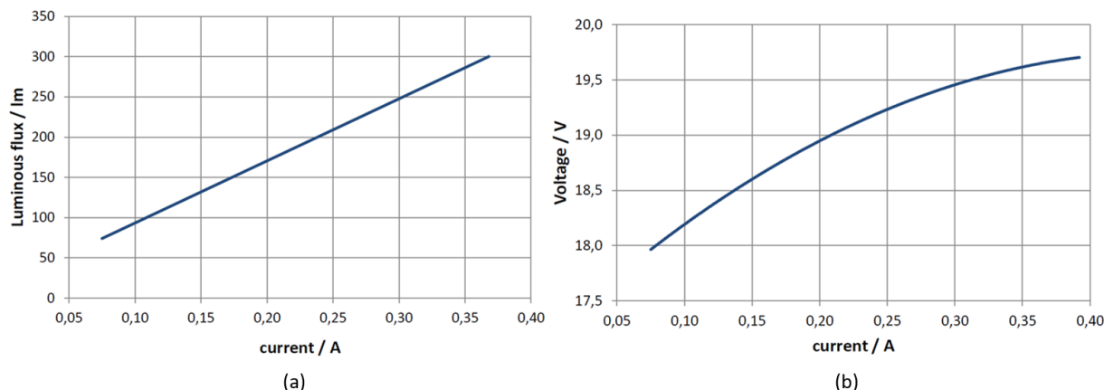
Figure 6.2 Dependence of (a) Luminous Flux and (b) Drive Voltage on Current
