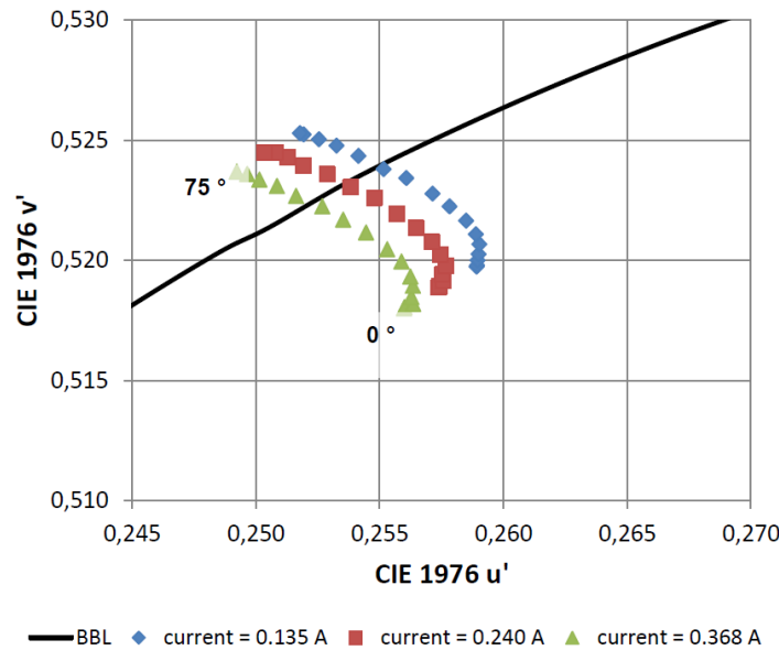
Figure 6.9 Variation of Color Point on CIE1976 ( u' , v' ) Diagram with Drive Current and Emission Angle Source: OLEDWorks FL300 Datasheet, 2016 [111]
