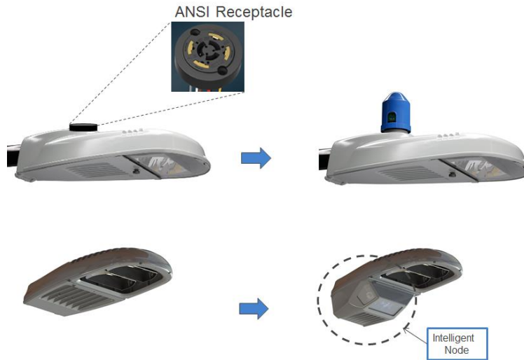
Figure 4.7 LED Lighting Street Light Fixtures Showing the Location of Integrated Sensors
