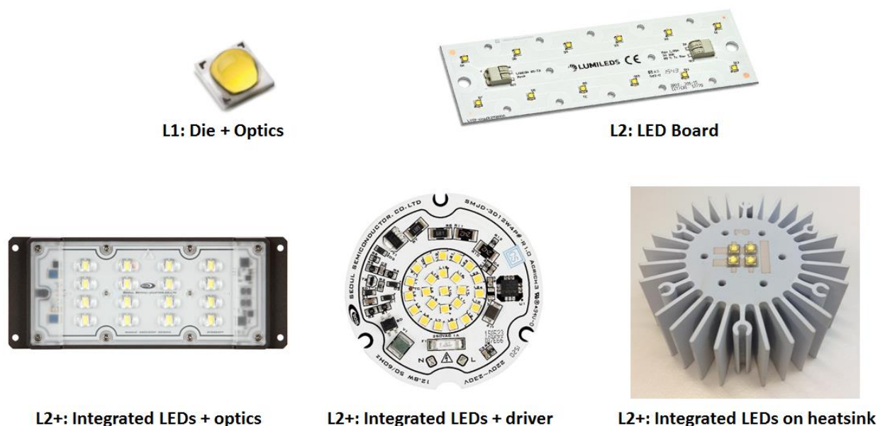
Figure 5.10 Integration Path for LED Components
