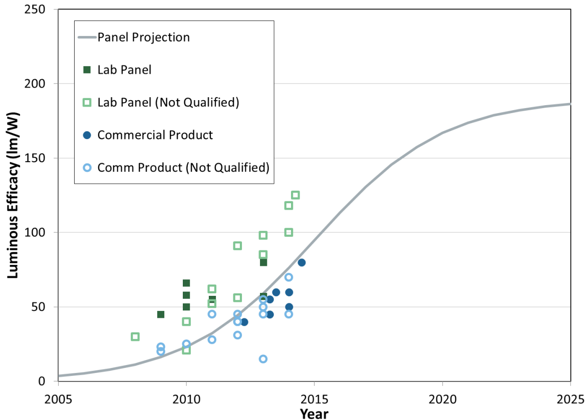
Figure 7.3 White-Light OLED Panel Efficacy Projections
