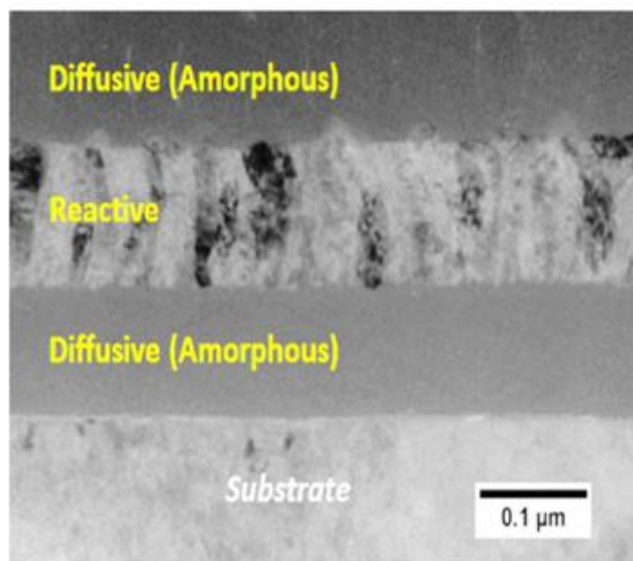
Figure 6.25 Multi-Stack Barriers with Alternating Inorganic Layers of Varying Hardness (Vitriflex) Source: Ravi Prasad, Vitriflex, “Transparent Barrier Films,” OLED Stakeholder meeting, Pittsburgh, September 2015 [174]
