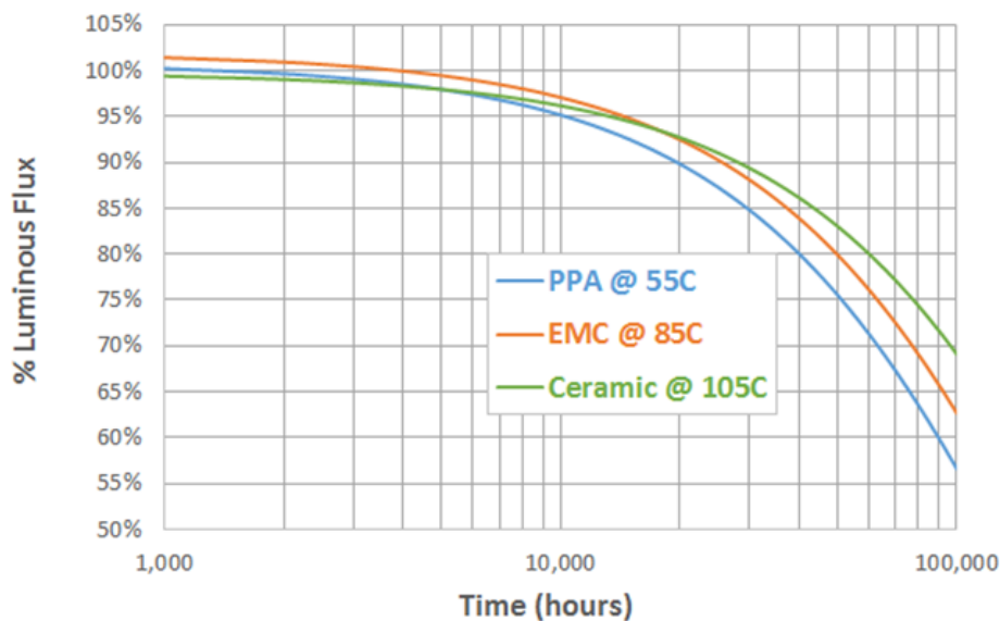
Figure 5.20 Lumen Degradation Performance of Typical Mid-Power Packages (PPA and EMC Plastic Resins) and High Power Packages (Ceramic Substrates).
