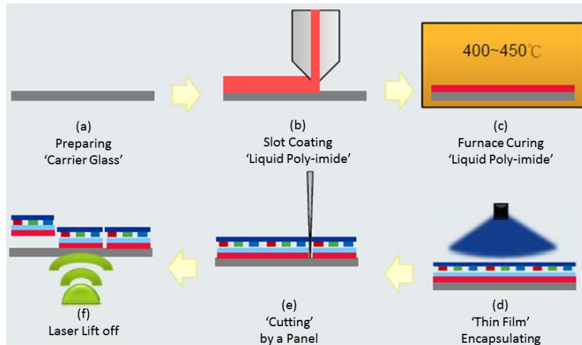
Figure 6.32 Use of Carrier Glass in Fabrication of OLED Panels on Plastic Substrates
