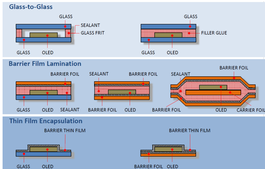
Figure 6.28 Alternative Approaches to OLED Encapsulation
