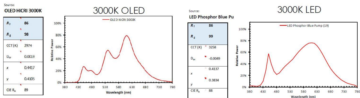
Figure 6.8 TM-30 Comparison of OLED and LED, 3000K
