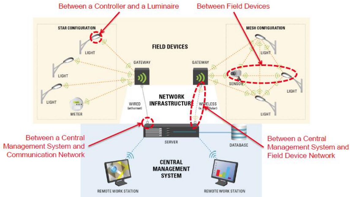
Figure 4.4 Lights, Sensors, Meters, Gateways, and Management Systems Working Together
