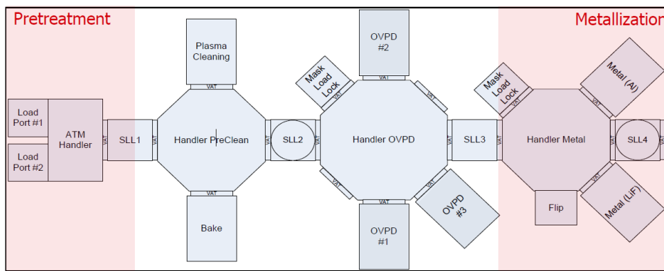
Figure 6.30 Cluster Configuration for OLED Panel Manufacturing Source: Juergen Kreis, Aixtron, OLEDs World Summit, San Diego, CA, 2016 [198]
