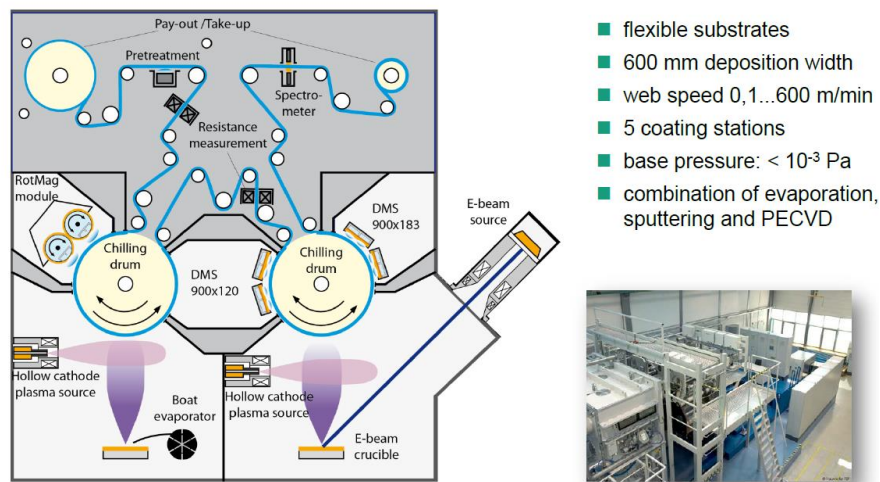
Figure 6.31 Prototype Line used at the Fraunhofer Institute FEP in Dresden
