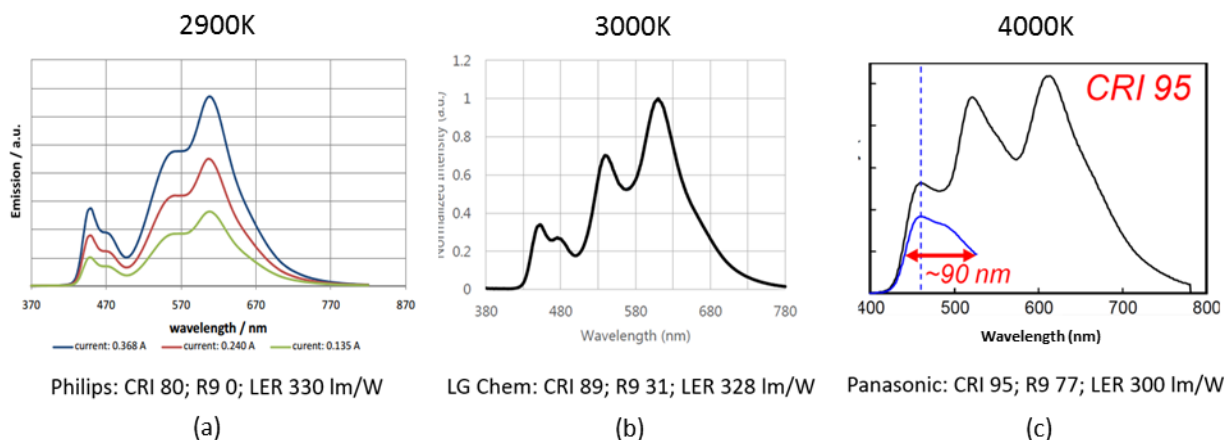
Figure 6.1 Spectra of Commercial and Laboratory OLED Panels
