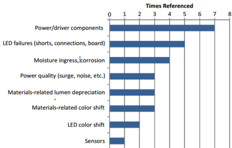
Figure 5.25 The Most Commonly Observed Failures from LSRC Member Survey
