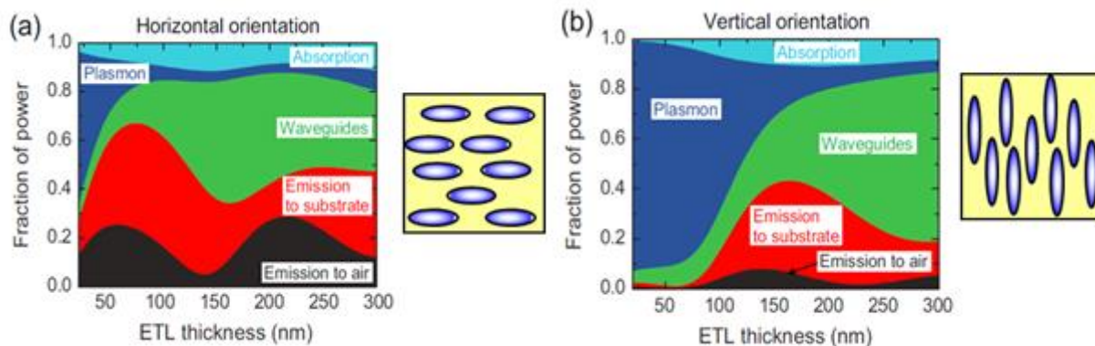
Figure 6.6 (a) Horizontally Oriented Emitters as Compared to (b) Vertically Oriented Emitters Source: B. Scholz et al, Optics Express Journal Entry , 2012 [133]
