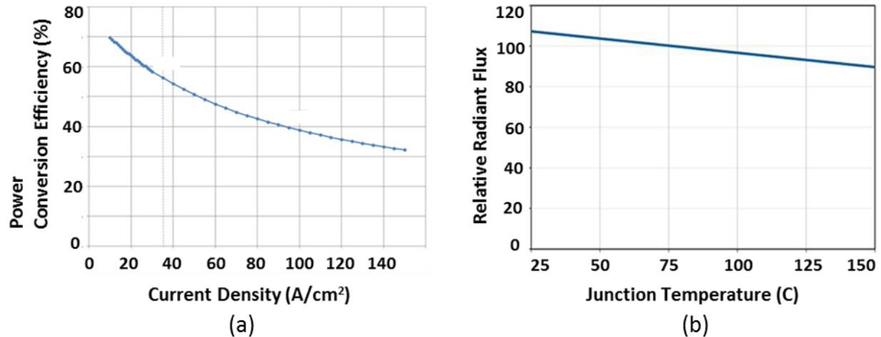
Figure 5.2 Two Types of Efficiency Droop: (a) Current Efficiency Droop, and (b) Thermal Efficiency Droop
