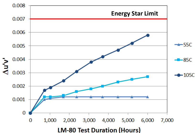
Figure 5.21 Color Shift of LED Package as a Function of Temperature
