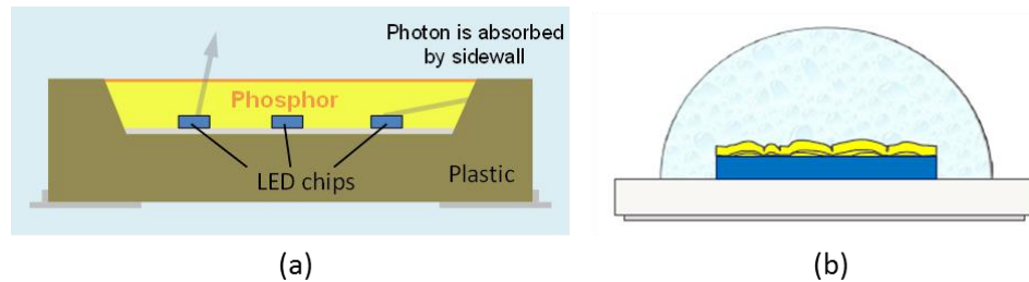
Figure 5.19 LED Package Schematics Showing (a) Sidewall Discoloration and (b) Phosphor Delamination
