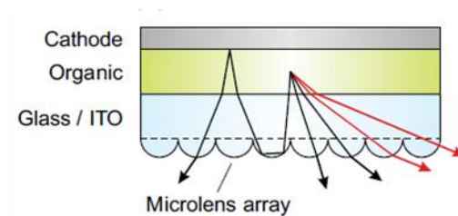
Figure 6.3 External Light Extraction Schematic
