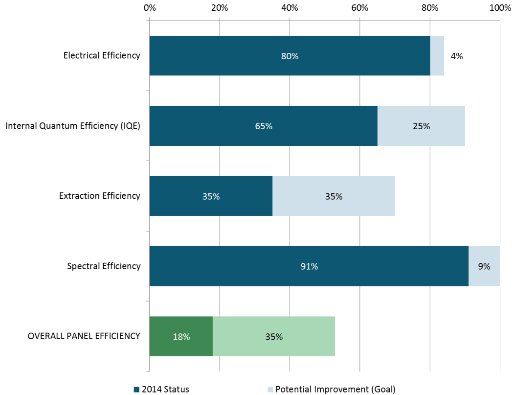
Figure 6.7 OLED Panel Loss Channels and Efficiencies
