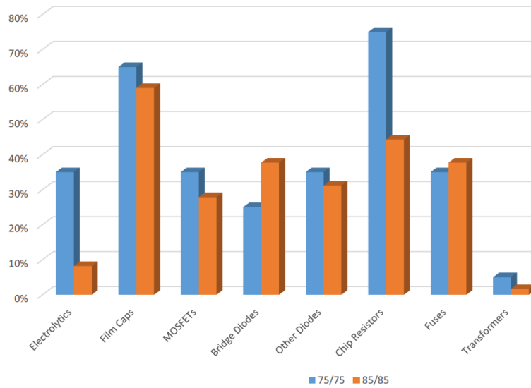
Figure 5.26 A Comparison of Driver Component Failures in 6 in. Downlights After Accelerated Testing at 75°C/75% Relative Humidity (Blue) and 85°C/85% Relative Humidity (Orange)
