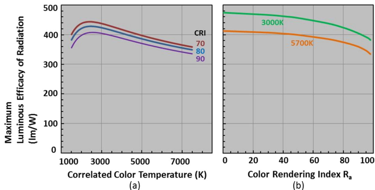
Figure 5.3 Theoretical Limits to White Light Luminous Efficacies of Radiation vs (a) CCT for a Given CRI, and (b) CRI for a Given CCT
