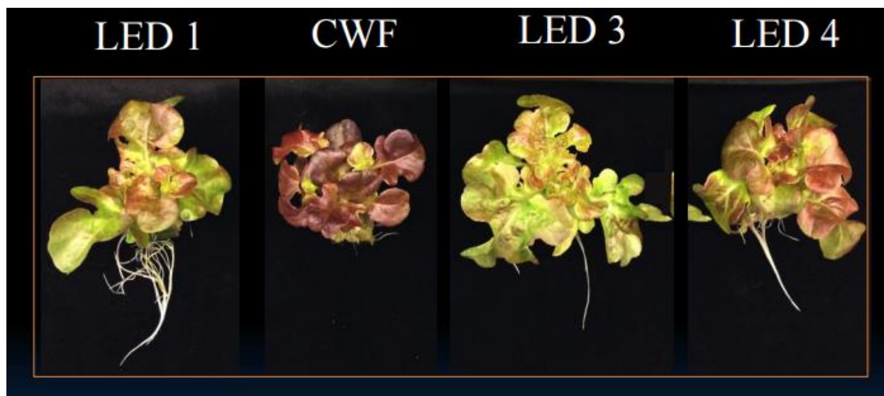
Figure 2.11 The Influence of Spectra on Anthocyanin Production in Red Lettuce
