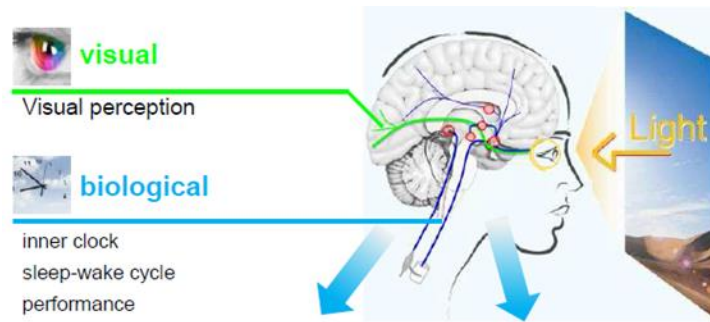
Figure 2.7 How Light Affects a Biological Systems
