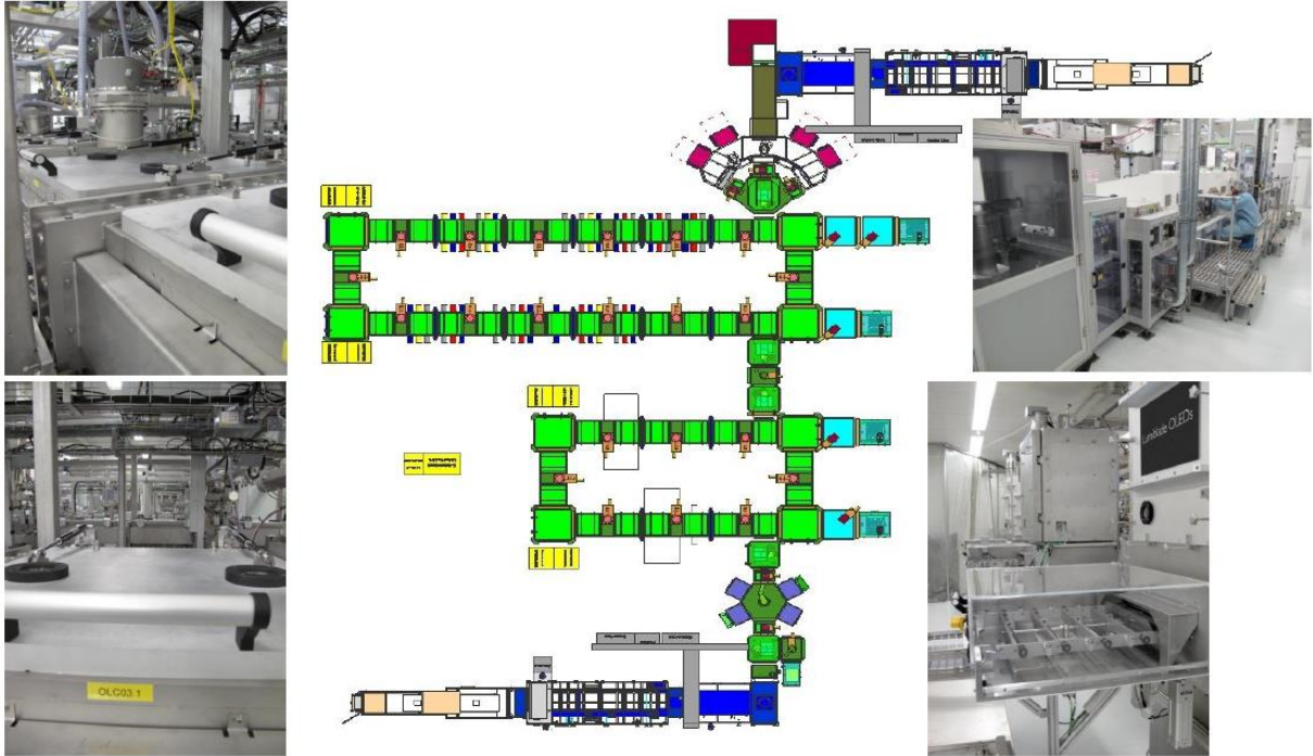
Figure 6.29 OLED Panel Production Line in Aachen, Germany Source: U. Hoffman, China International OLED Summit, Beijing, 2015 [161]
