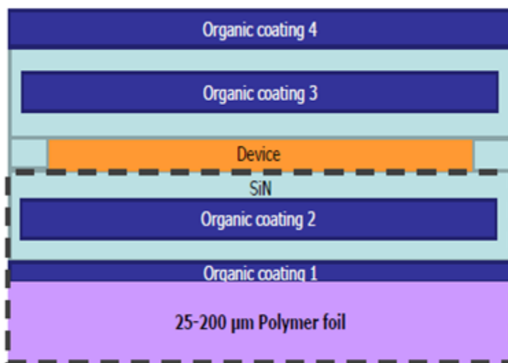
Figure 6.22 Multi-Layer Barrier Coating to Prevent Ingress of Moisture and Oxygen
