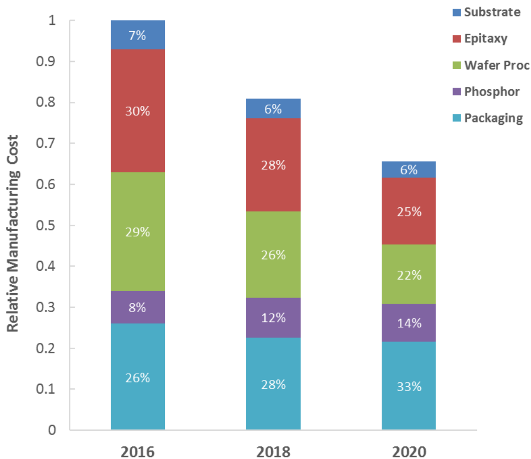
Figure 5.14 Projected High Power LED Package Cost Reduction Source: Inputs from DOE SSL Roundtable and Workshop attendees
