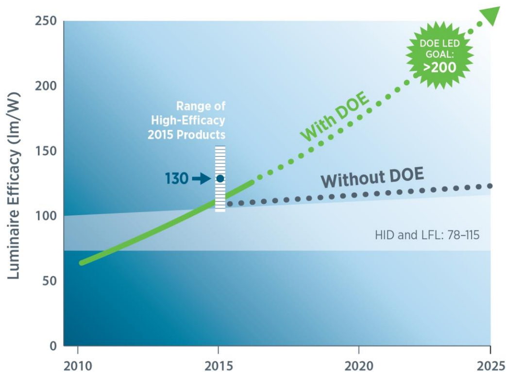
Figure 2.1 Comparison of LED and Incumbent Light Source Efficacies
