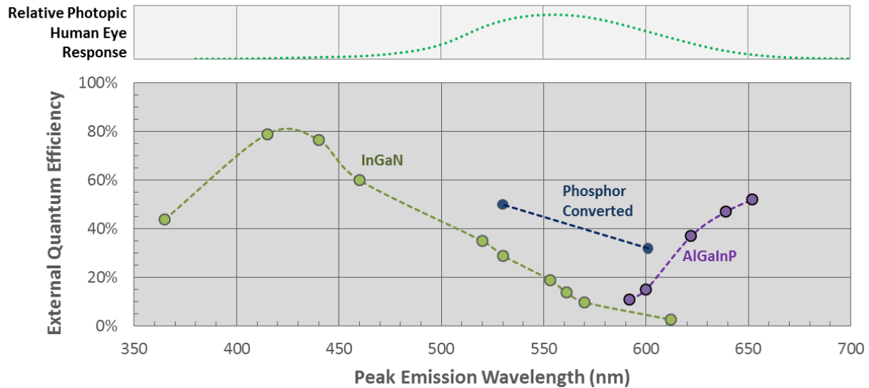
Figure 5.7 (Top) Photopic Human Eye Response vs Wavelength, and (Bottom) External Quantum Efficiencies of “Best Research” LEDs vs Wavelength.
