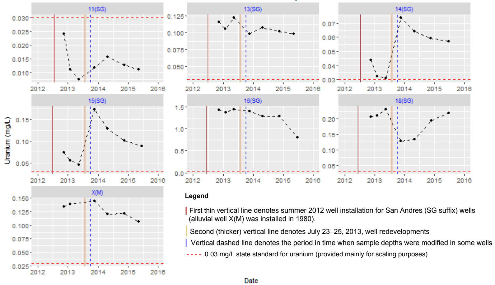
Figure C-1. Time-Concentration Plots of Uranium in Bluewater Disposal Site Wells Wells Redeveloped July 23–25, 2013
