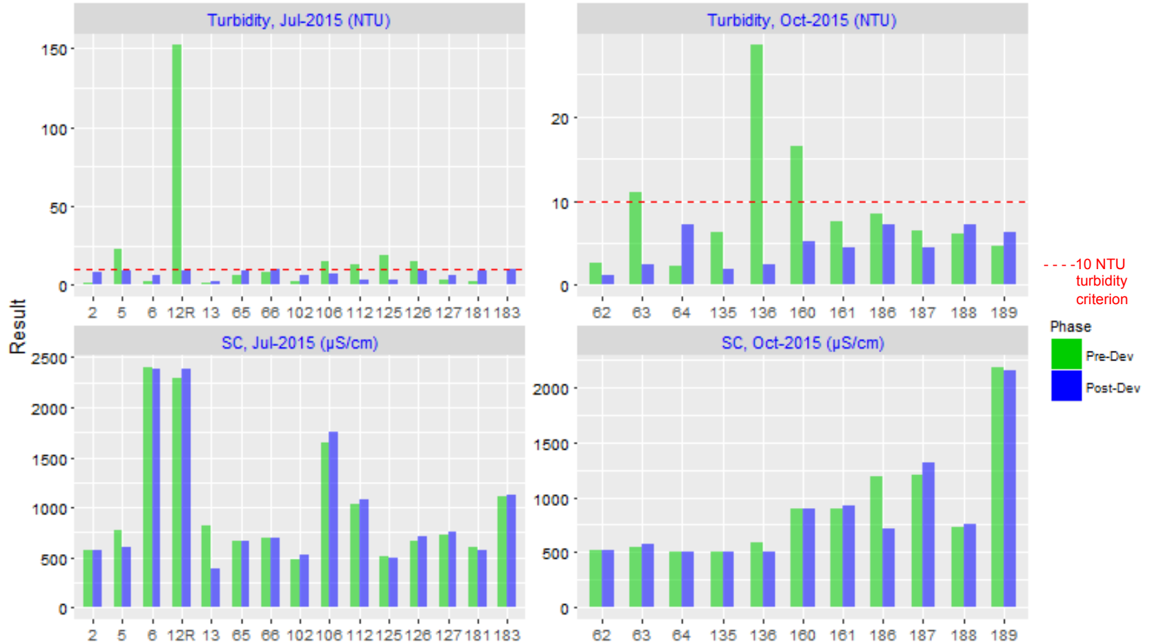
Figure 31. Bar Charts of Pre- and Post-Redevelopment Turbidity and SC in Gunnison Processing Site Wells
