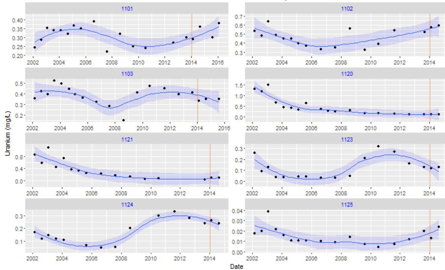
Figure C-10. Time-Concentration Plots of Uranium in Tuba City Disposal Site Extraction Wells page 2 of 4
