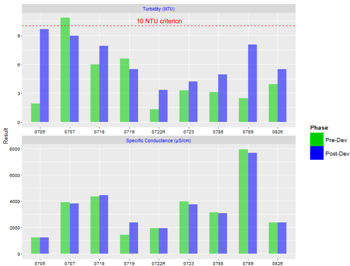
Figure 36. Pre- and Post-Redevelopment Turbidity and SC in Riverton Site Redeveloped Wells
