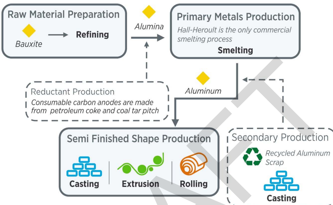
Figure 2-1. Aluminum Manufacturing Process Flow Diagram
