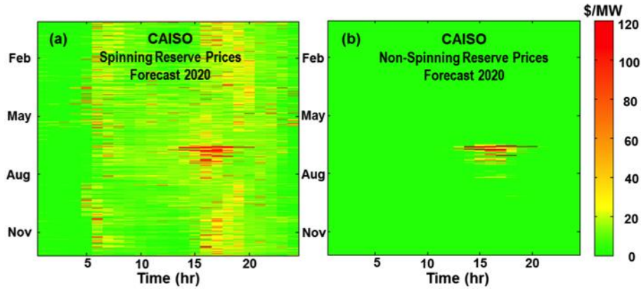
Figure 2.8. Spinning and non-spinning reserve price ($/MW) forecast for CAISO market in 2020. Spinning reserve prices closely resemble load following up and regulation up prices.
