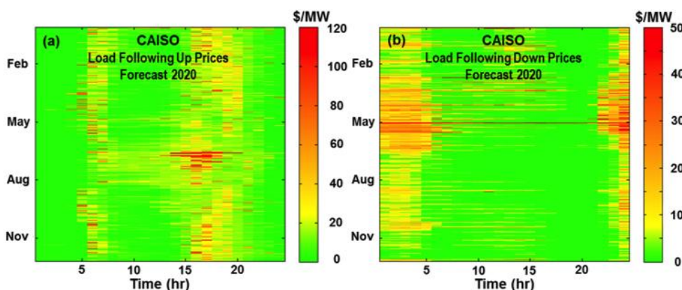
Figure 2.6. Load following up and down ancillary service price ($/MW) forecast for CAISO market in 2020. Load following up prices exceed $100/MWh during ramp ups to meet the morning and evening peak loads. Load following down prices exceed $40/MWh when load is falling in the late evening and early morning hours. Note the different color scales indicating that load following down prices are less than half of the load following up prices.
