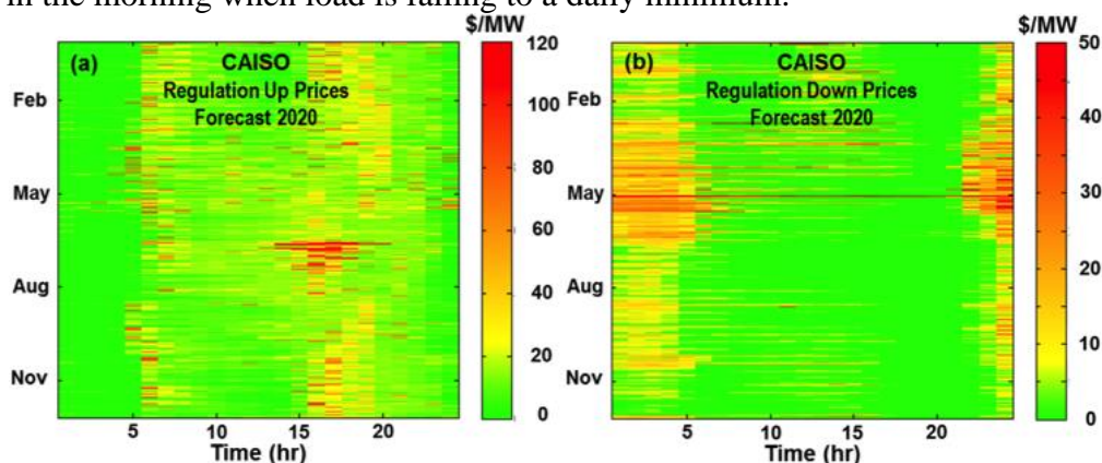
Figure 2.7. Regulation up and down ancillary services price ($/MW) forecast for CAISO market in 2020. Regulation prices follow the same general patterns as load following service prices.
