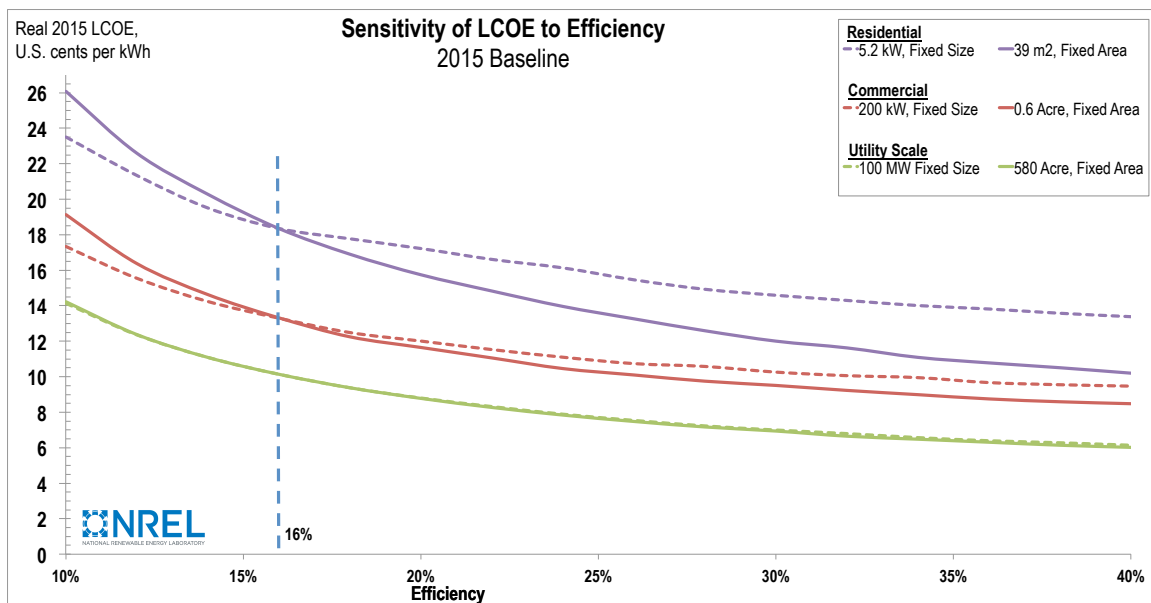
Figure 6. Efficiency versus 2015 real LCOE for fixed size and fixed area PV systems, without ITC. The systems costs used are shown in Figure 5.
