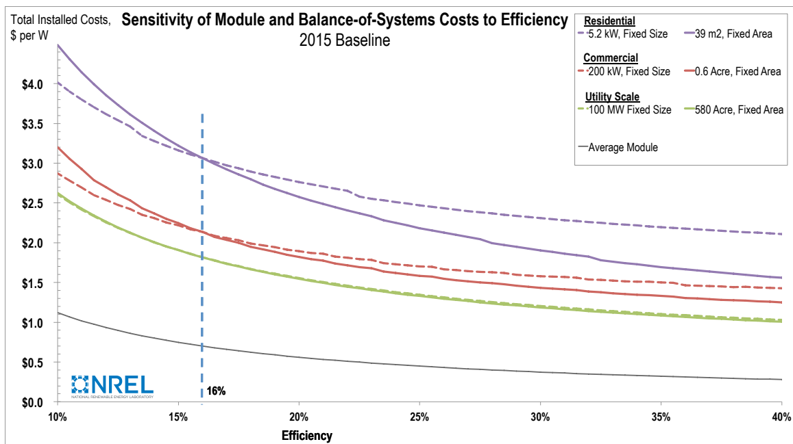
Figure 5. Dollars-per-Watt sensitivity of module and systems costs to changes in efficiency. The module price represented is for multicrystalline silicon. Systems costs are shown for fixed area and fixed size systems for representative residential, commercial and utility-scale systems. The kinks in the residential and commercial lines represent step changes in cost due to changes in inverter price points. A vertical line is shown at the 2015 benchmark module efficiency of 16%.
