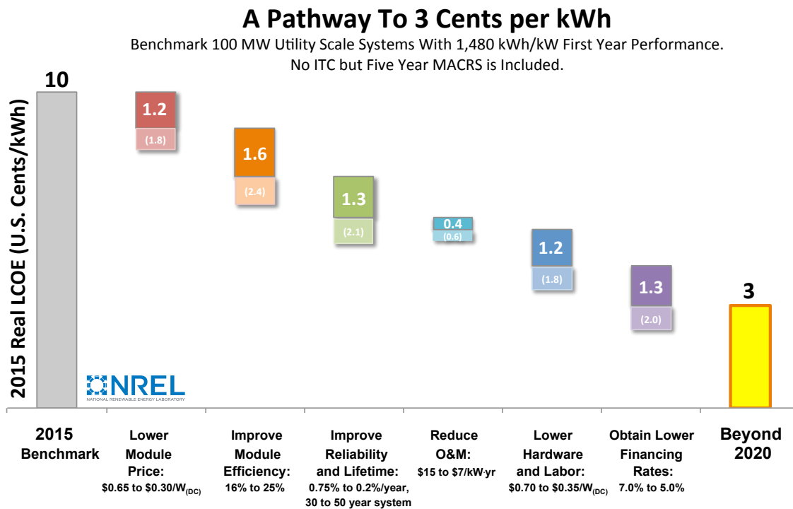
Figure 9. Progress toward an LCOE target of 3 cents per kWh for 100 MW utility scale systems with 1,480 kWh/kW first-year performance. See the note on interdependencies in Figure 8, and also note that reductions in operations and maintenance (O&M) expenses are called upon.
