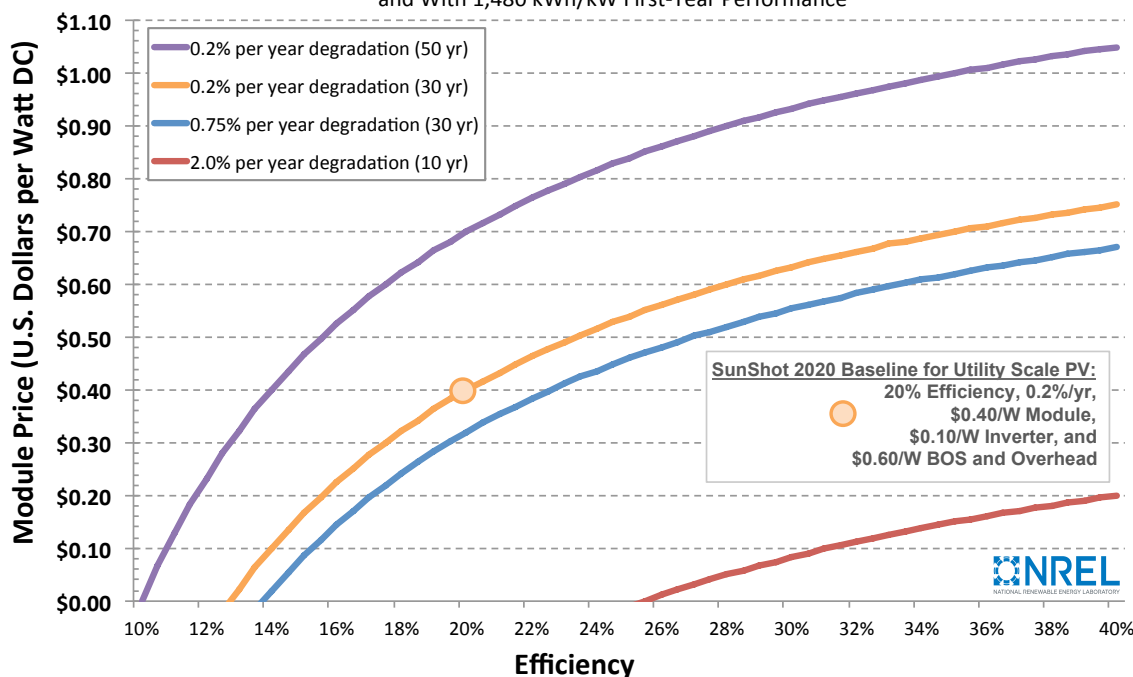
Figure 2. Permutations of the key metrics of module price, efficiency, degradation rate, and system lifetime that could reach the utility scale SunShot target of 6 cents per kWh with energy yield around 1,480 kWh/kW. The inverter, balance-of-systems, and overhead contributions are held constant at $140/m 2 , which corresponds $0.70/W at 20% efficiency, and which is a 35% reduction from 2015 costs. Thus, some concurrent innovation in the non-module components is also assumed. The SunShot baseline case described in the text is shown as an orange circle. Impacts due to changes in the discount rate are not included within this particular figure but are shown later (in Figure 7).
