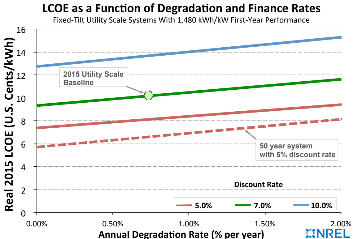
Figure 7. Lifetime, degradation rate, and financing impacts upon LCOE for 2015 residential (top—Figure 7a) and fixed-tilt utility scale systems (bottom—Figure 7b) in Kansas City without any ITC. With the exception of the bottommost curves, 30-year system lifetimes are used.
