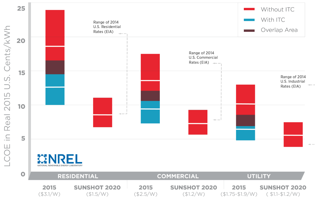
Figure 1. LCOE calculations using baseline 2015 and SunShot 2020 systems costs. A 30% federal ITC is included in the 2015 “With ITC” cases. The other assumptions are detailed in Table 1. The white lines indicate the LCOE results for Kansas City, Missouri. The bottom of each red or blue bar corresponds to the LCOE value calculated for Daggett, while the top of each bar corresponds to the LCOE values calculated for Seattle. The utility scale cases range from fixed-tilt in Seattle (upper end) to one-axis tracking in Daggett (lower end). EIA data for the 2014 range of average residential, commercial, and industrial electricity rates across the continental United States is also shown [8]
