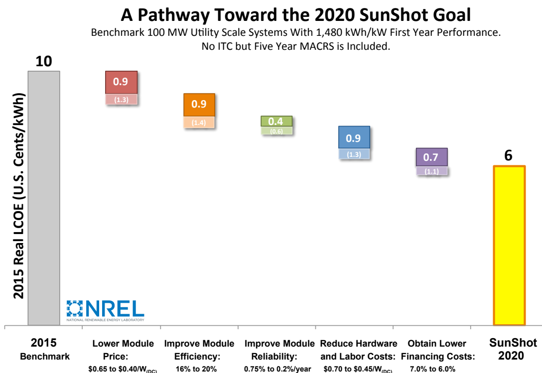
Figure 8. Progress toward the SunShot 2020 goal for 100 MW utility scale systems with 1,480 kWh/kW first-year performance.
