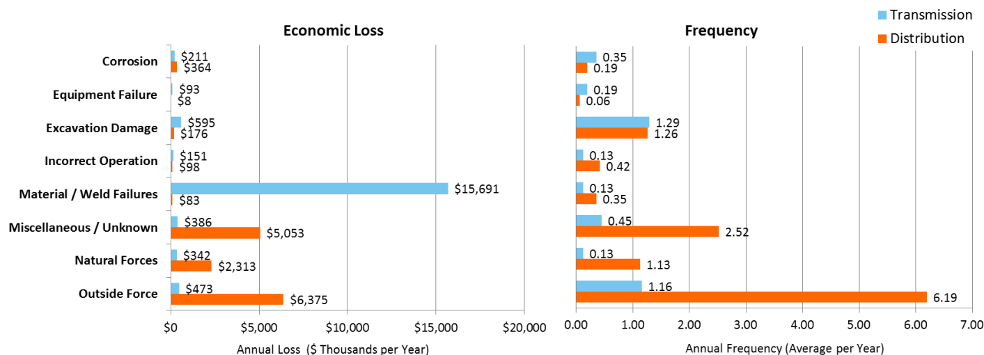
Top Events Affecting Natural Gas Transmission and Distribution in California (1986–2014)
