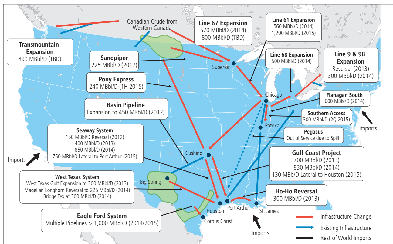
Figure 4-2. Highlighted Pipeline Reversals and Expansions Accommodating Increased Domestic and Canadian Supply 7
