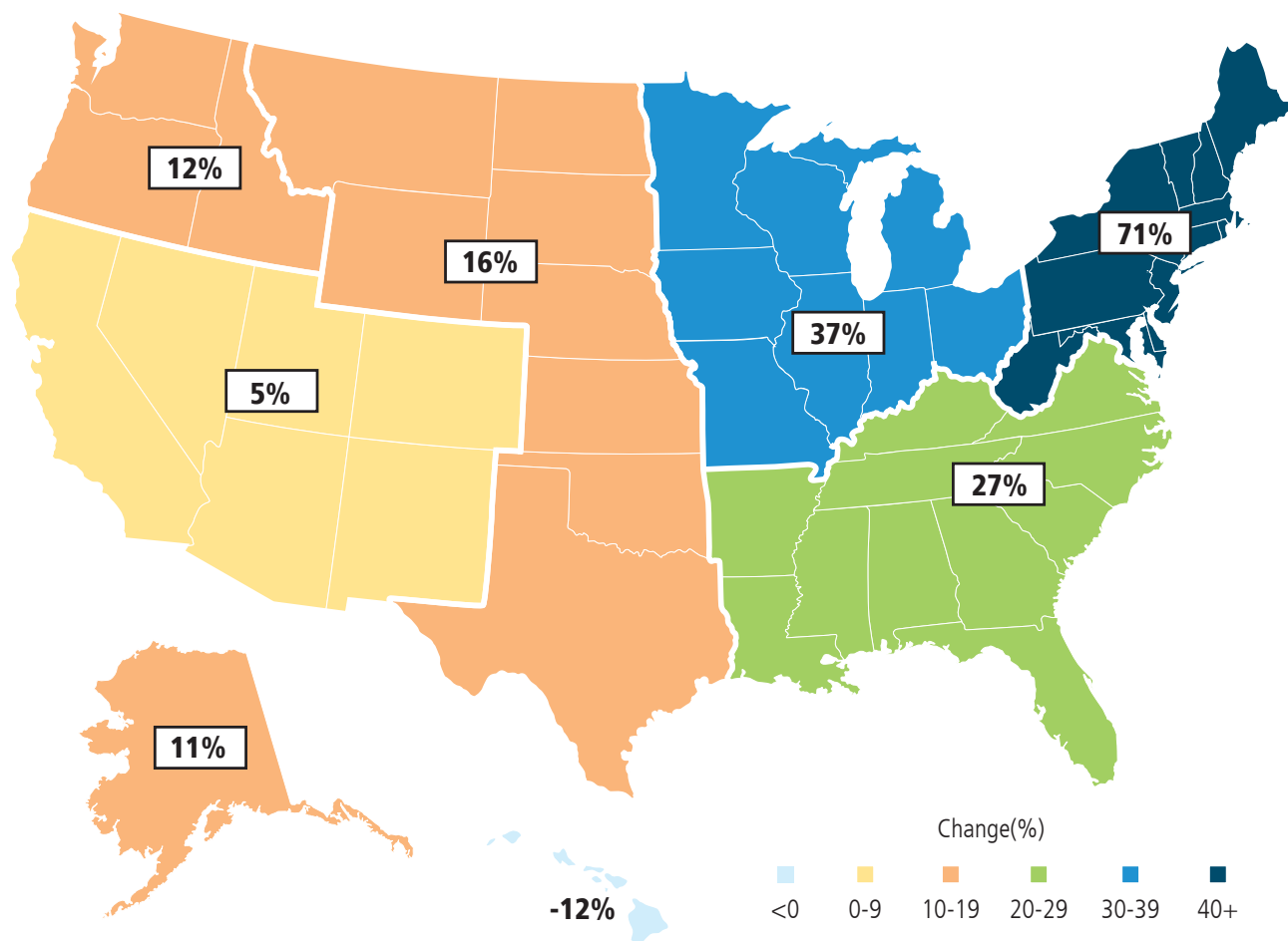
Figure 1-6. Observed Change in Very Heavy Precipitation 67
