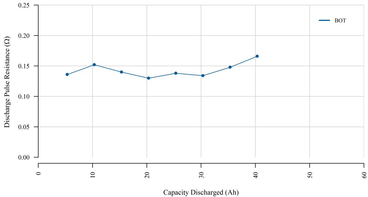
Figure 3. Thirty-second discharge pulse resistance versus capacity discharged
