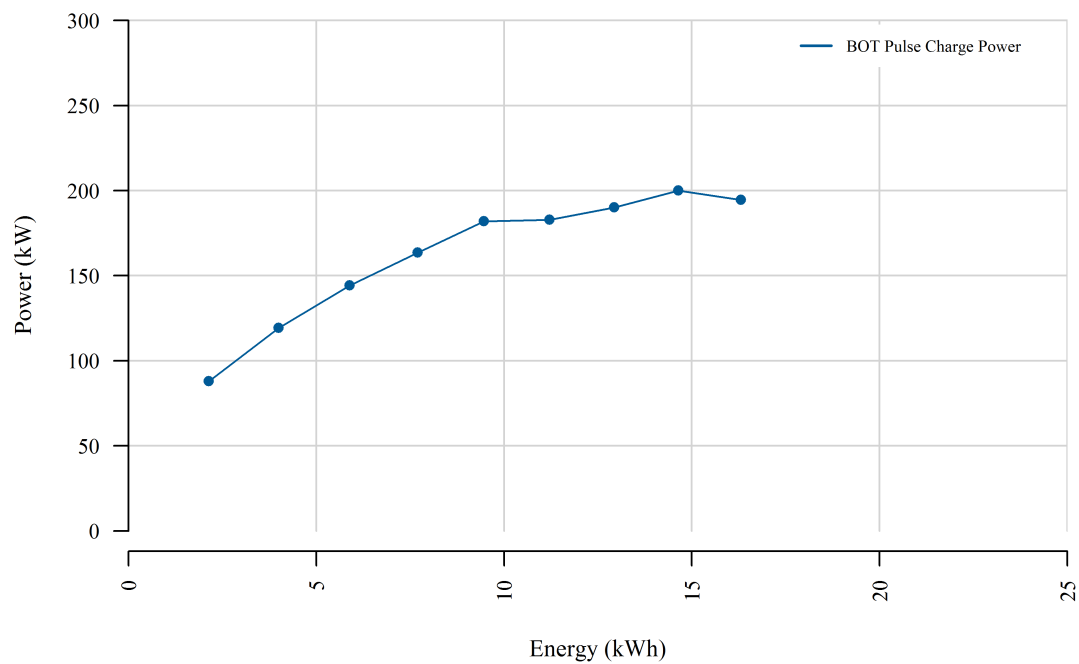
Figure 4. Charge power capability versus energy discharged
