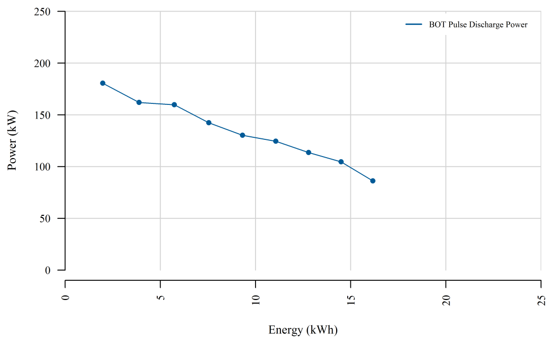
Figure 5. Discharge power capability versus energy discharged
