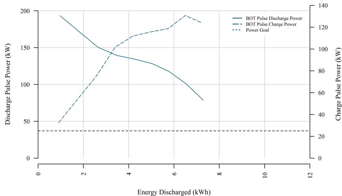
Figure 4. Discharge and charge power capability versus energy discharged
