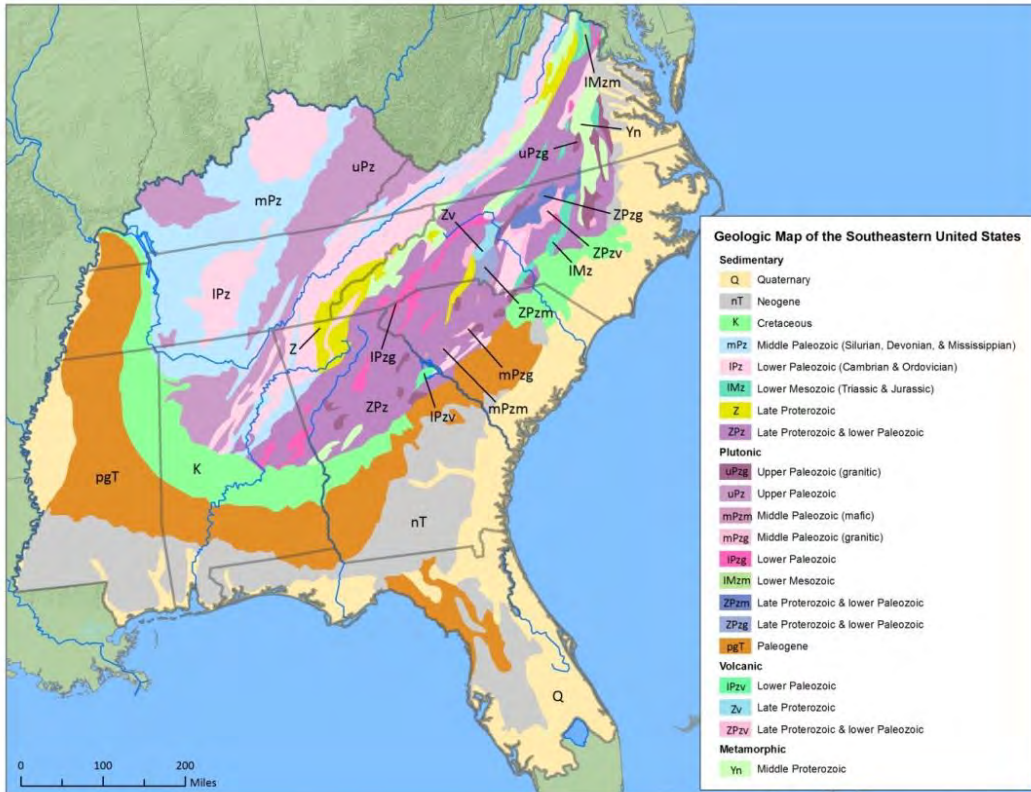
Figure 3.4-4: Generalized Geology of the Project Area
