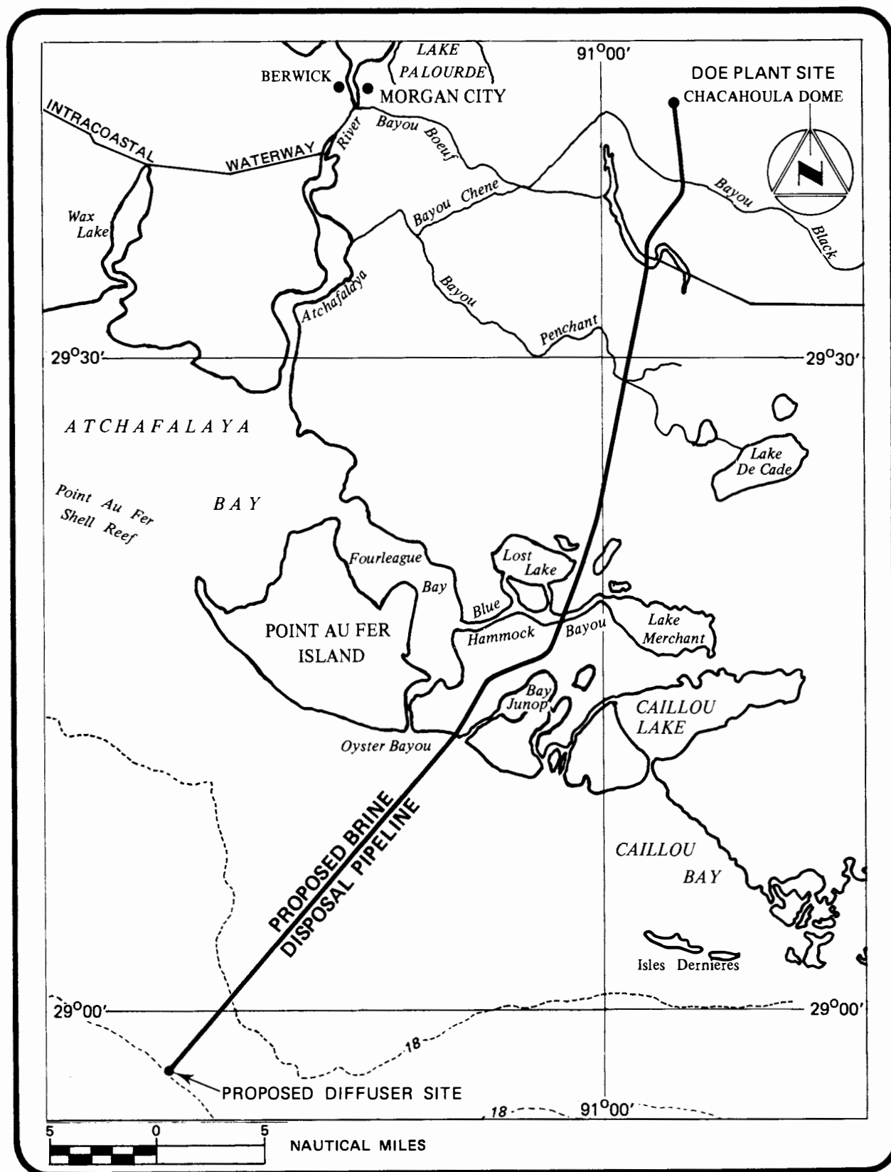
FIGURE A.7-5 Brine disposal pipeline route - Chacahoula dome.
