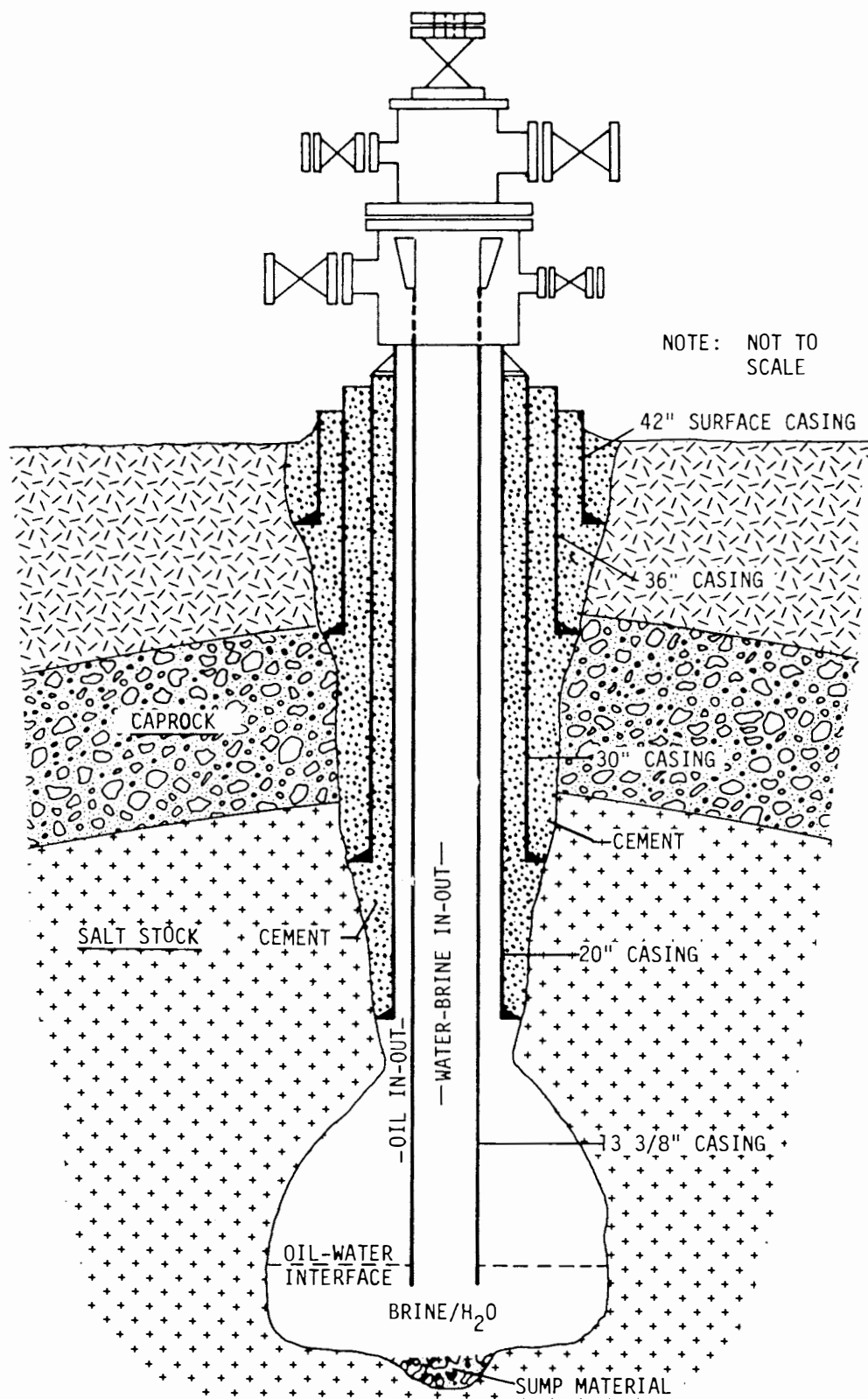
FIGURE A.3-2 Typical storage well casing diagram.
