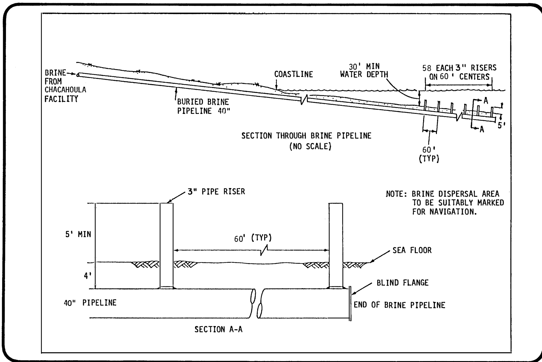
FIGURE A.7-6 Brine dispersal system - Chacahoula dome.
