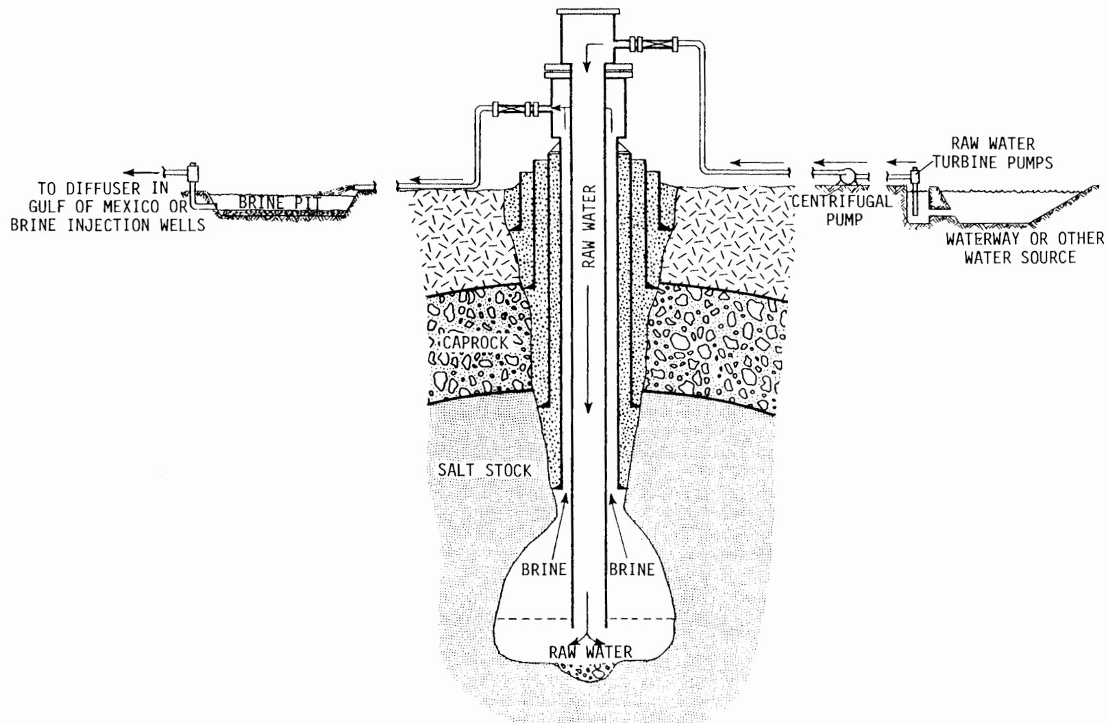
FIGURE A.2-1 Representation of solution mining cycle
