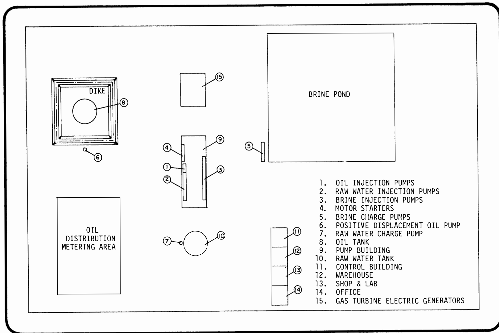
FIGURE A.6-9 Storage area layout - Iberia dome.
