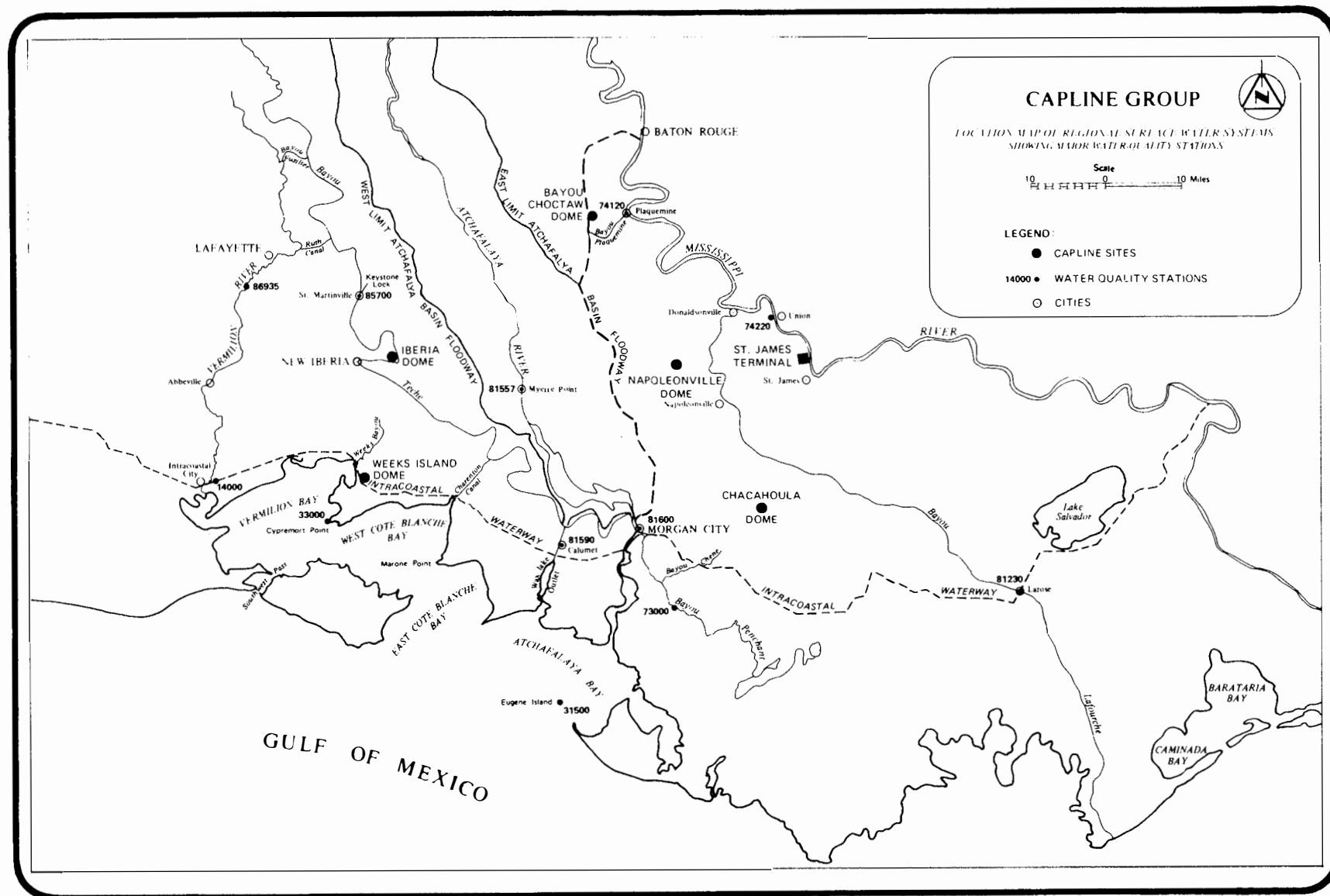
FIGURE 3.2-4 Capline Group location map of regional surface water systems showing major water quality status.
