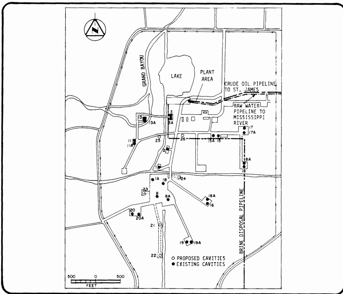
FIGURE 2.5-2 Vicinity and site map - Bayou Choctaw dome.
