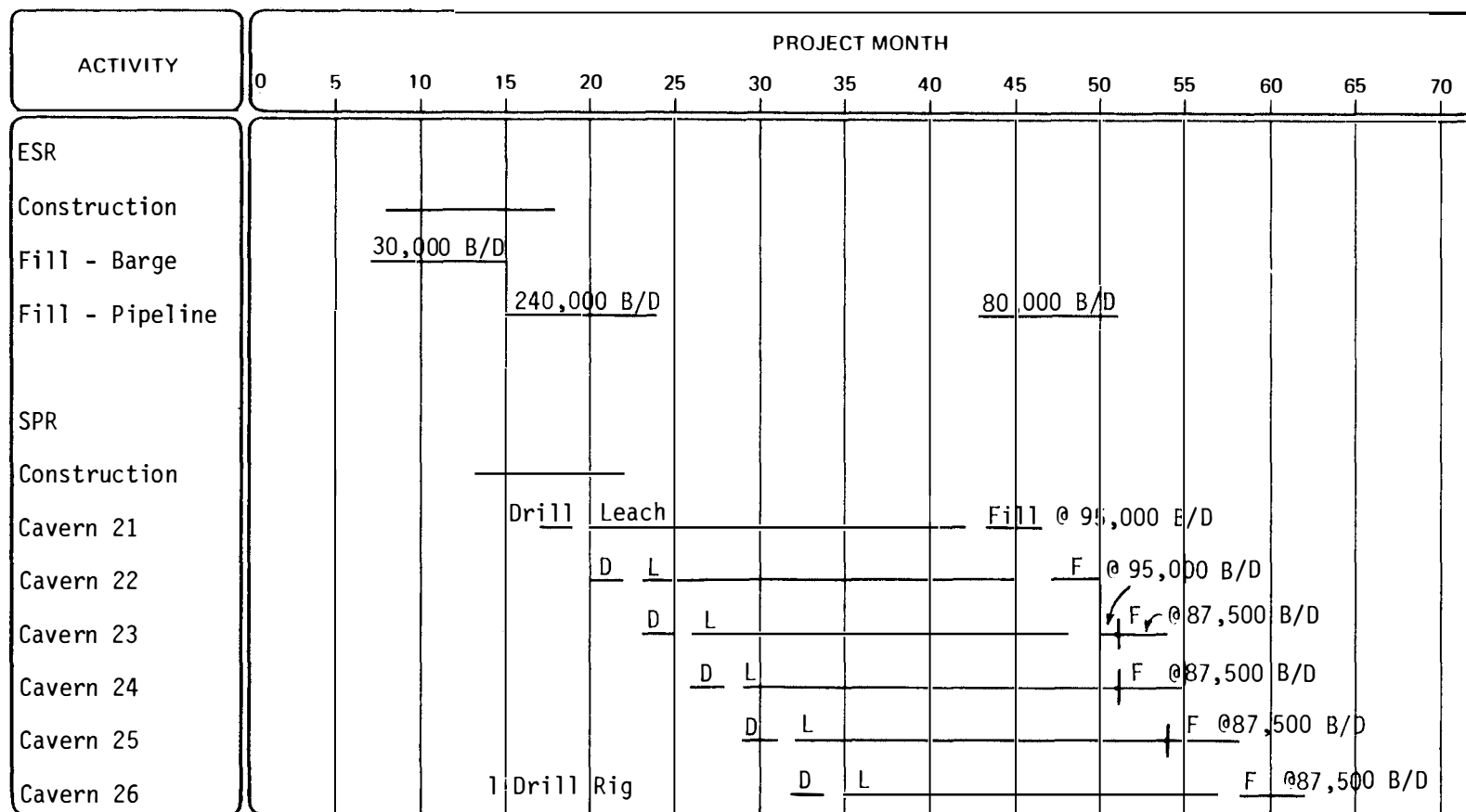
FIGURE 2.5-3 Development timetable for Bayou Choctaw dome.
