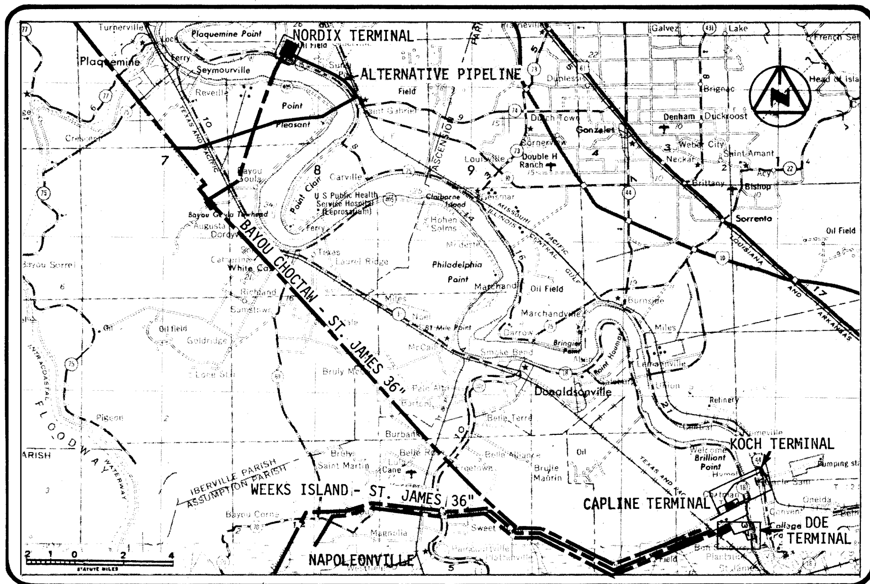
FIGURE 2.3-2 Capline Group oil distribution terminal facilities.
