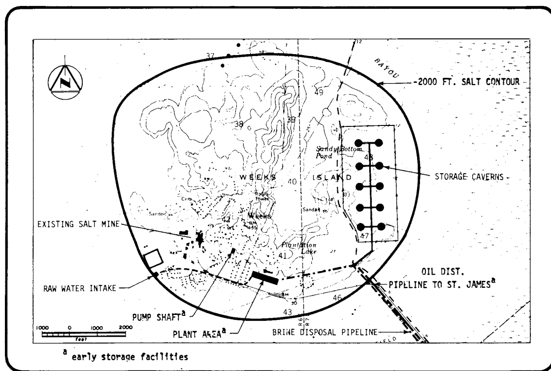
FIGURE 2.4-2 Vicinity and site map - Weeks Island dome.
