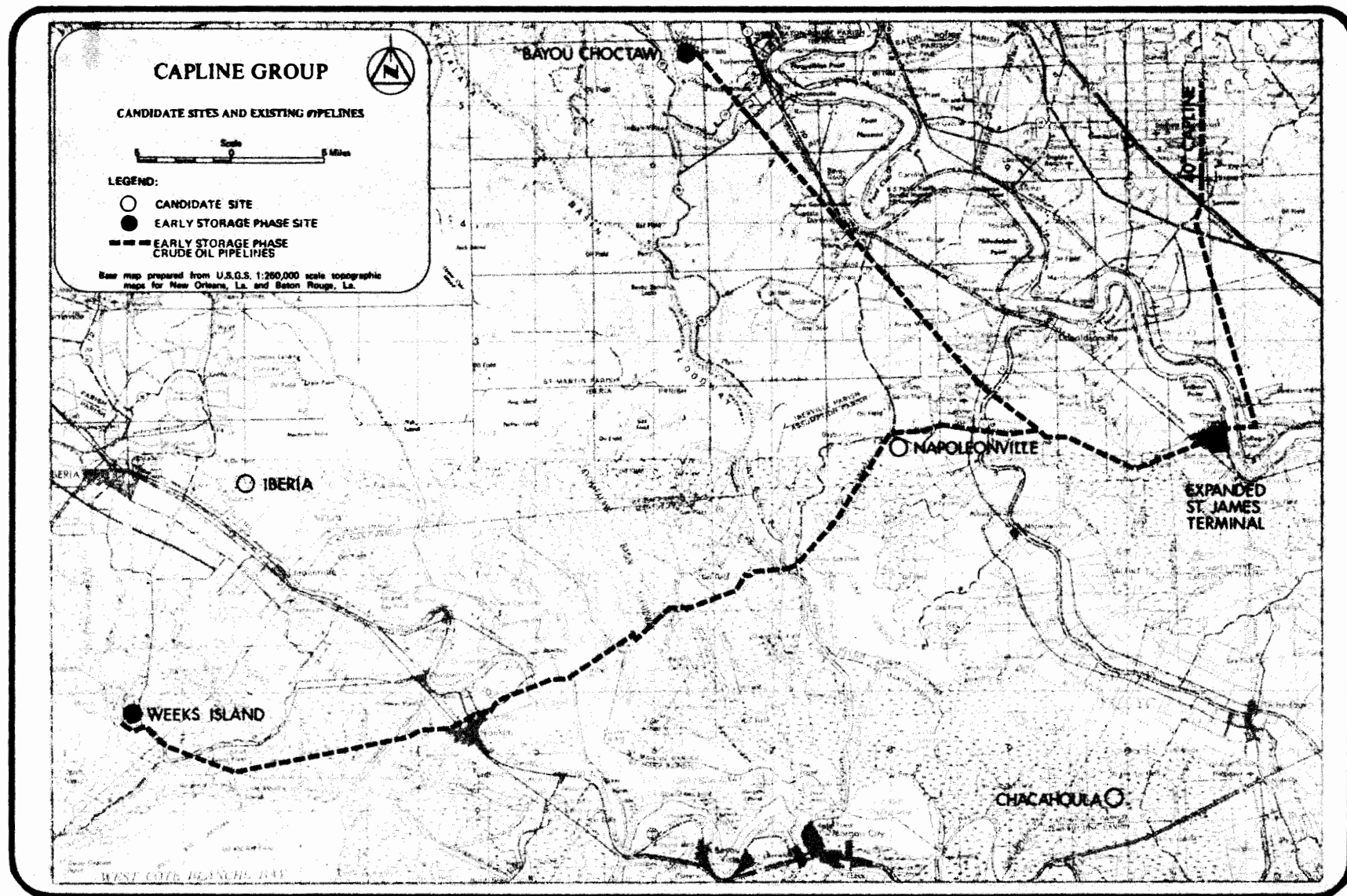
FIGURE 2.1-1 Capline Group - alternative sites and existing pipelines.
