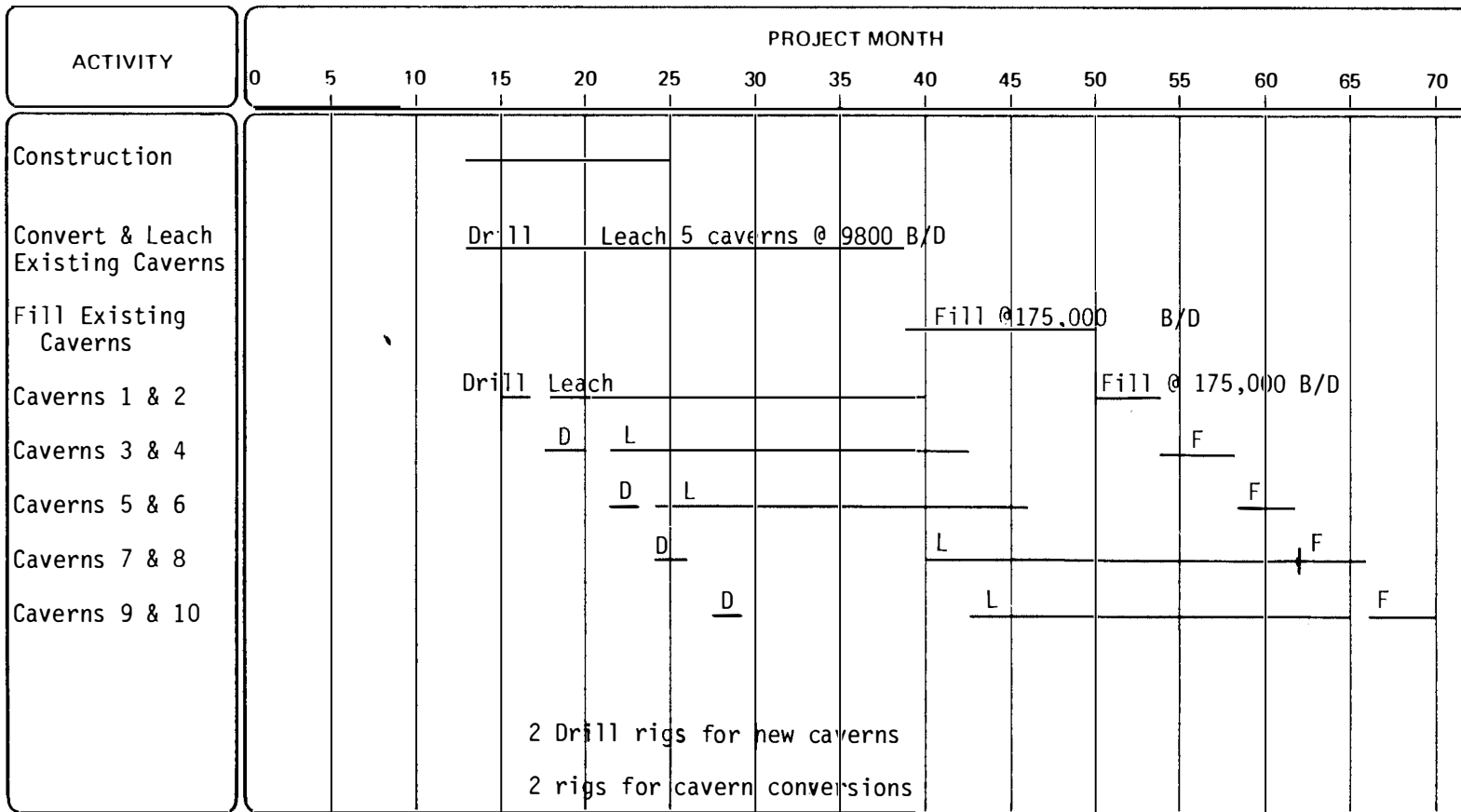
FIGURE 2.3-4 Development timetable - Napoleonville.
