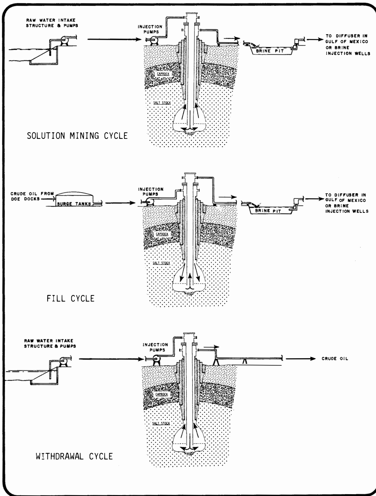
FIGURE 2.2-1 Schematic representation of SPR facility operation
