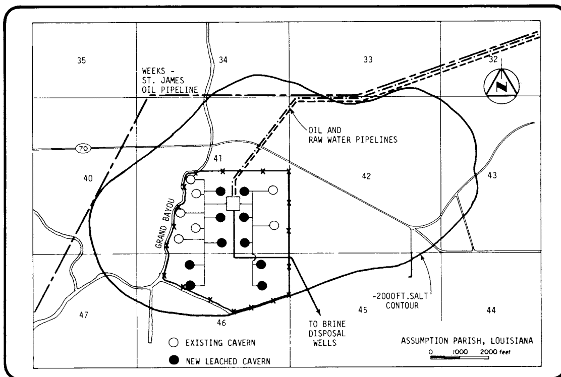
FIGURE 2.3-3 Vicinity and site map - Napoleonville dome.
