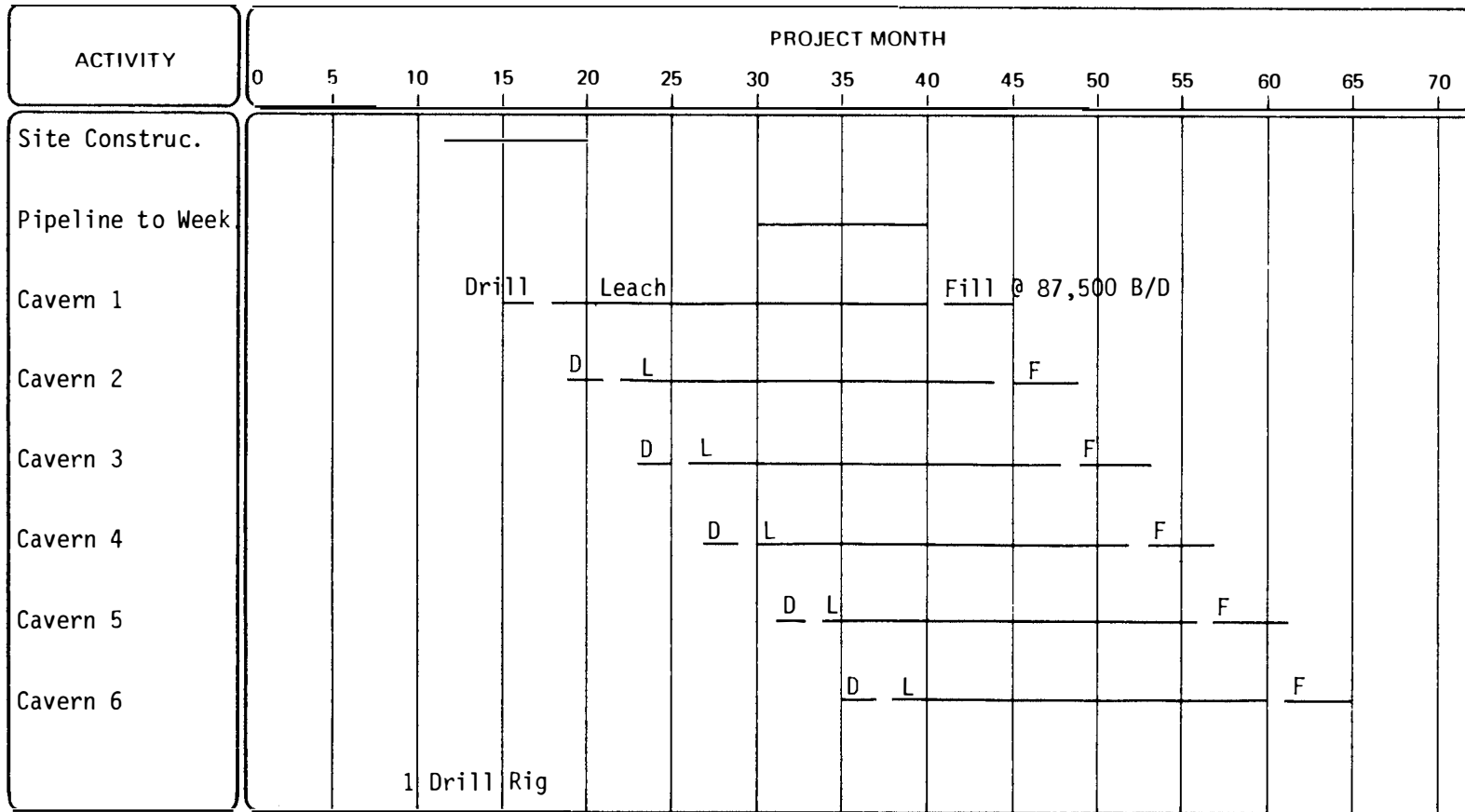
FIGURE 2.5-5 Development timetable for Iberia dome.
