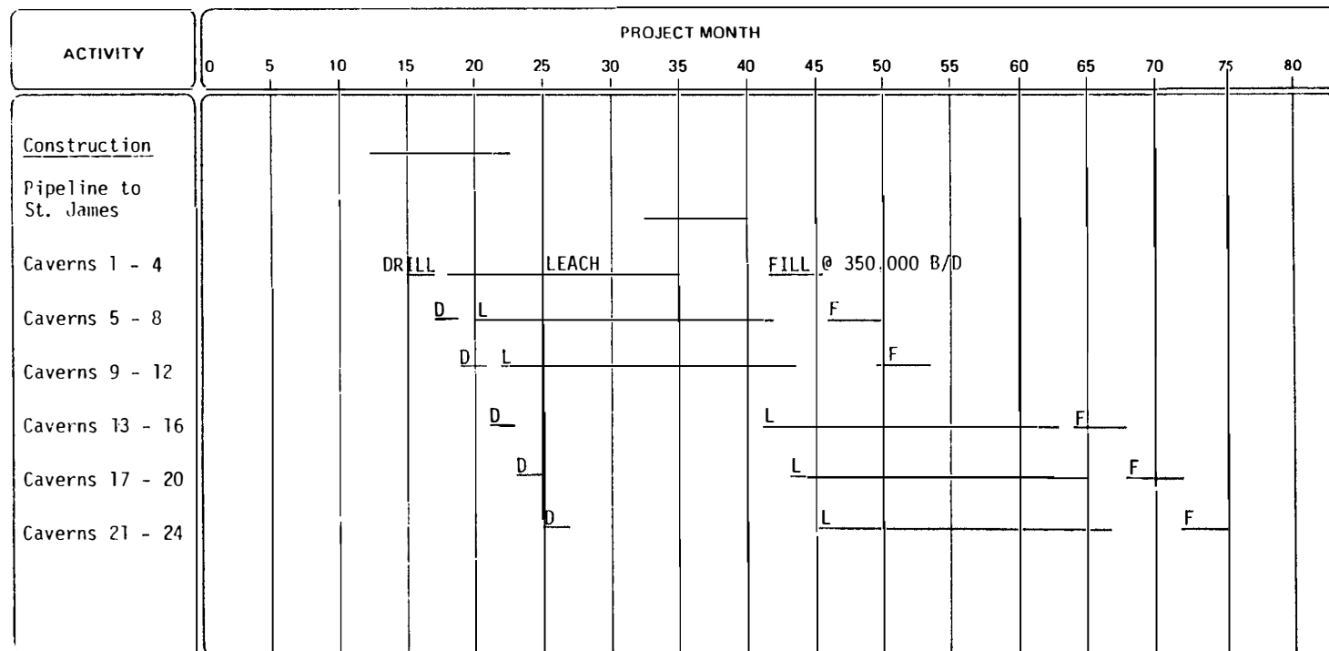
FIGURE 2.6-3 Development timetable for Chacahoula dome.
