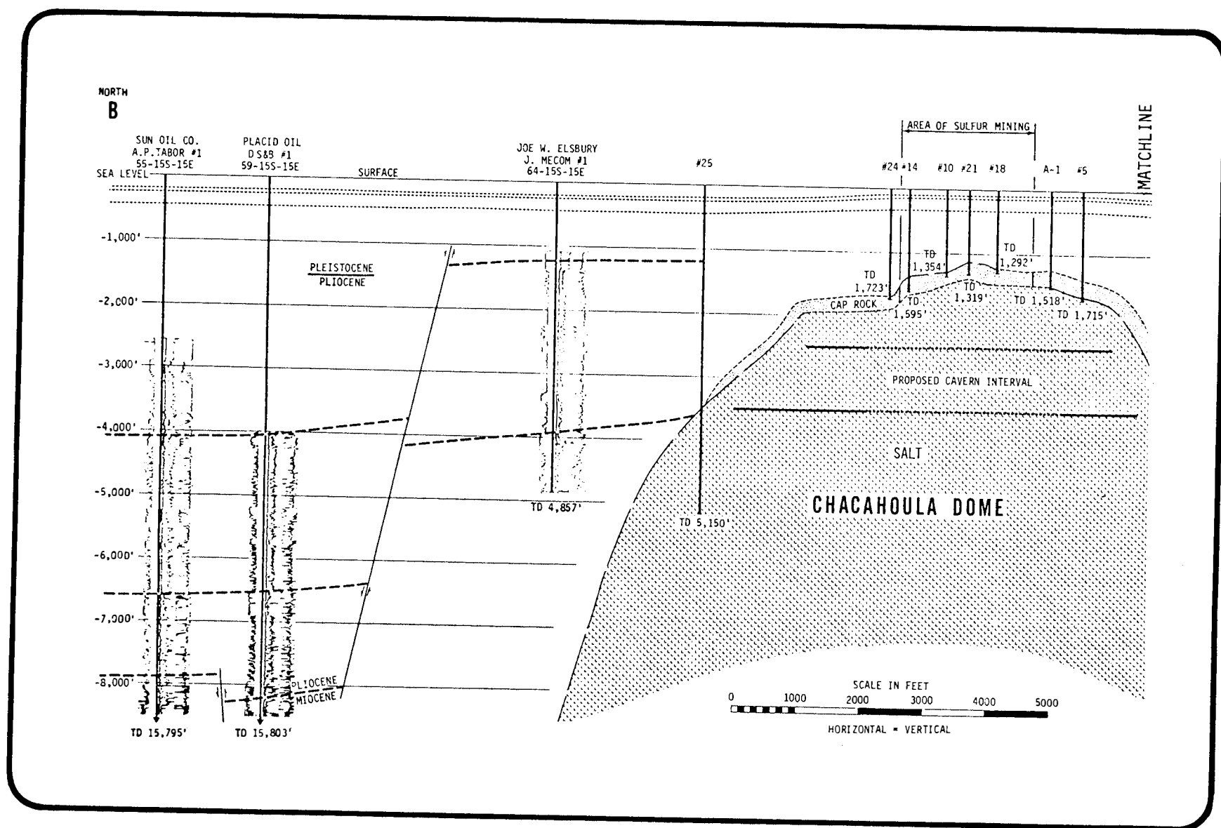
FIGURE 3.6-1 Geologic cross section (north/south) Chacahoula dome.
