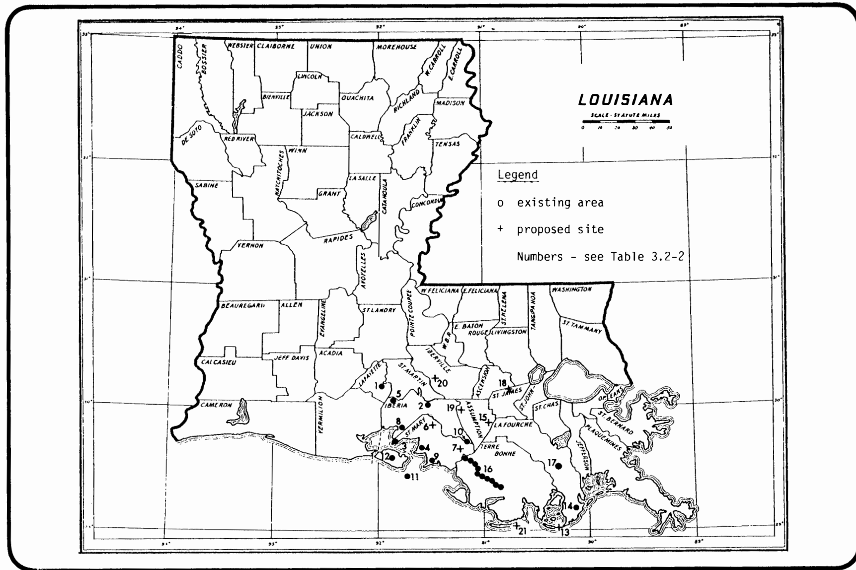
FIGURE 3.2-5 Existing and potential recreation and wildlife areas.
