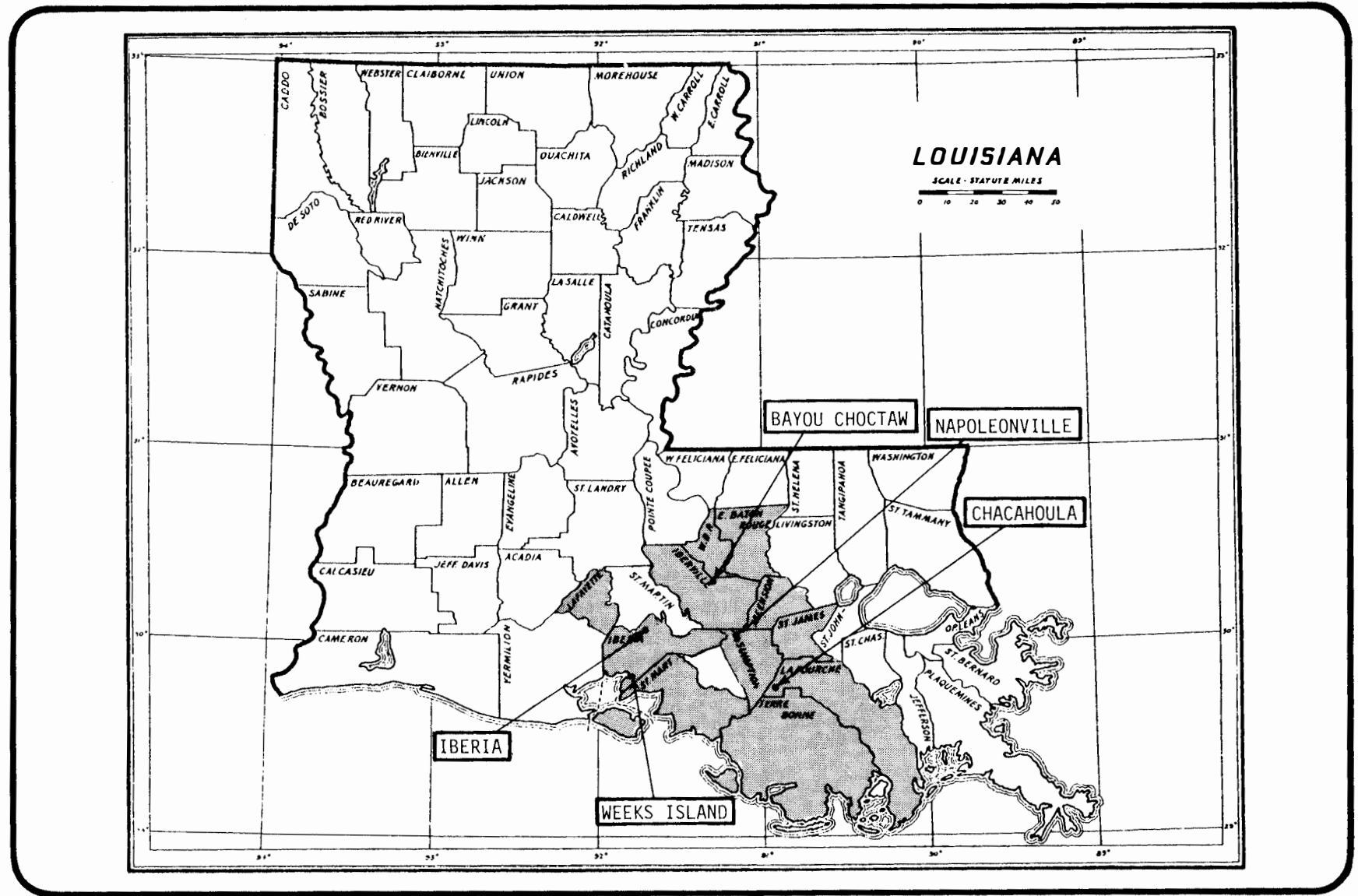
FIGURE 3.2-6 SPR sites and socioeconomic region.
