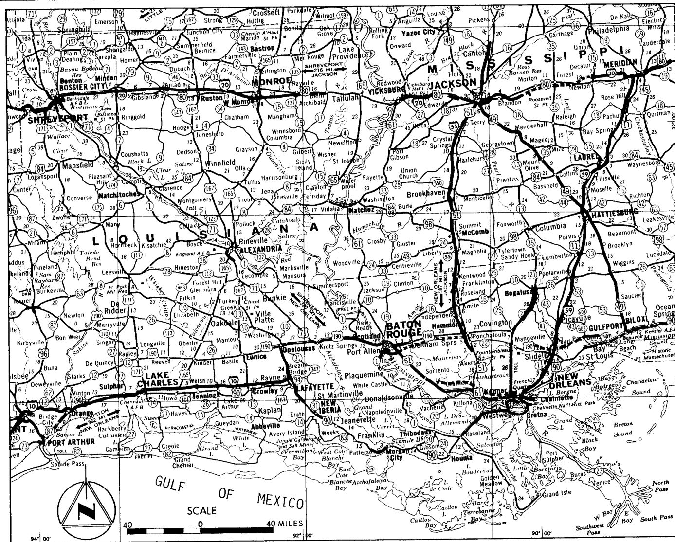
FIGURE 3.2-7 Regional highway network.
