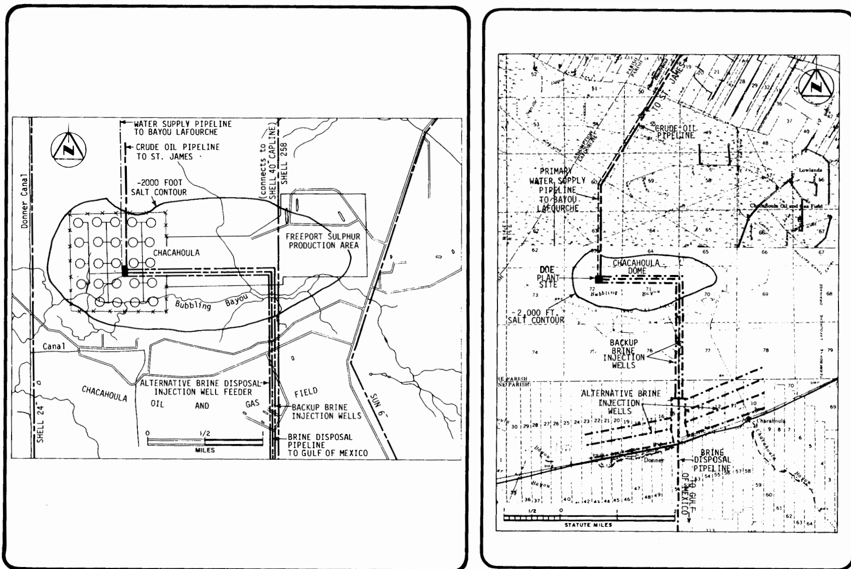
FIGURE 2.6-2 Vicinity and site map - Chacahoula dome.
