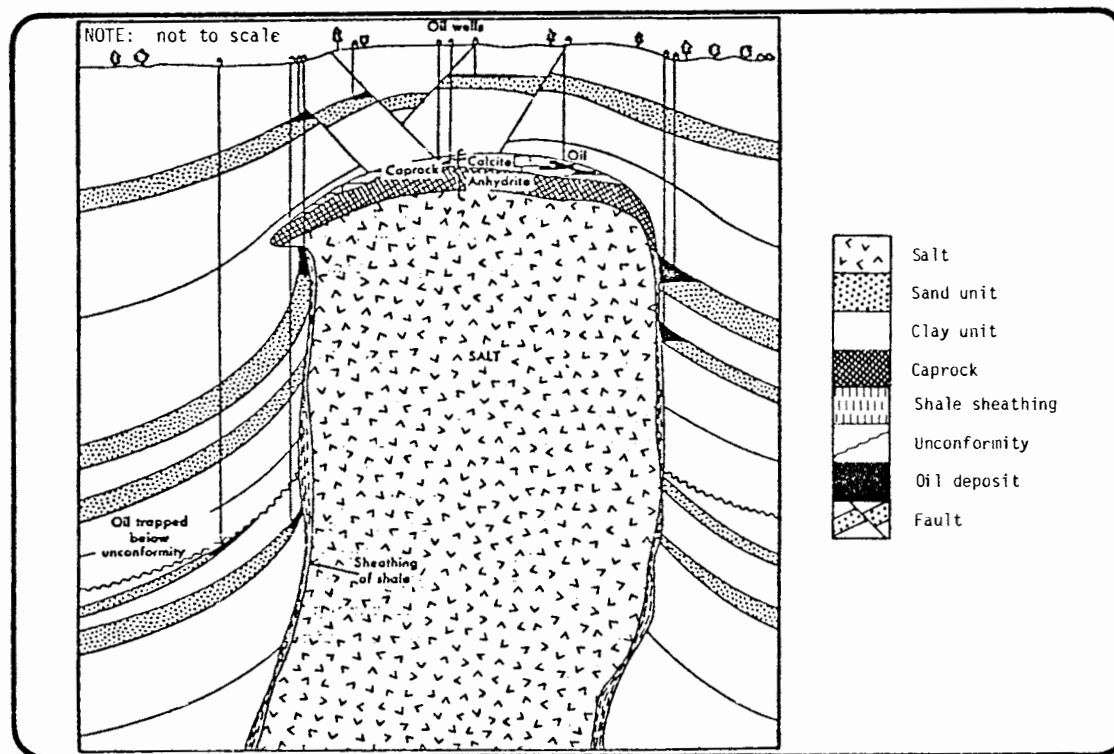
FIGURE 3.2-2 Regional geologic cross section (top); typical salt dome structure (bottom).
