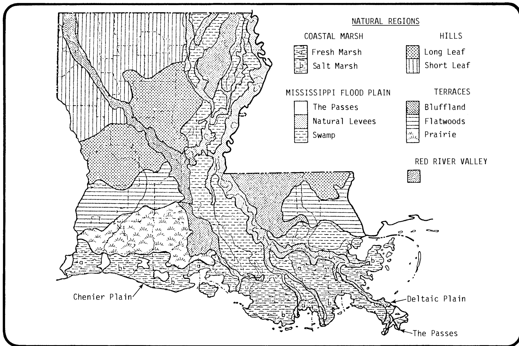
FIGURE 3.2-1 Natural regions of the state of Louisiana.
