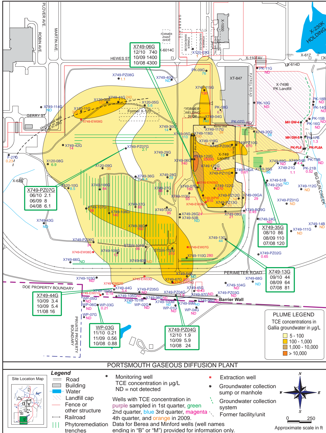
Figure 6.2. Trichloroethene-contaminated Gallia groundwater plume at the X-749/X-120/PK Landfill – 2010.
