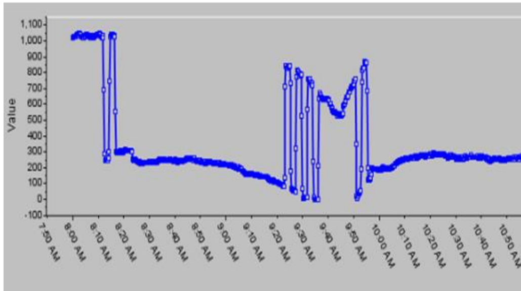
Figure 7. Water Flow Stabilized After 2 Hours at 300gpm
