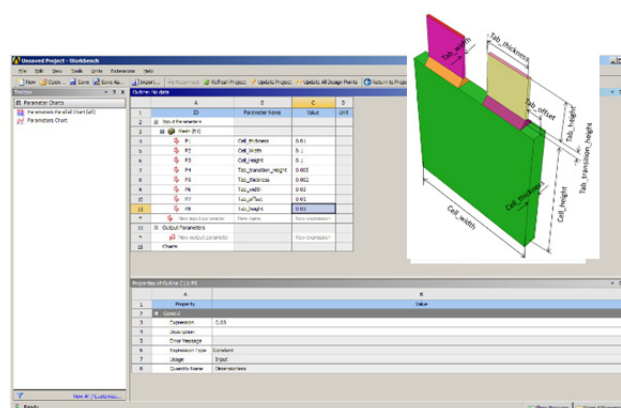
Figure IV - 78: Set cell geometry based on parameterized templates
