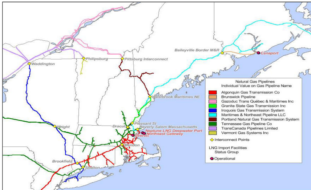
Figure 3. Interstate and importing gas pipelines of New England (Source: ISO New England)
