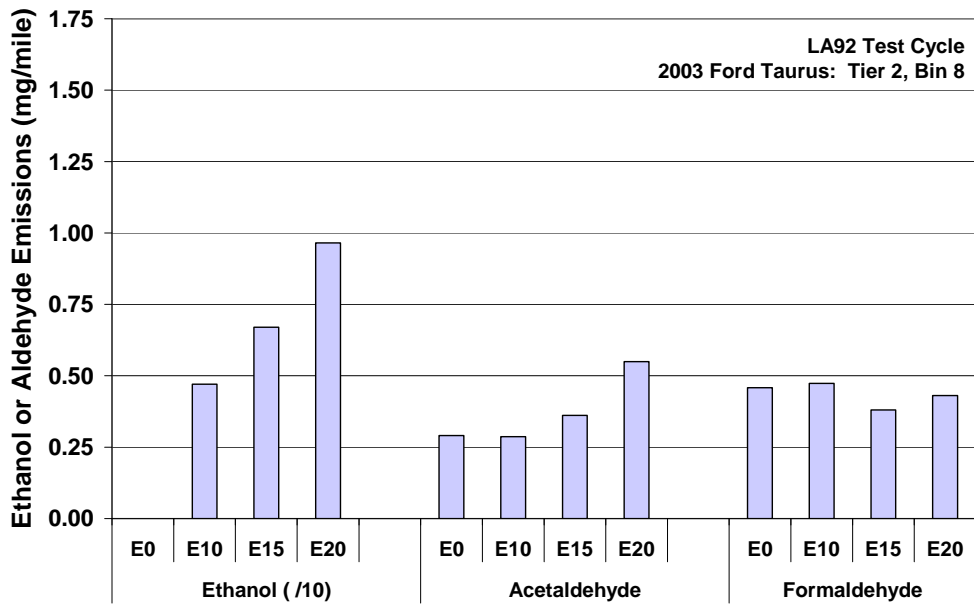
Fig. C.8. Ethanol, acetaldehyde, and formaldehyde emissions for 2003 Ford Taurus on LA92 cycle. Bars show average of 3 tests at 75°F.
