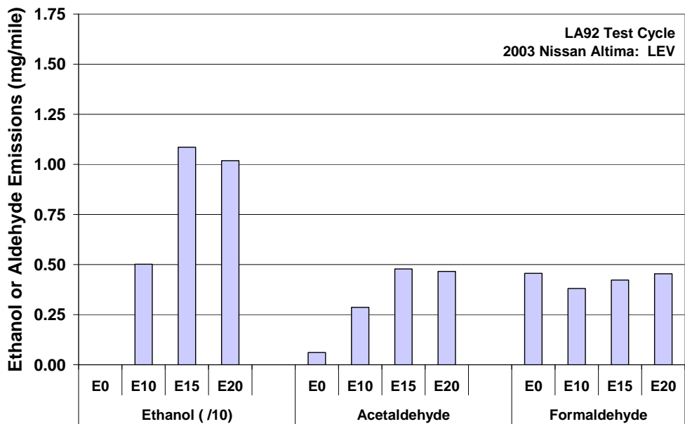
Fig. C.18. Ethanol, acetaldehyde, and formaldehyde emissions for 2003 Nissan Altima on LA92 cycle. Bars show average of 3 tests at 75°F.
