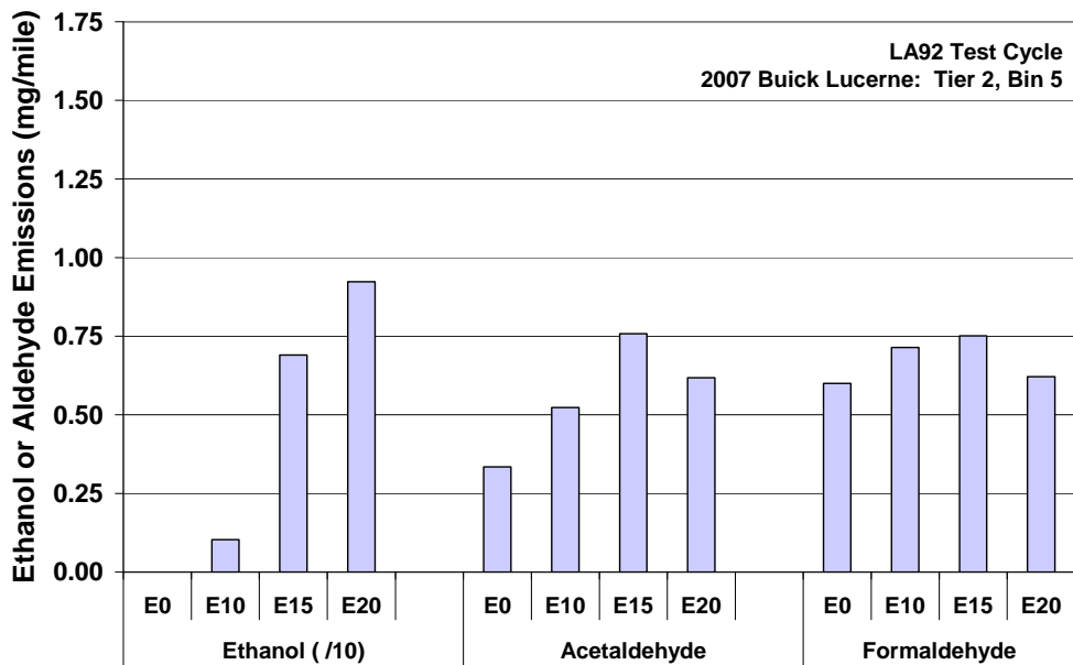
Fig. C.10. Ethanol, acetaldehyde, and formaldehyde emissions for 2007 Buick Lucerne on LA92 cycle. Bars show average of 3 tests at 75°F.
