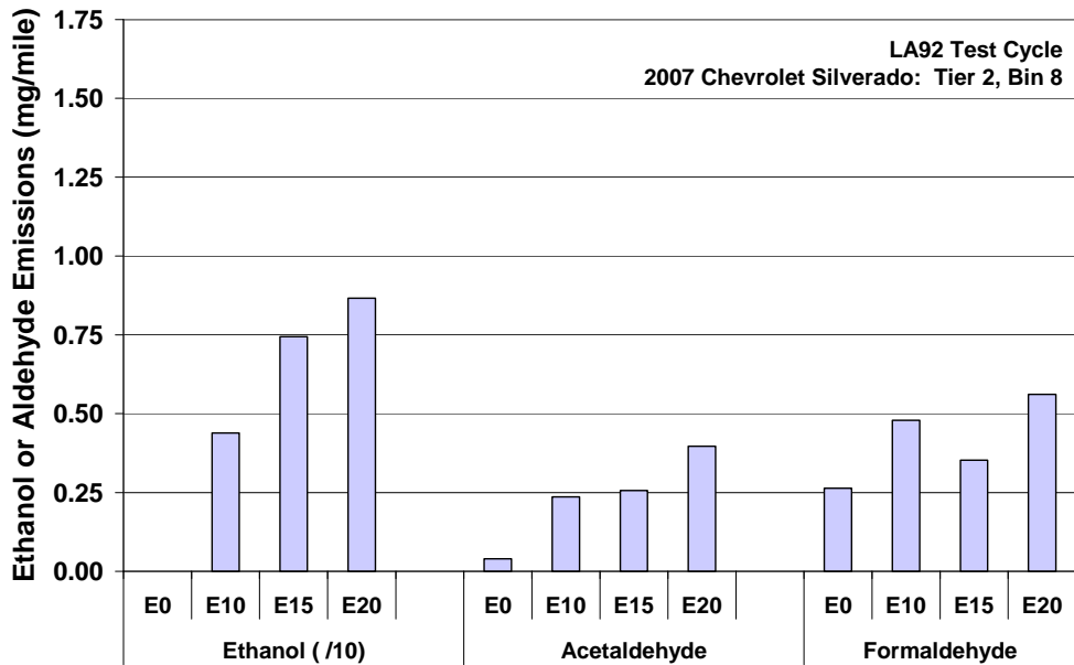
Fig. C.14. Ethanol, acetaldehyde, and formaldehyde emissions for 2007 Chevrolet Silverado on LA92 cycle. Bars show average of 3 tests at 75°F.
