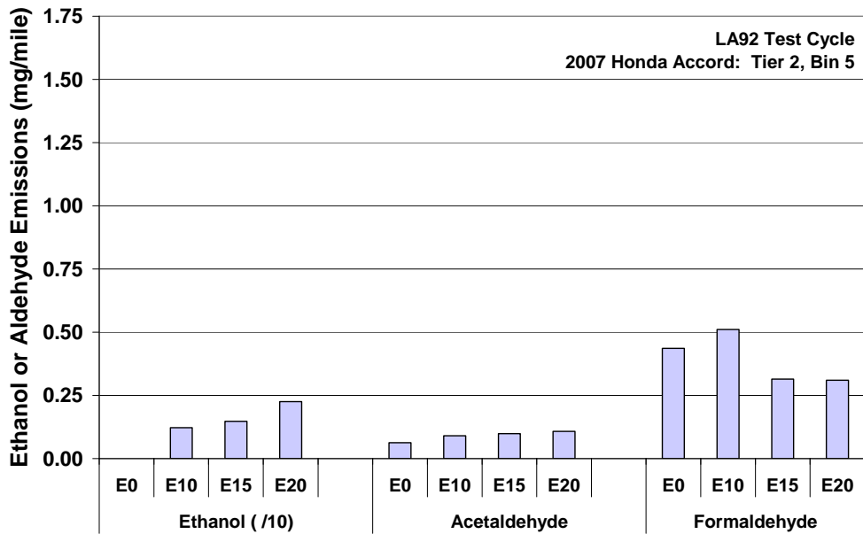
Fig. C.16. Ethanol, acetaldehyde, and formaldehyde emissions for 2007 Honda Accord on LA92 cycle. Bars show average of 3 tests at 75°F.
