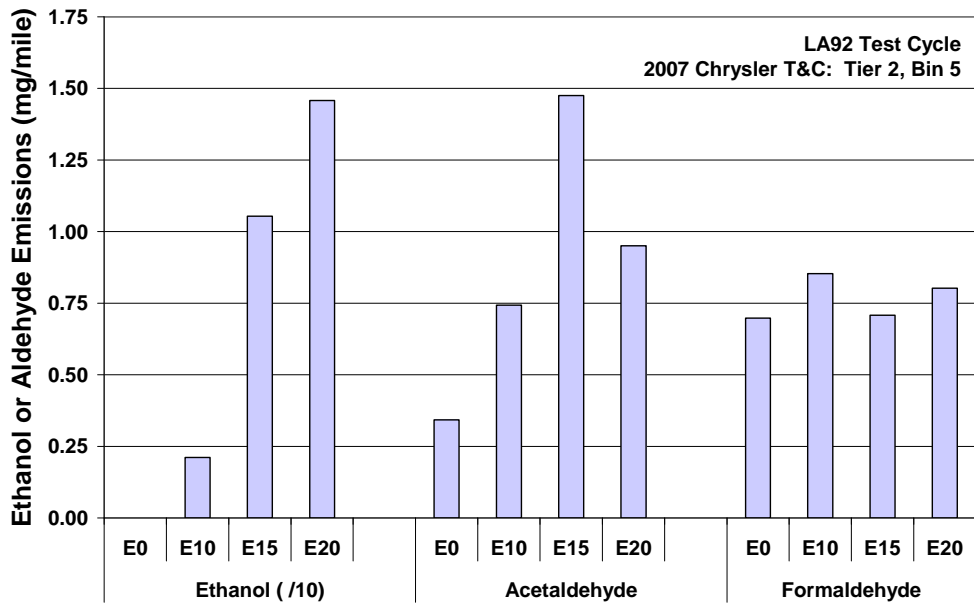
Fig. C.2. Ethanol, acetaldehyde, and formaldehyde emissions for 2007 Chrysler Town and Country on LA92 cycle. Bars show average of 3 tests at 75°F.
