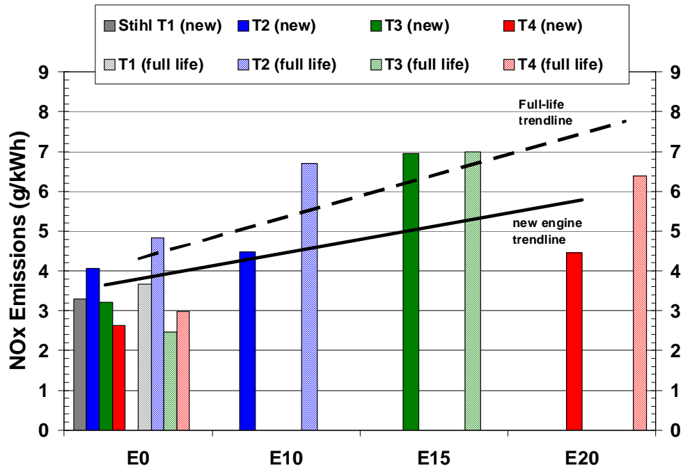
Fig. D.18. Nitrogen oxide (NO x ) emissions for Class IV Stihl line trimmer engines at new and full-useful-life (full-life) condition. Solid colors represent tests in the new condition while striped bars of the same color represent the same engine at the full-life condition.
