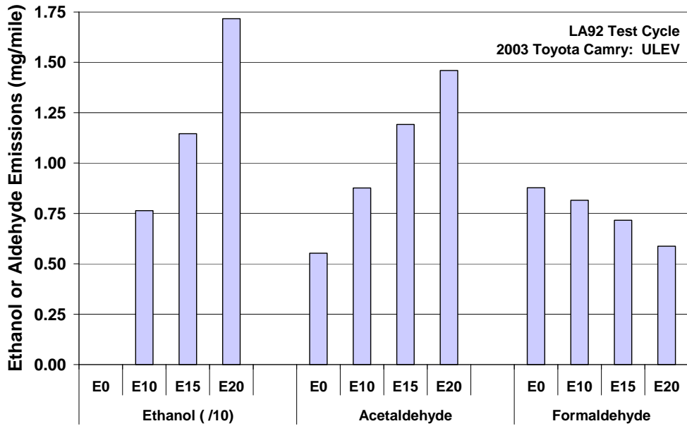
Fig. C.22. Ethanol, acetaldehyde, and formaldehyde emissions for 2003 Toyota Camry on LA92 cycle. Bars show average of 3 tests at 75°F.
