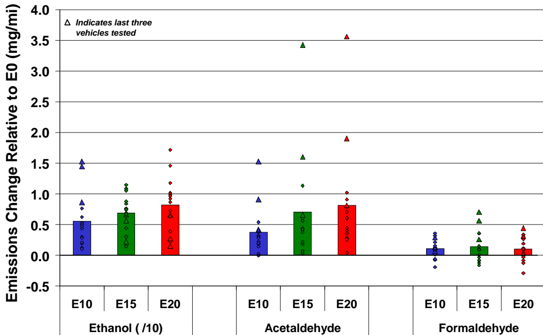
Fig. 3.2. Average change in ethanol and aldehyde emissions for all vehicles compared to E0 fuel on the LA92 cycle. Bars show average for all vehicles, while discrete data points show the change for each vehicle tested.
