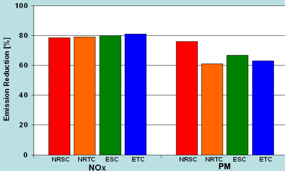
SCRi system performance during steady state and transient test cycles
