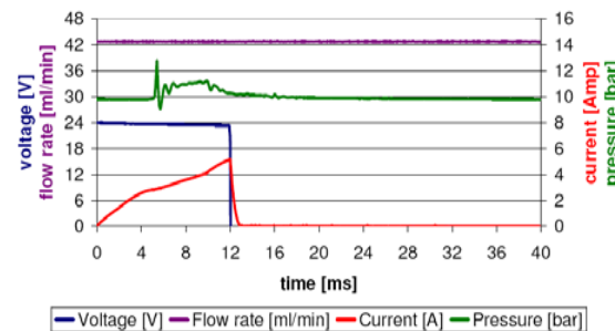
Signal chart of one pump stroke pump frequency: 25 Hz; switching on-time: 12ms
