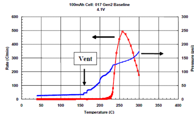
ARC chamber pressure evolution C. Orendorff, SNL
