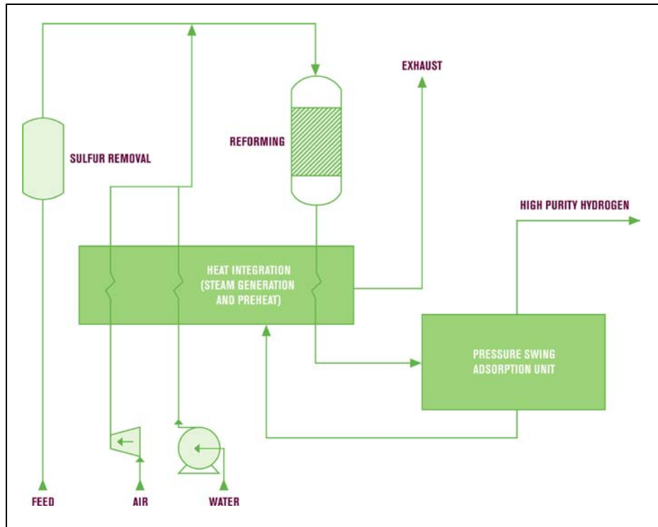
Figure C-5. HyRadix hydrogen production process (Courtesy of HyRadix)
