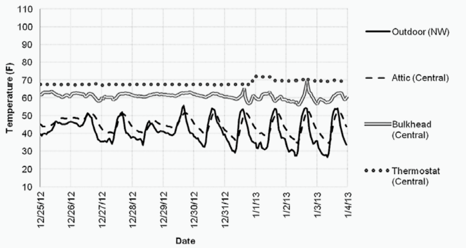
Bulkhead temperatures relative to indoor and outdoor temperatures in the heating season
