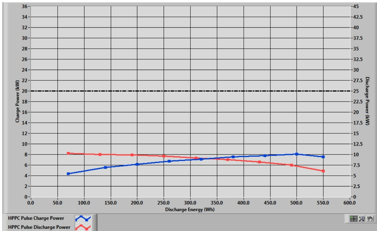
Figure 6: Peak Power Values with DOE Performance Goals
