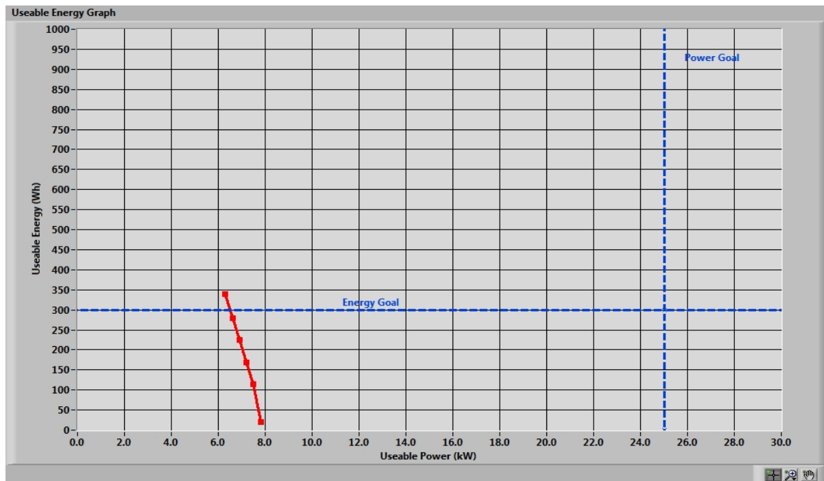
Figure 7: Useable Energy
