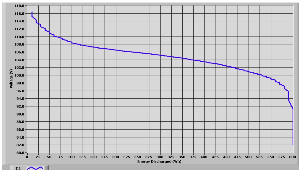
Figure 1: Voltage vs. Energy Discharged
