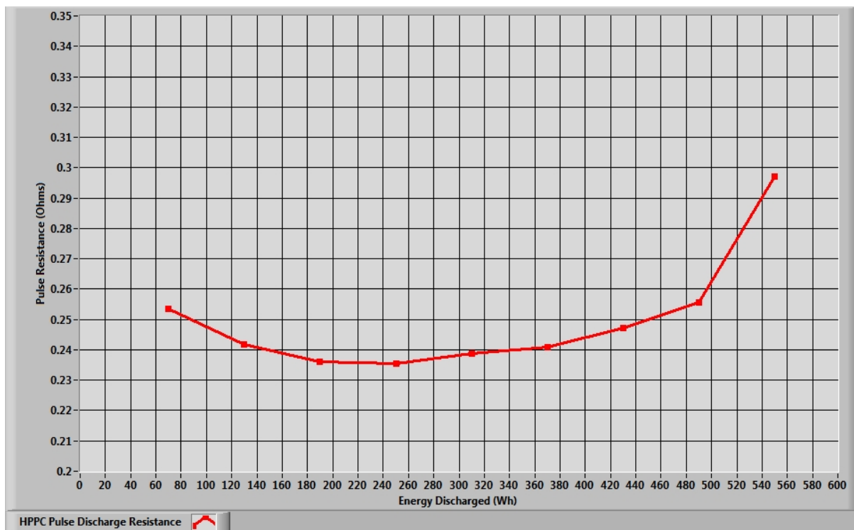
Figure 3: Discharge Pulse Resistance vs. Energy Discharged
