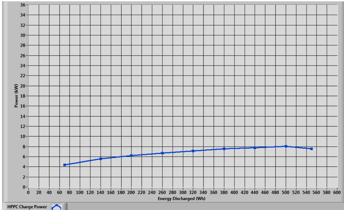
Figure 4: Charge Pulse Power vs. Energy Discharged
