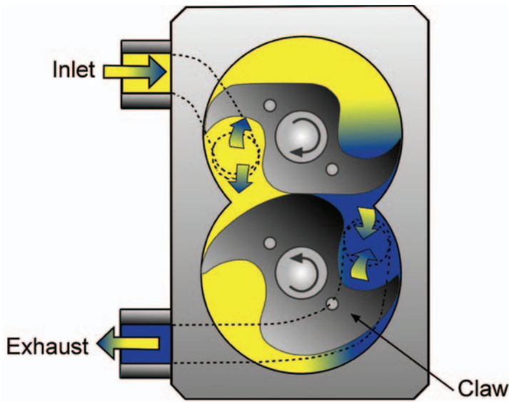
Figure 3. Typical claw technology
