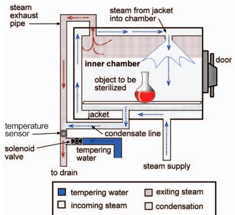
Figure 4. Typical steam sterilizer
