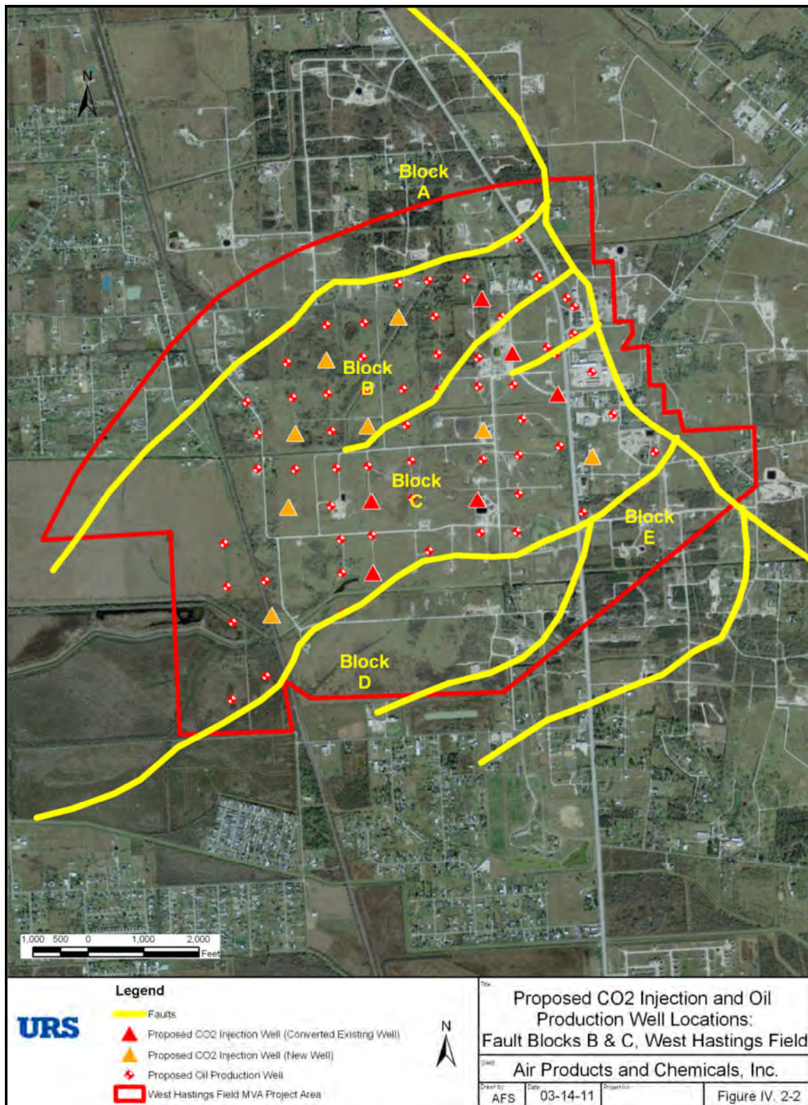
Figure 4: General Location of APCI / Denbury Project Activities within West Hastings Field, Brazoria County (Aerial)
