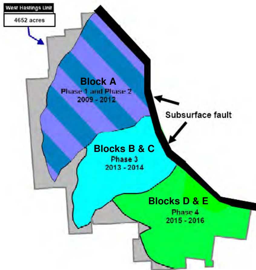
Figure IV.2-1. Proposed Phased Implementation Schedule for CO 2 Injection into the West Hastings Field.
