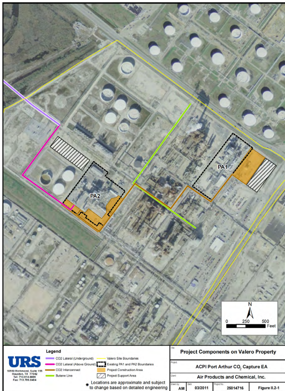
Figure II.2-1. Approximate Locations of Project Components on Valero Refinery Property
