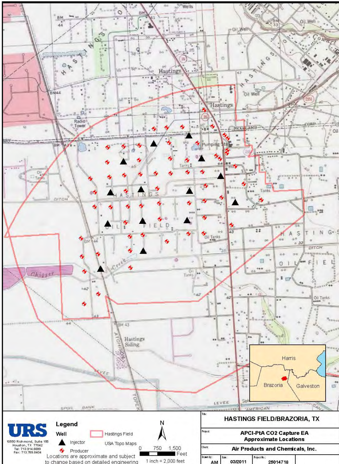
Figure 4: Overview of West Hastings Field, Brazoria County
