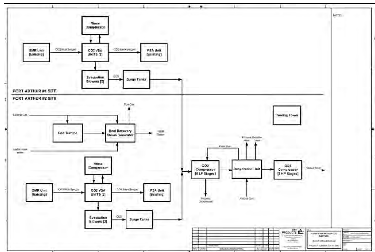
Figure II.2-2. Conceptual Process Flow Diagram for the CO 2 Capture Process
