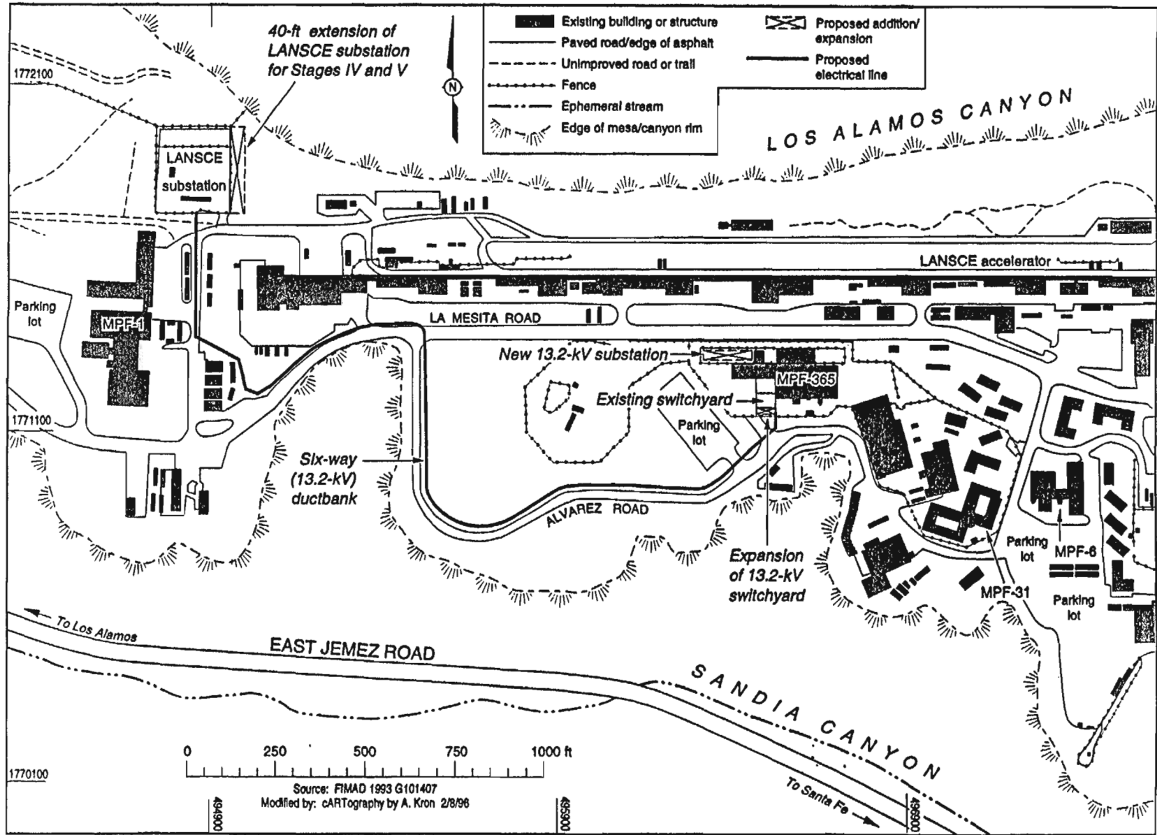
Figure 6B. Additions to electrical distribution system required for LEDA, Option 2.
