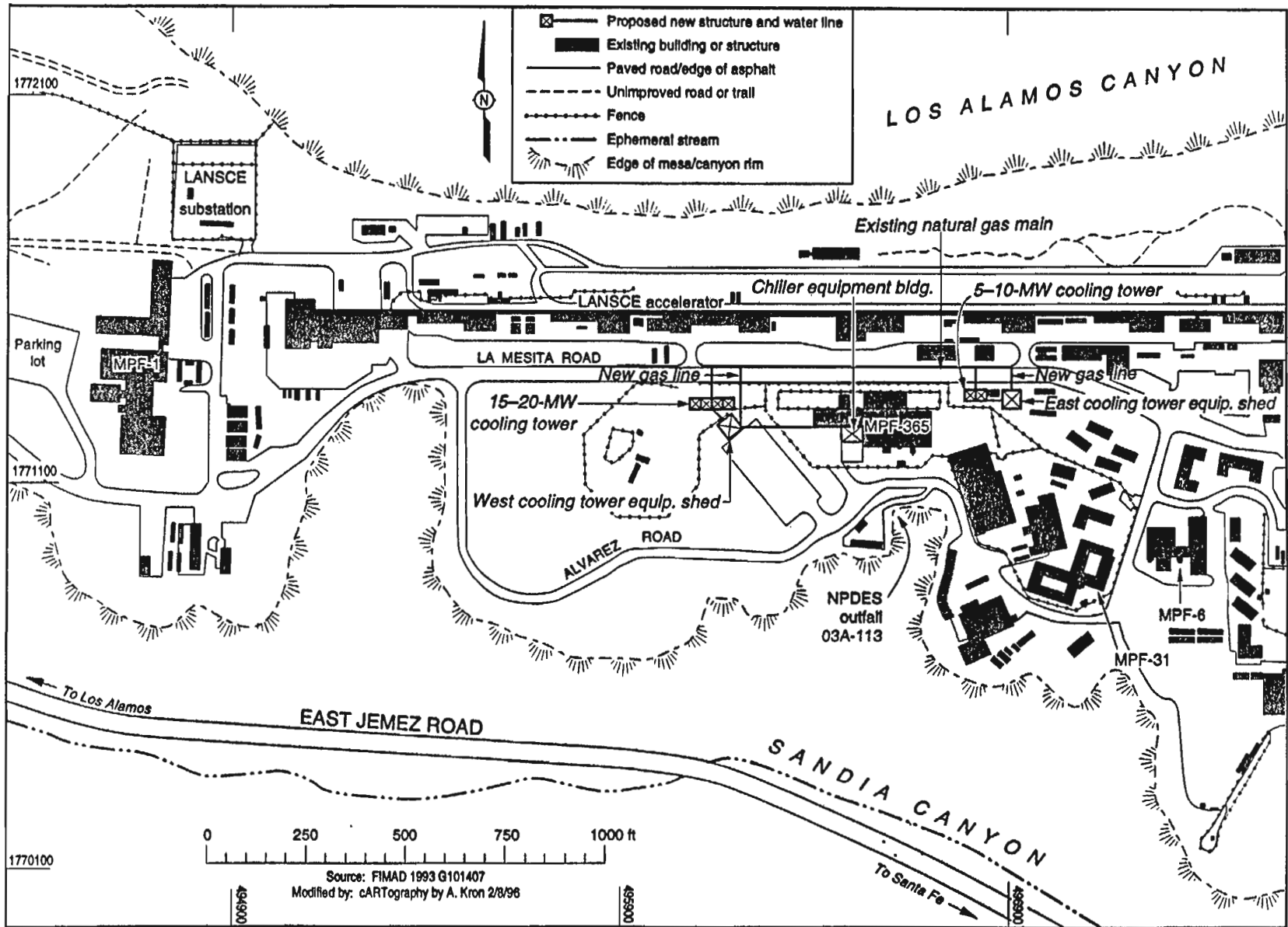
Figure 7. Additions to water distribution system required for LEDA.
