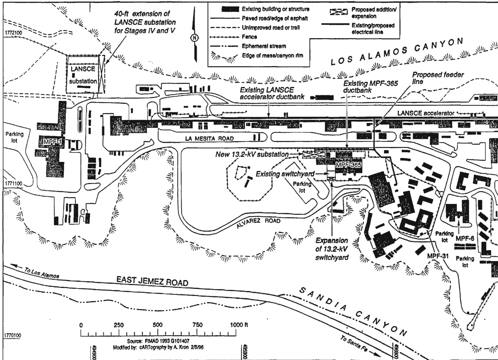
Figure 6A. Additions to electrical distribution system required for LEDA, Option 1.
