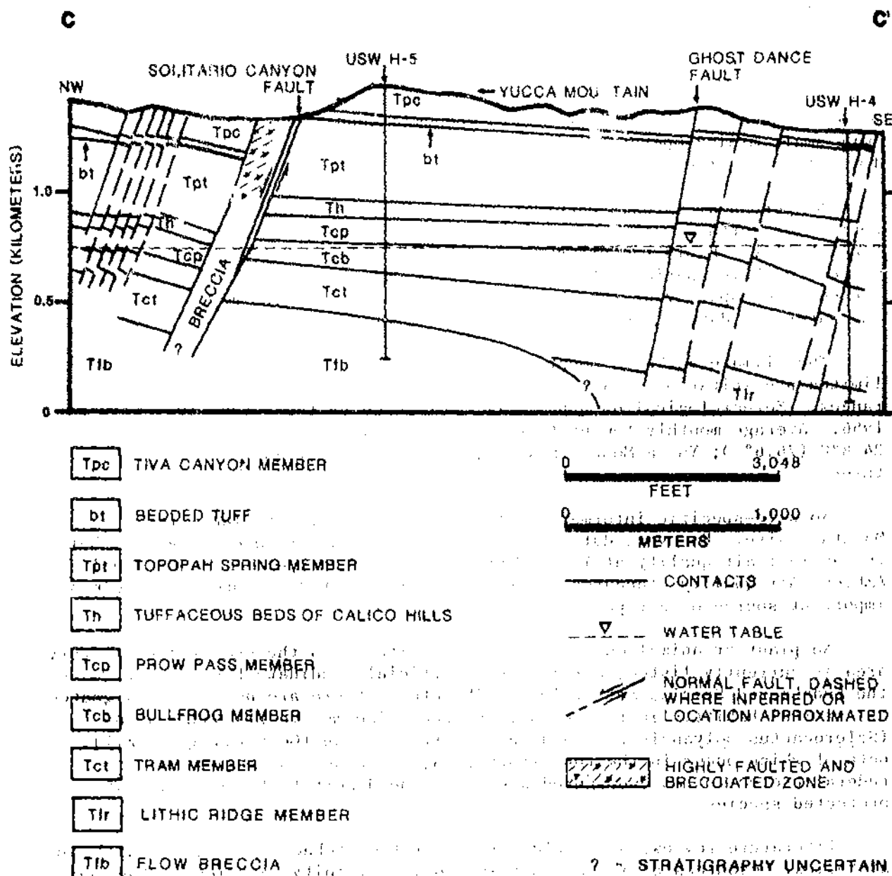
Figure 3. Geologic cross section of the Yucca Mountain site.
