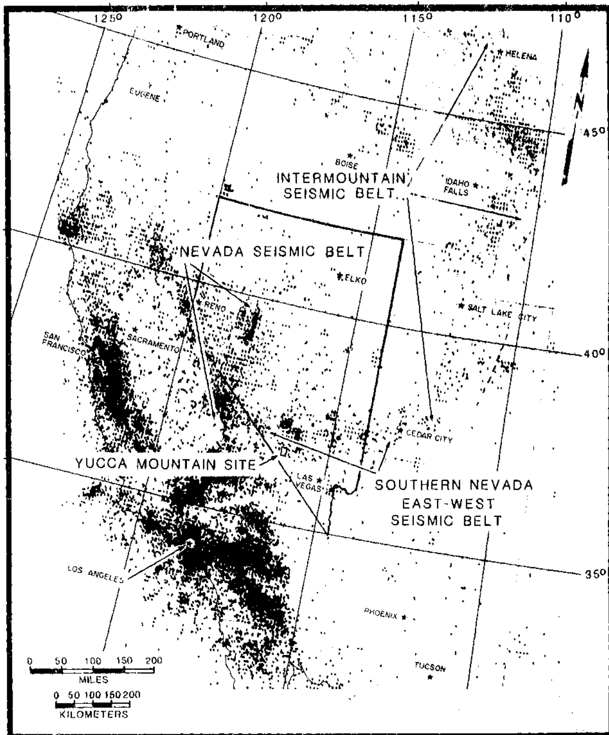
Figure 3-9. Historical seismicity in the western United States showing the Nevada Seismic Belt, the Intermountain Seismic Belt, and the southern Nevada East-West Seismic Belt. It should be noted that some of the seismicity in the western end of the East-West Seismic Belt represents underground explosions at the Nevada Test Site. For California, the minimum-magnitude earthquakes plotted where Richter M \sim 1 and for the rest of the western United States, they were Richter M \sim 3 . Modified from Smith (1978).
