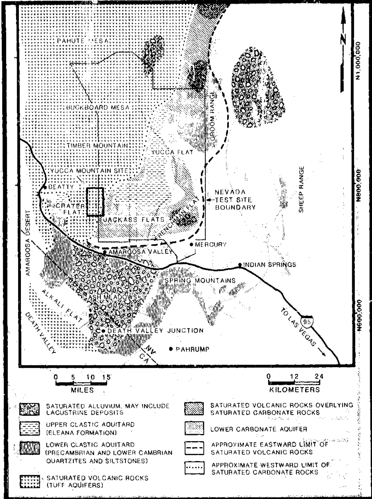
Figure 2-6. General distribution of the major aquifers and aquitards in the southern Great Basin near Yucca Mountain. Compiled from Waddell et al. (1984).
