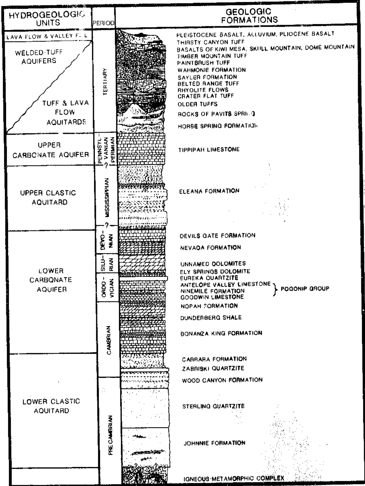
Figure 2-4. General relationships among hydrogeologic units and geologic formations in the southern Great Basin. The question marks refer to an uncertain boundary. Modified from Sinnock (1982).
